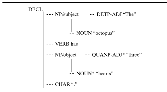
SYNTACTIC PARSE TREE
