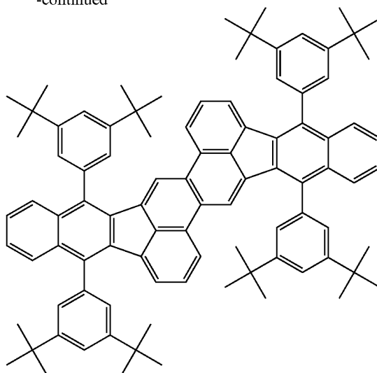
Exemplified Compound H-6
