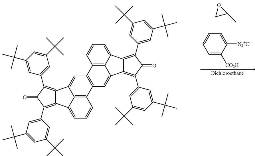
Compound 1-8
