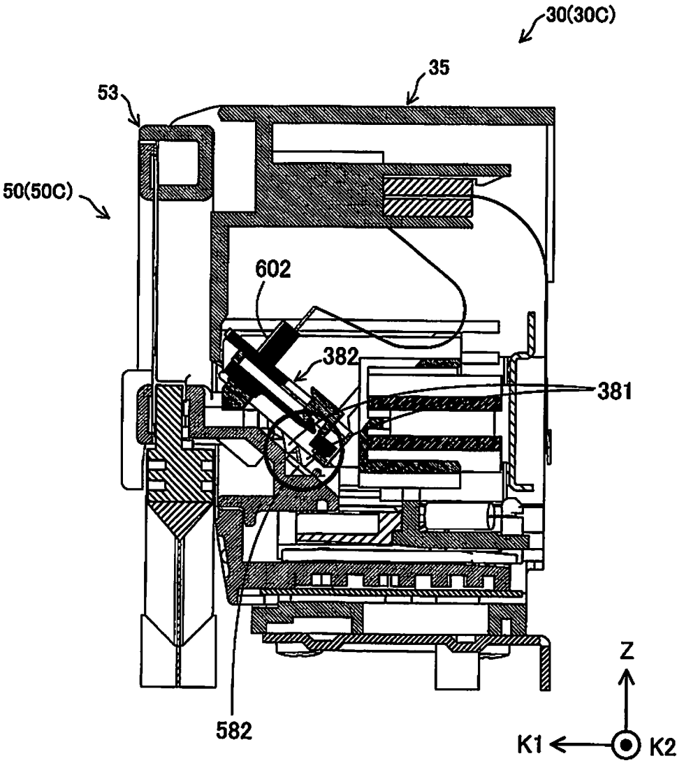
F25B-F25B PARTIAL SECTIONAL VIEW
