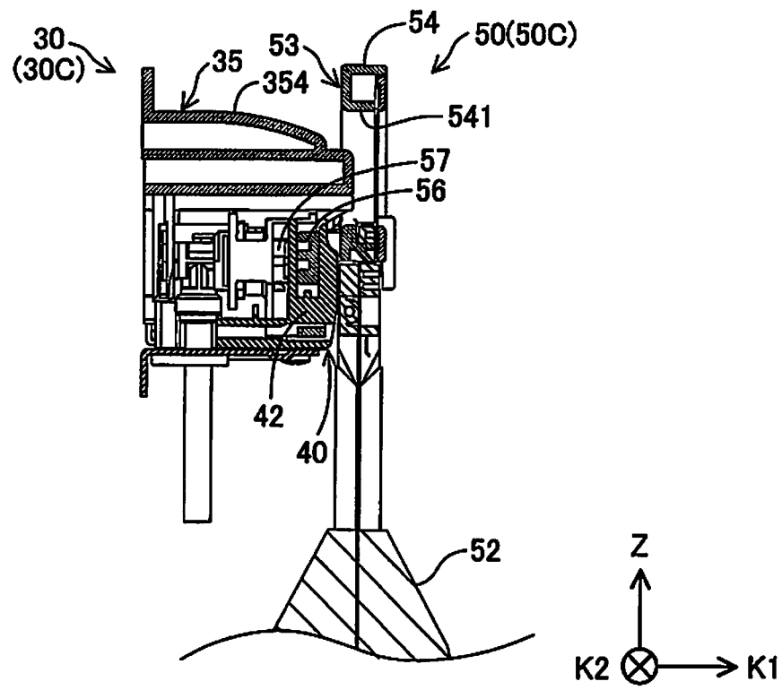
F20-F20 PARTIAL SECTIONAL VIEW
