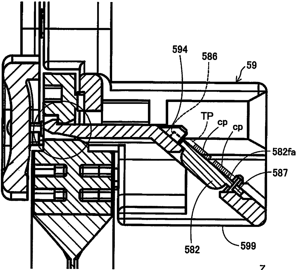
F13a-F13a PARTIAL SECTIONAL VIEW
