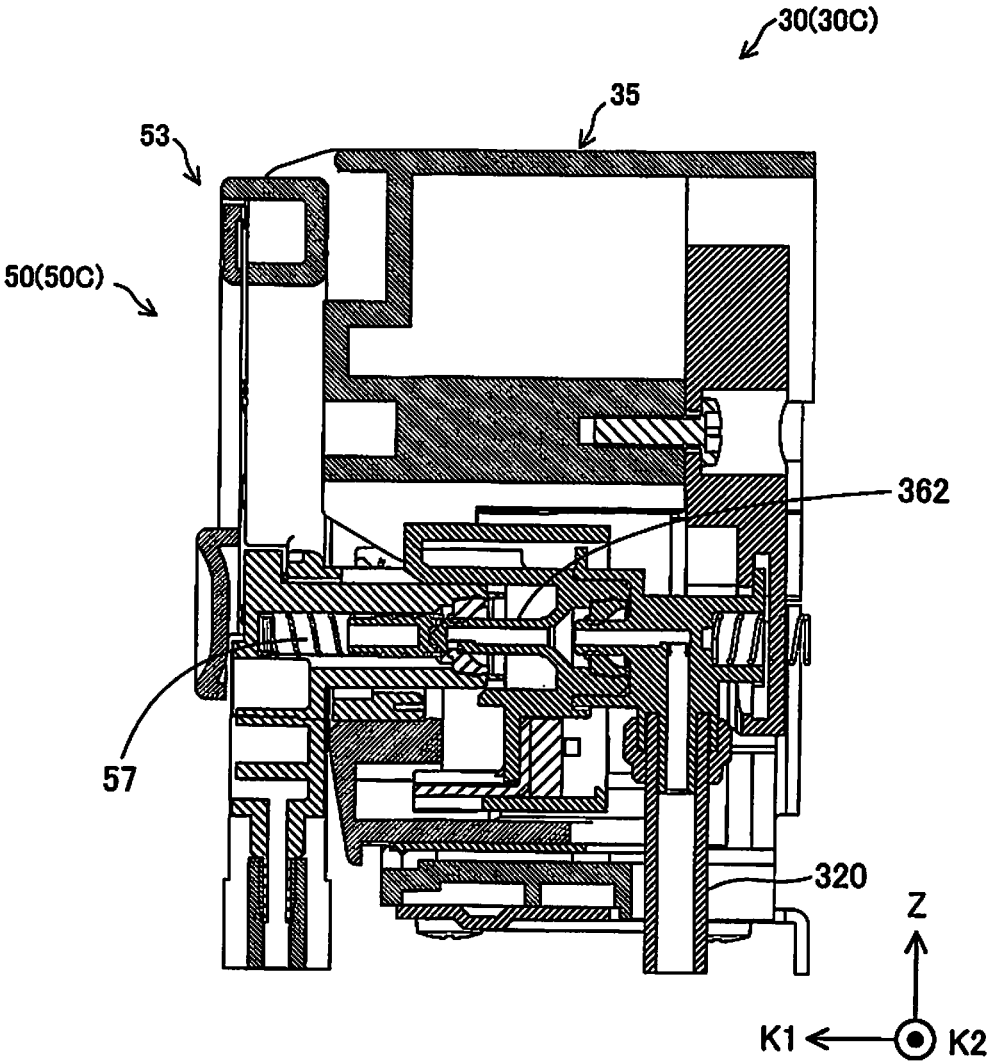
F25A-F25A PARTIAL SECTIONAL VIEW
