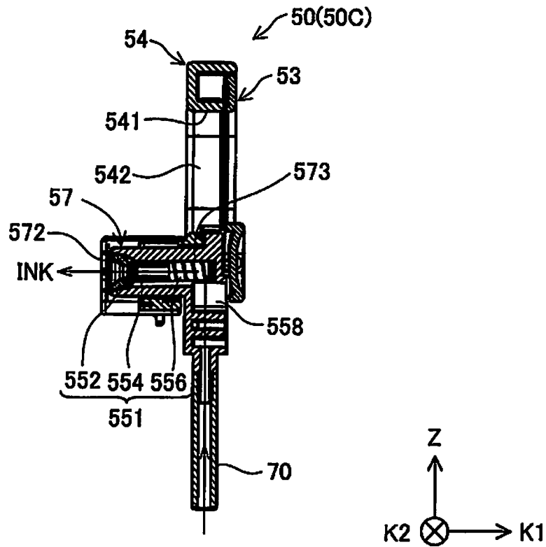
F13-F13 SECTIONAL VIEW
