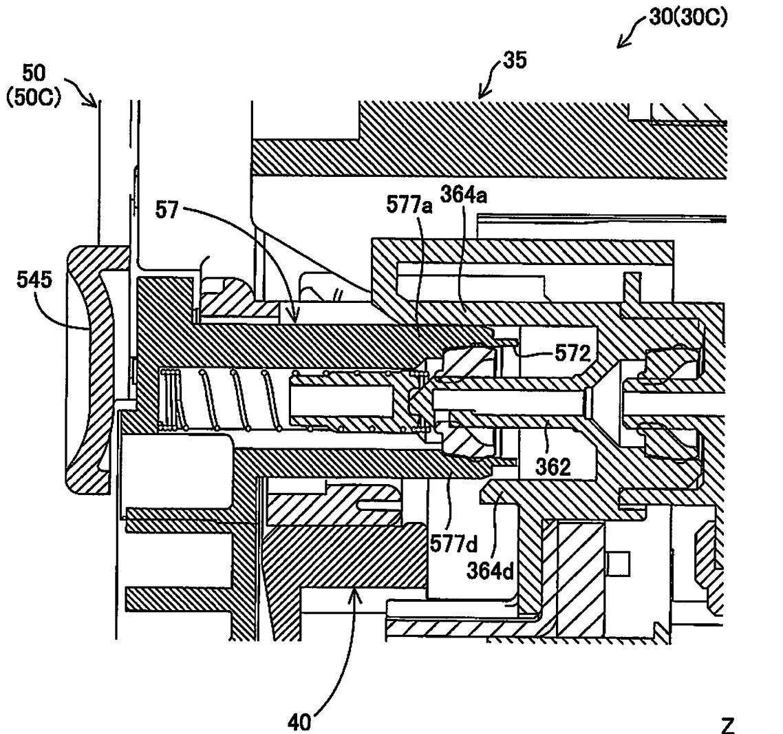
F25A-F25A PARTIAL SECTIONAL VIEW
