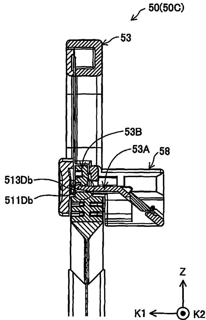
F17Da-F17Da PARTIAL SECTIONAL VIEW
