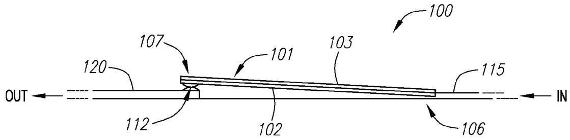
FIG. 1 (PRIOR ART)
