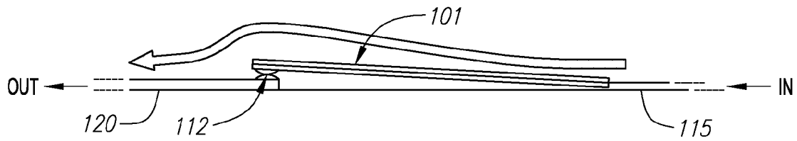
FIG. 2-1 (PRIOR ART)
