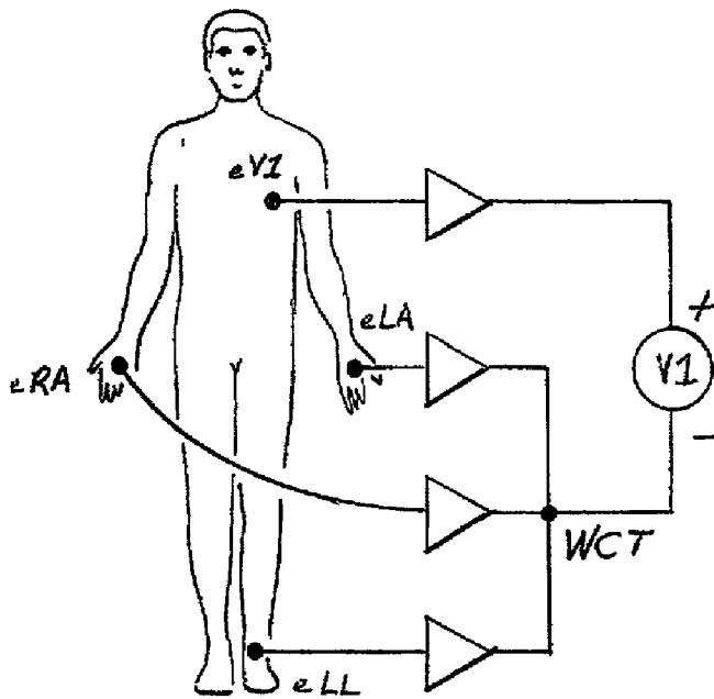
Fig. 3 PRIOR ART
