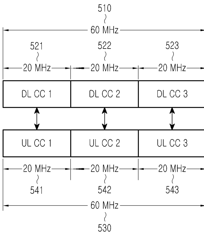
FIG.5 (PRIOR ART)
