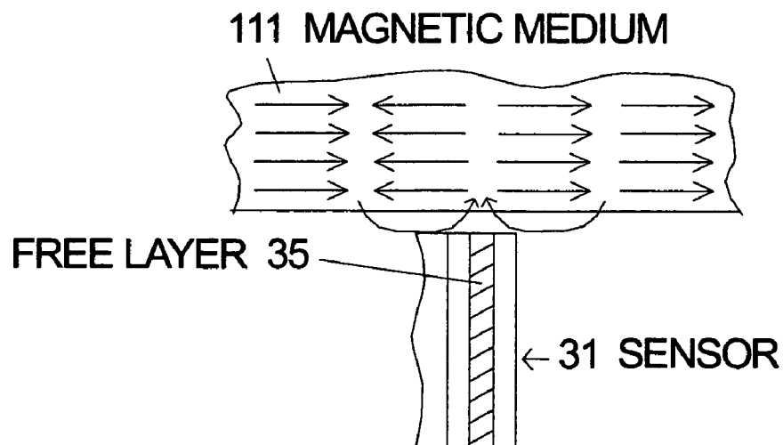
Fig. 12 PRIOR ART
