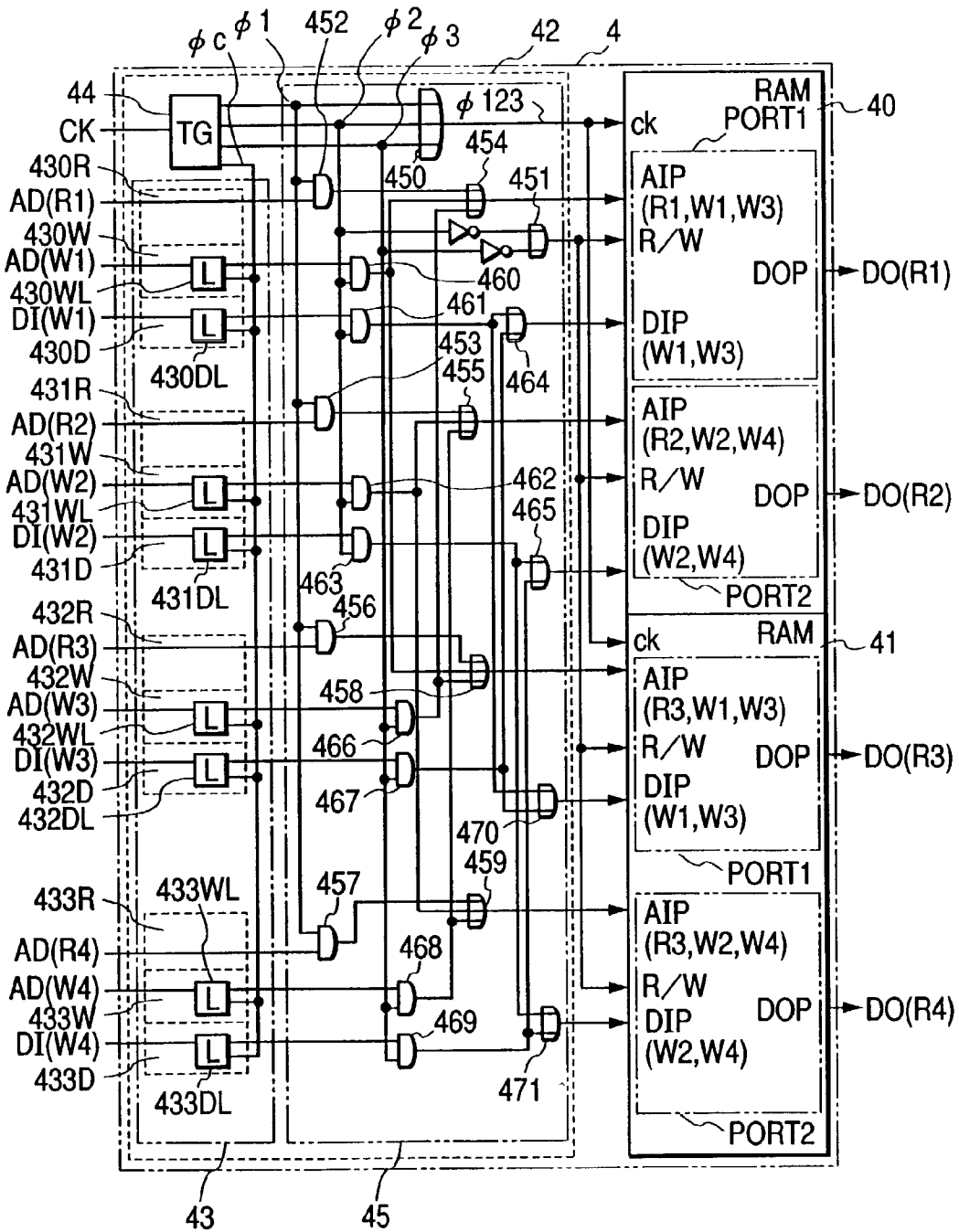
8 PORT RAM (USING TWO 2-PORT RAMS)
