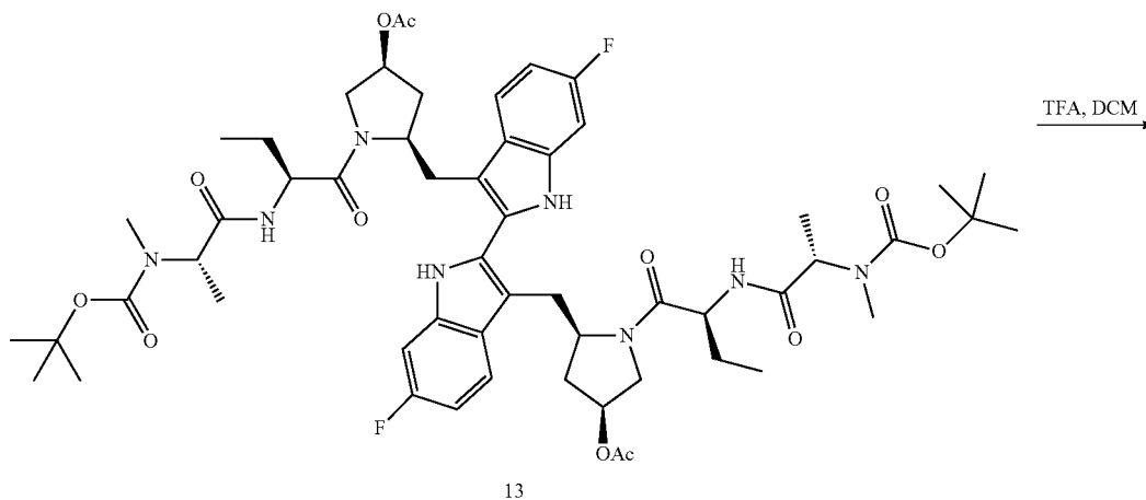
Scheme XIII
