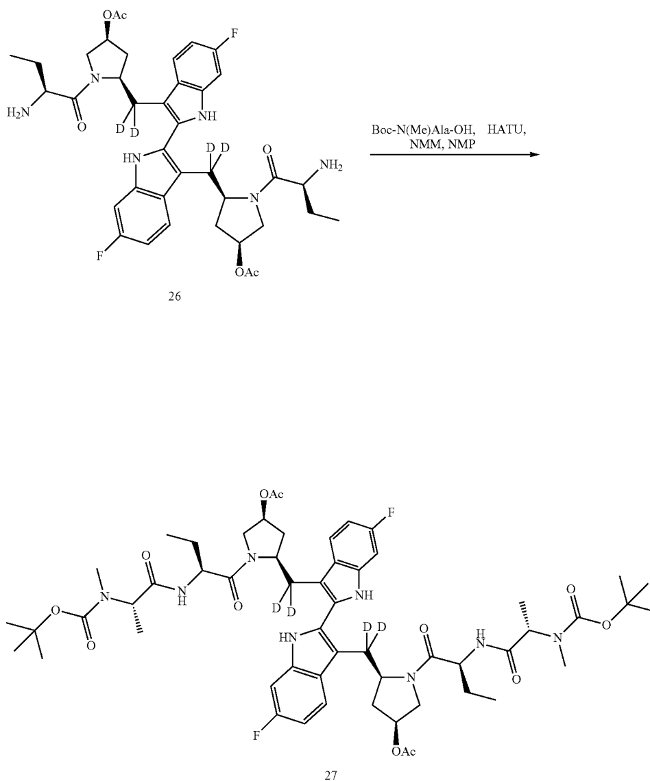
Scheme XXV
