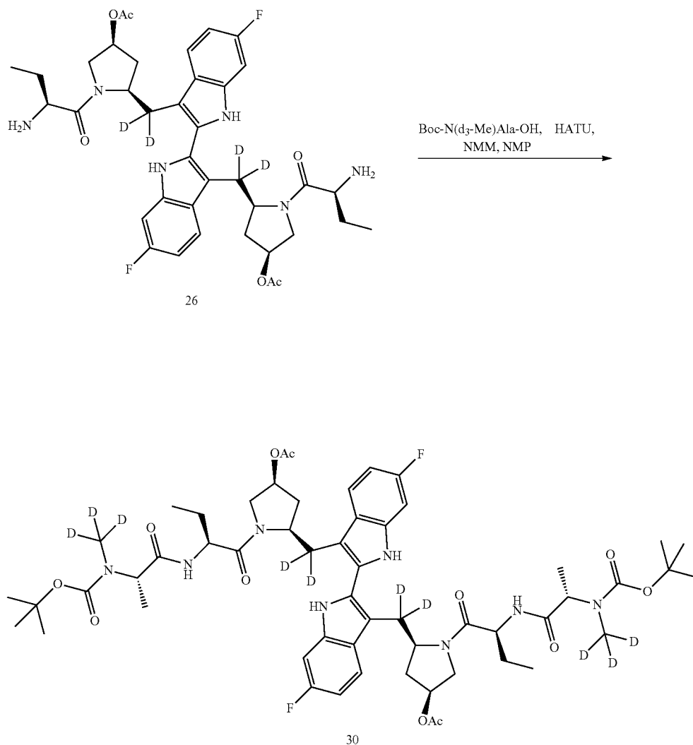
Scheme XXVIII
