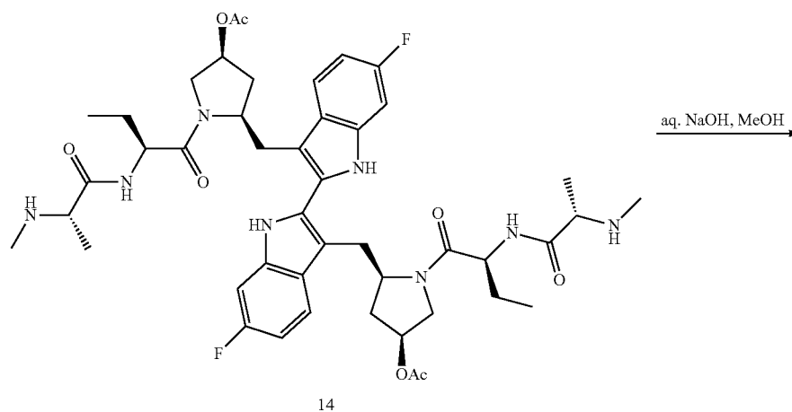
Scheme XIV
