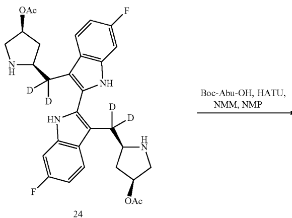
Scheme XXIII
