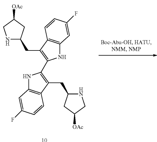
Scheme X
