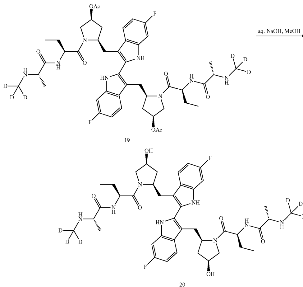
Scheme XVIII
