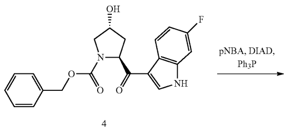
Scheme IV
