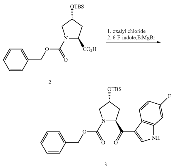
Scheme II
