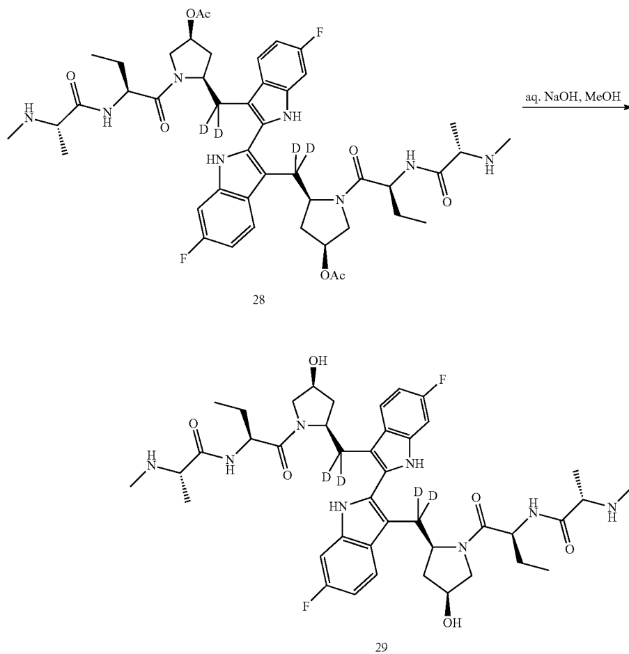
Scheme XXVII
