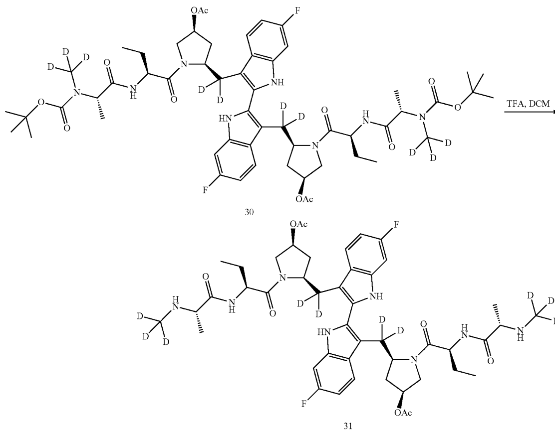
Scheme XXIX
