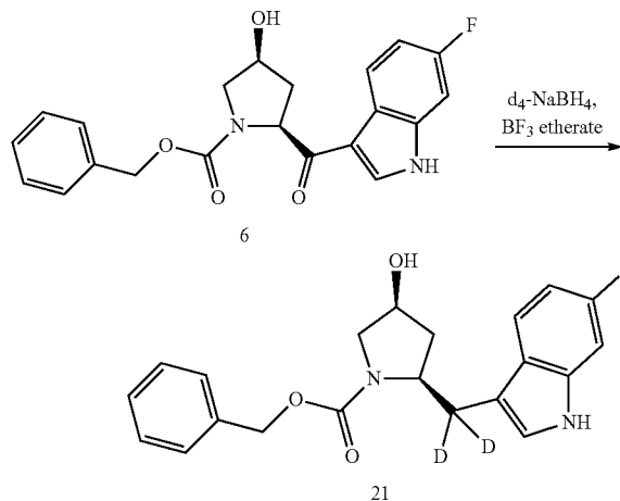
Scheme XIX
