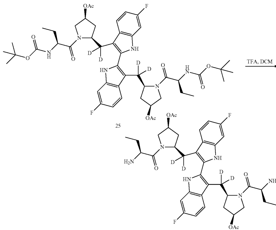
Scheme XXIV
