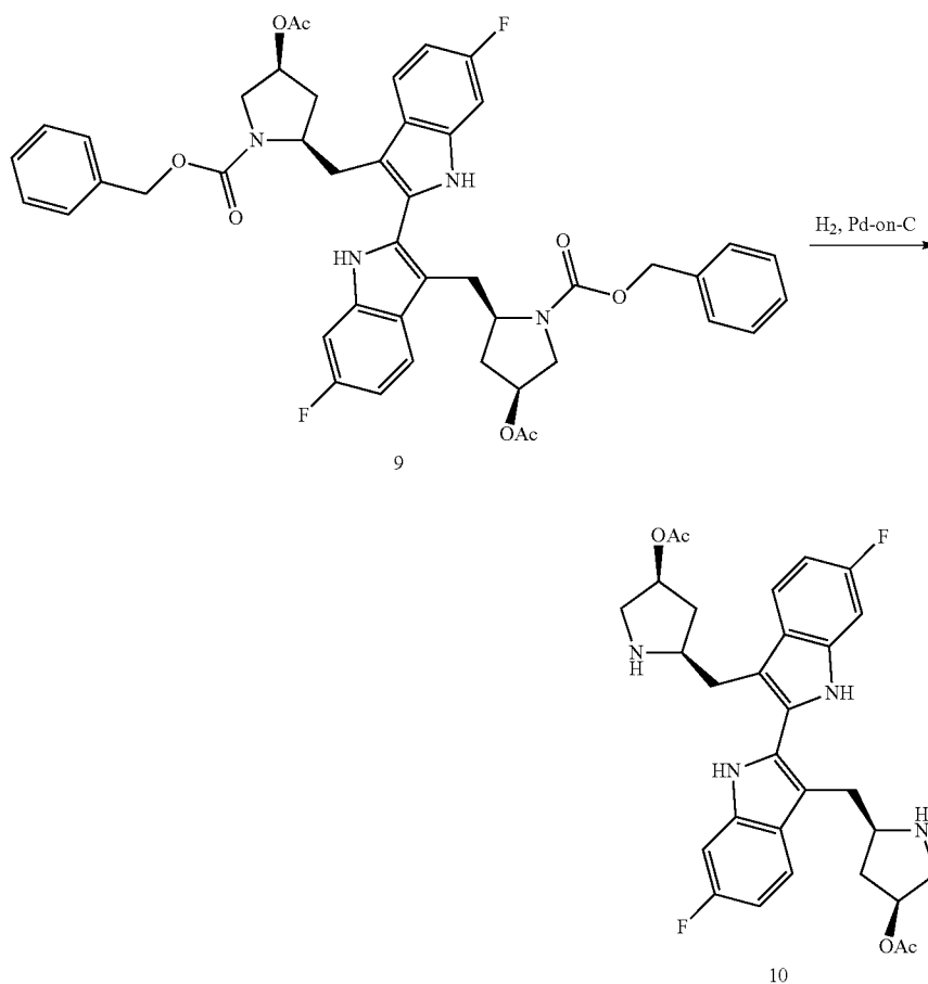
Scheme IX
