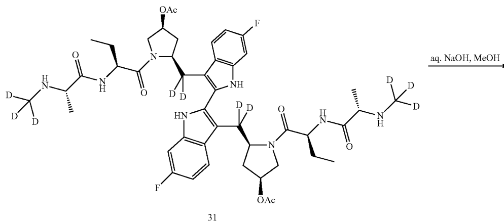
Scheme XXX
