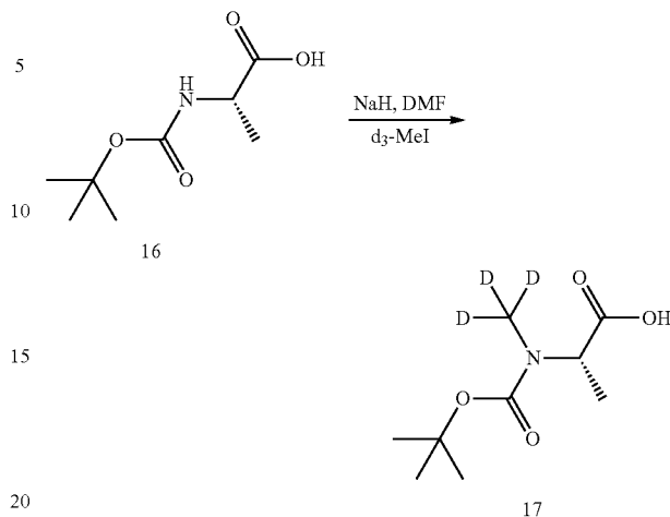
Scheme XV
