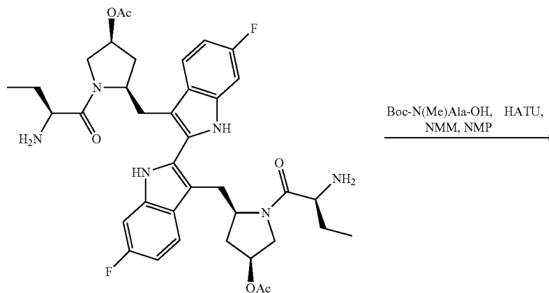
Scheme XVI
