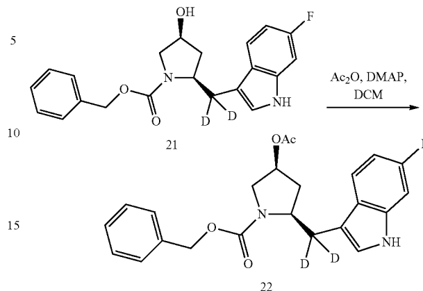
Scheme XX
