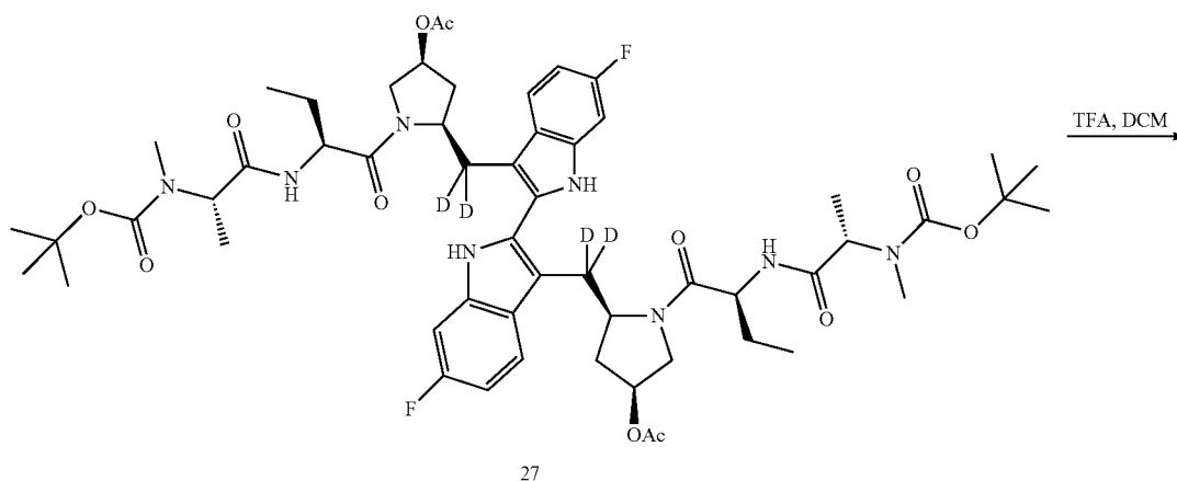
Scheme XXVI
