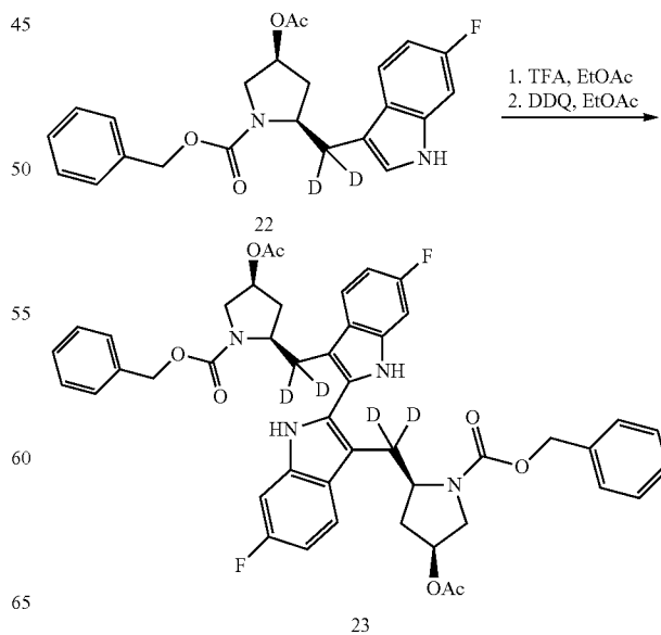
Scheme XXI
