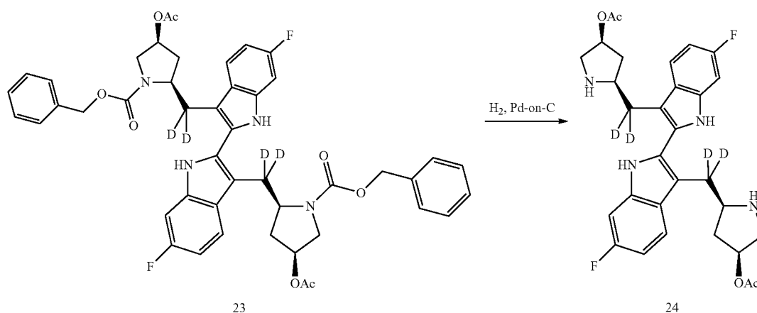
Scheme XXII
