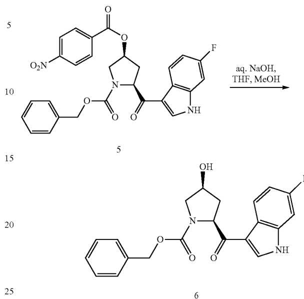
Scheme V
