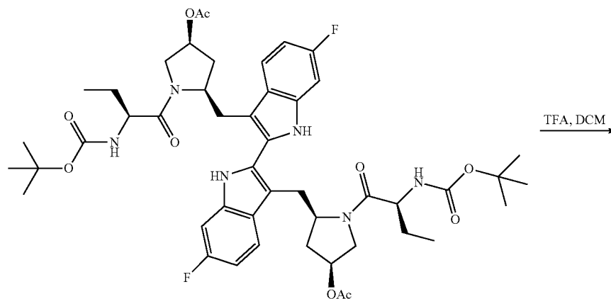
Scheme XI
