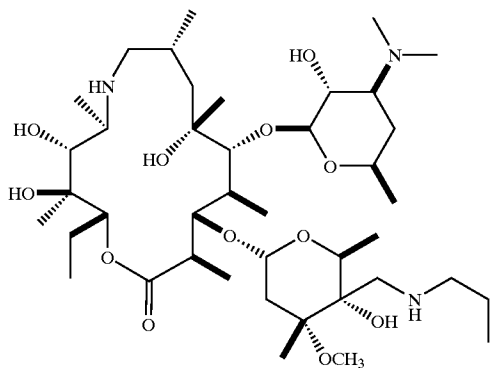
Isomer I
