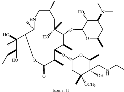
Isomer II
