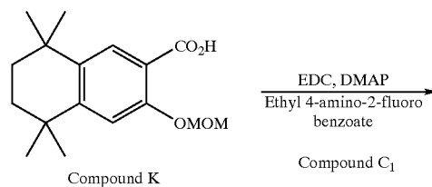
Reaction Scheme 8
