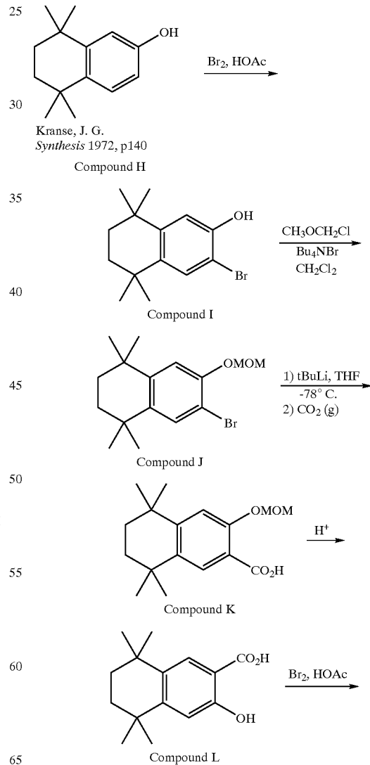
Reaction Scheme 2
