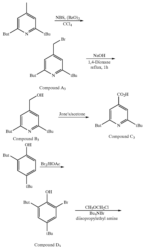
Reaction Scheme 13
