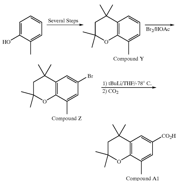
Reaction Scheme 4
