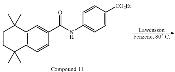
Reaction Scheme 7
