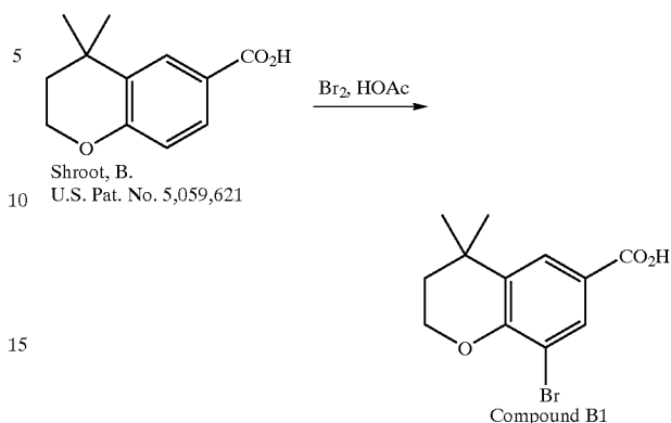
Reaction Scheme 5
