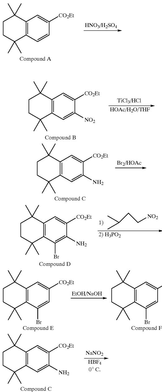
Reaction Scheme 1
