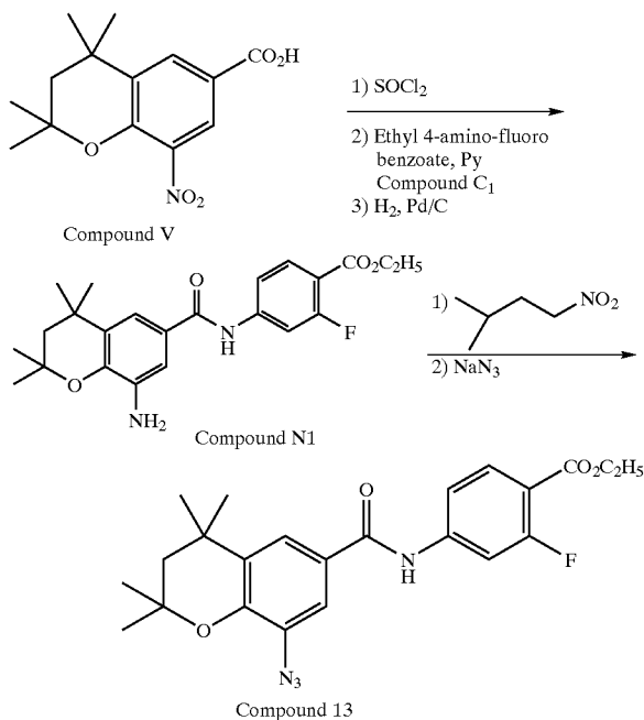
Reaction Scheme 10
