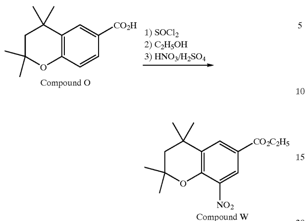
Reaction Scheme 3
