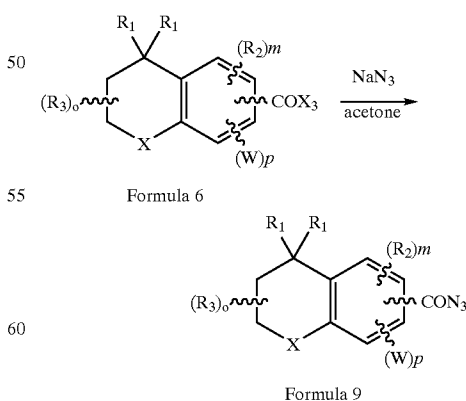
Reaction Scheme 11
