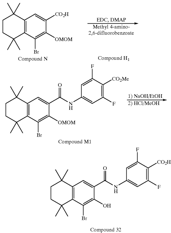
Reaction Scheme 9
