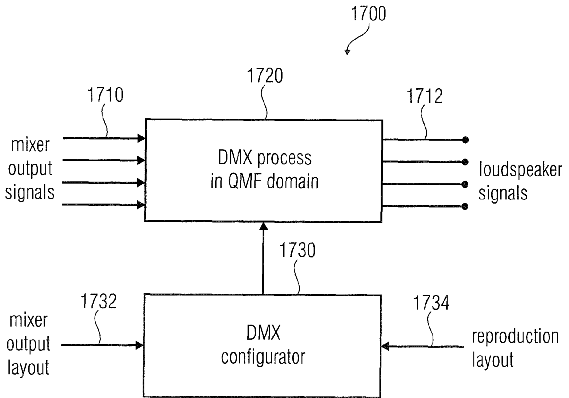
STRUCTURE OF FORMAT CONVERTER FIG 17
