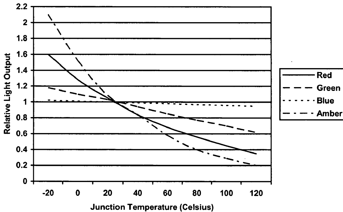
Figure 3 (Prior Art)
