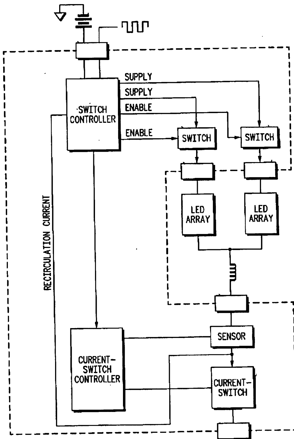
Figure 2 (Prior Art)
