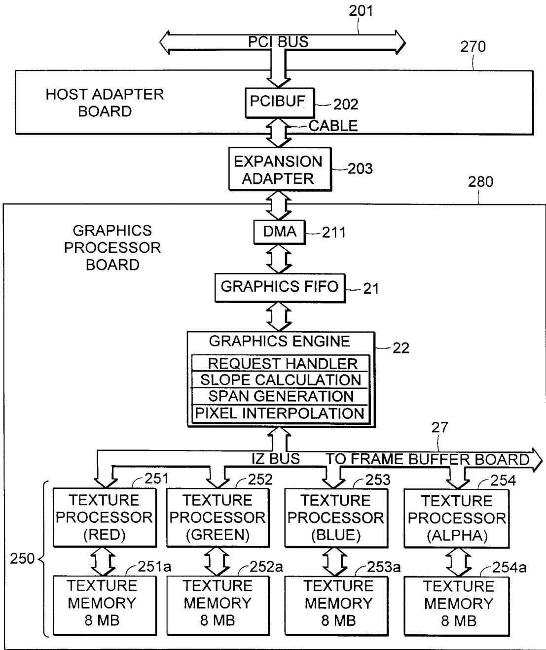
GLI BLOCK DIAGRAM
