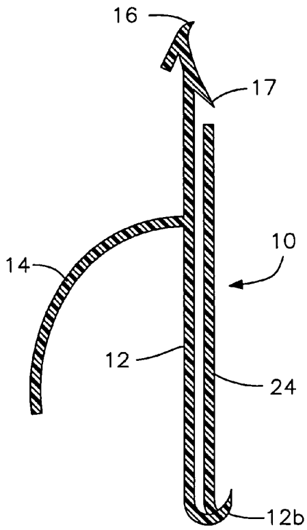
FIG. 1 (PRIOR ART)
