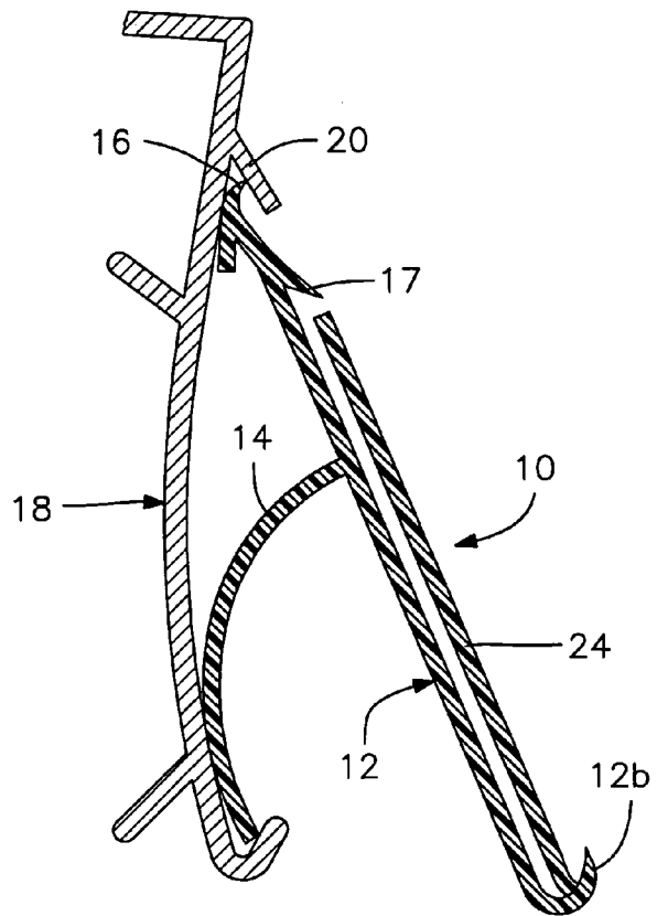
FIG. 2 (PRIOR ART)
