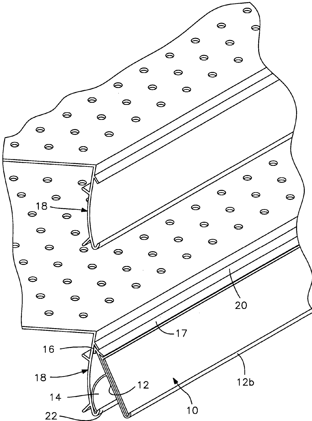
FIG. 3 (PRIOR ART)
