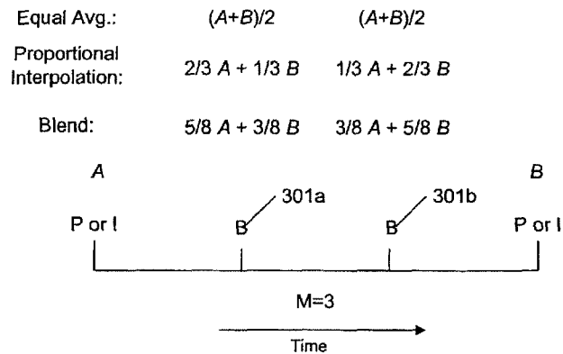
FIG. 3 Blended Pixel Value Weighting
