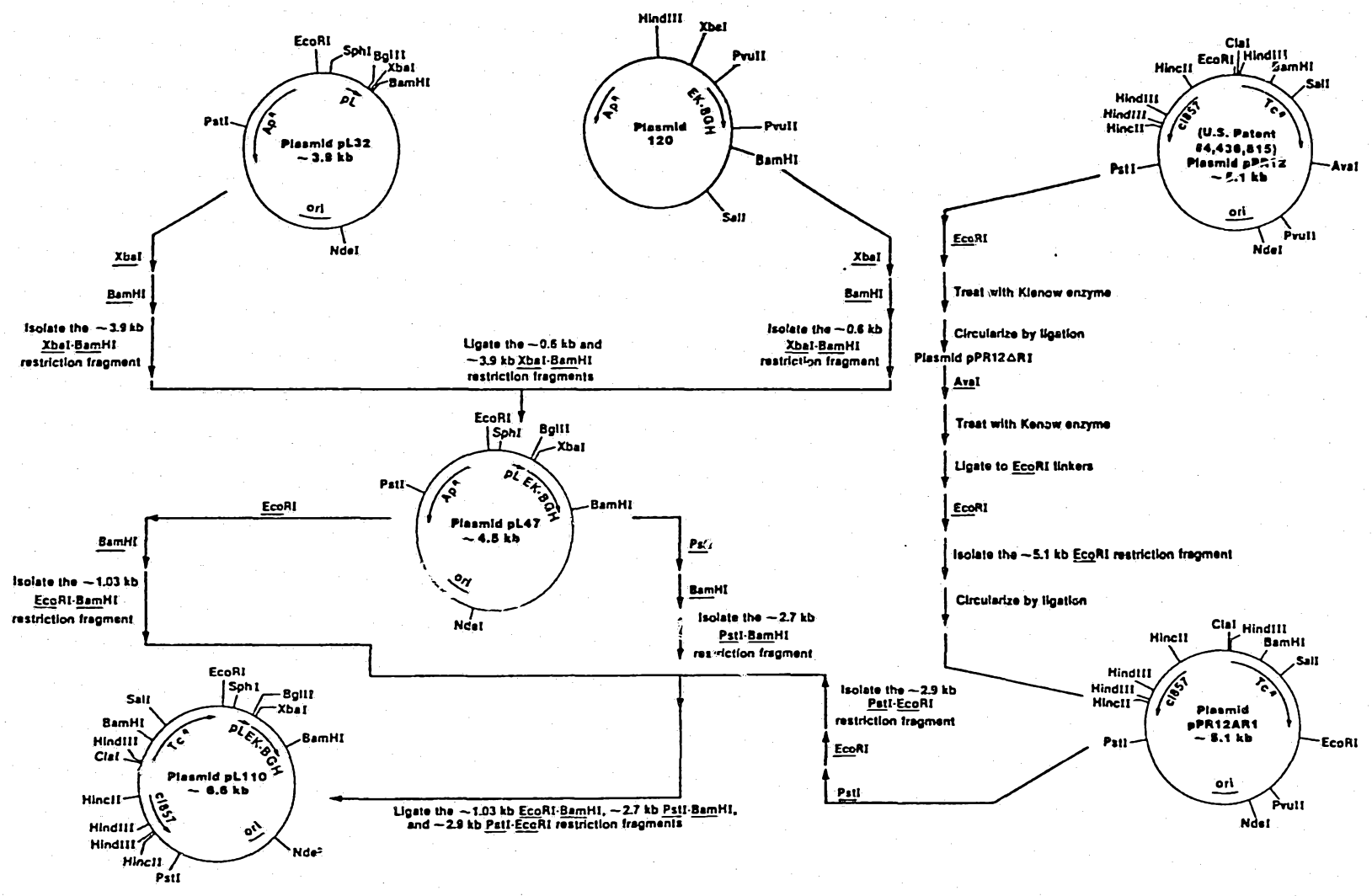
FIG. 4 Construction of Plasmid pL110
