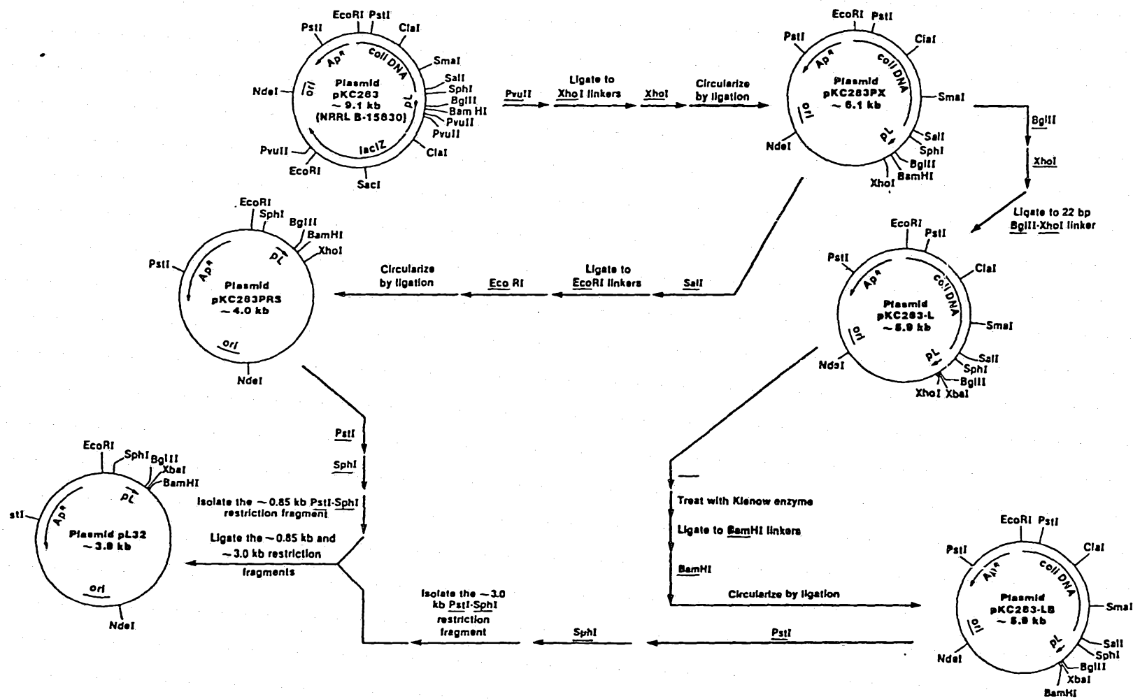
FIG. 1 Construction of Plasmid pL32
