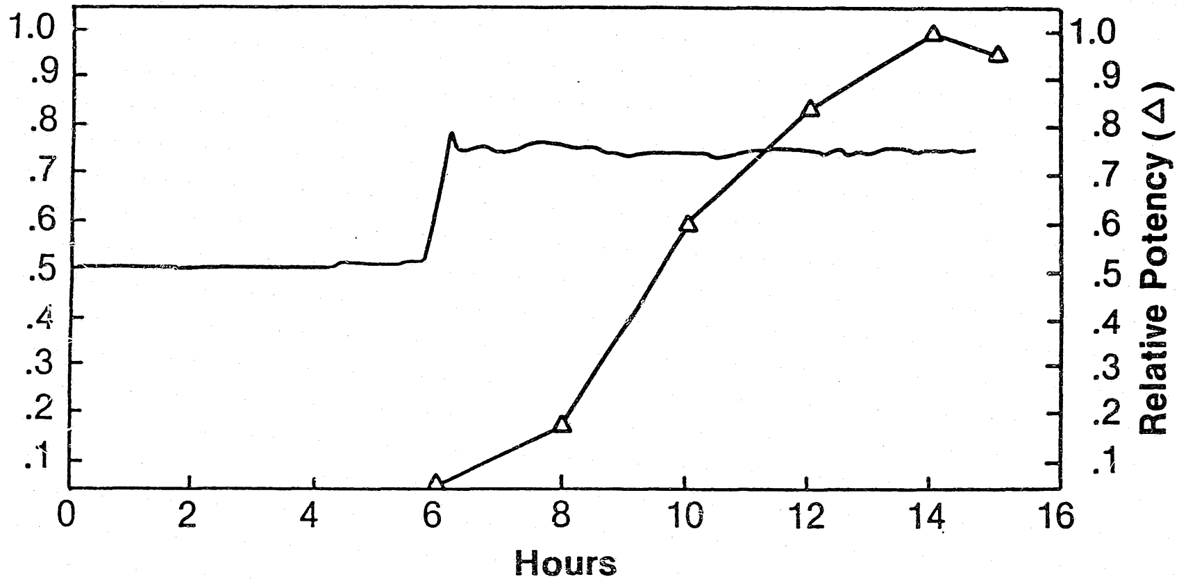
FIG.6 A Fermentation Process Using Cinoxacin to Control Aberrant Expression Vector Replication During Production of EK-bGH
