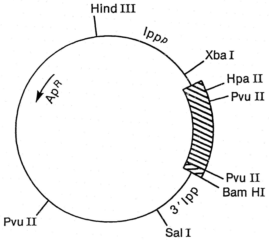
FIG.2 Restriction Site and Function Map of Plasmid pNM789
