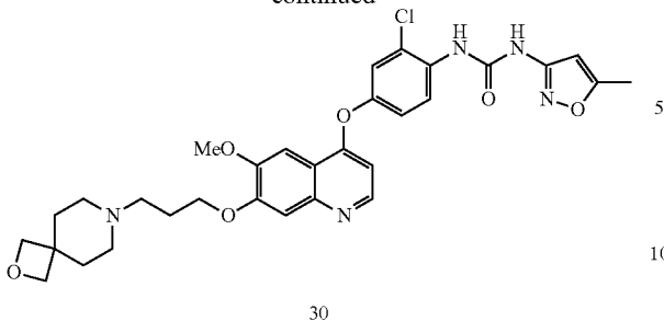
Compound 30
