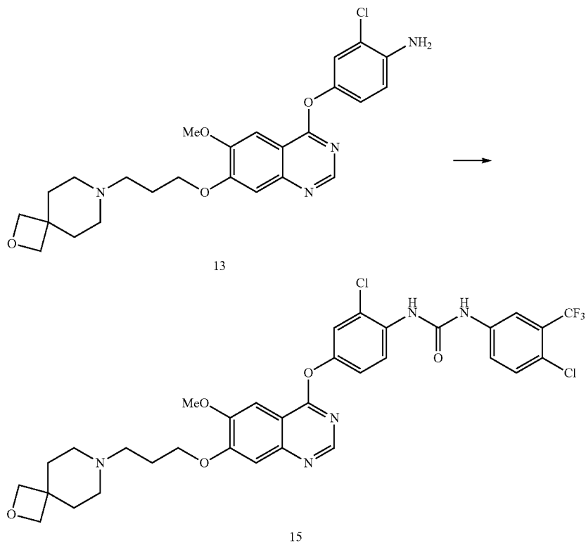
Compound 15
