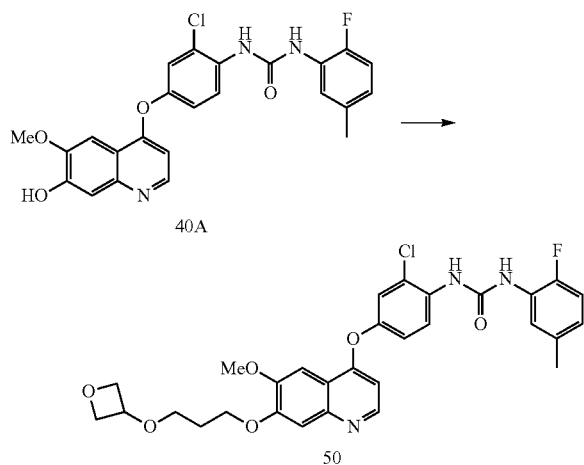
Compound 50
