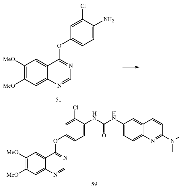
Compound 59
