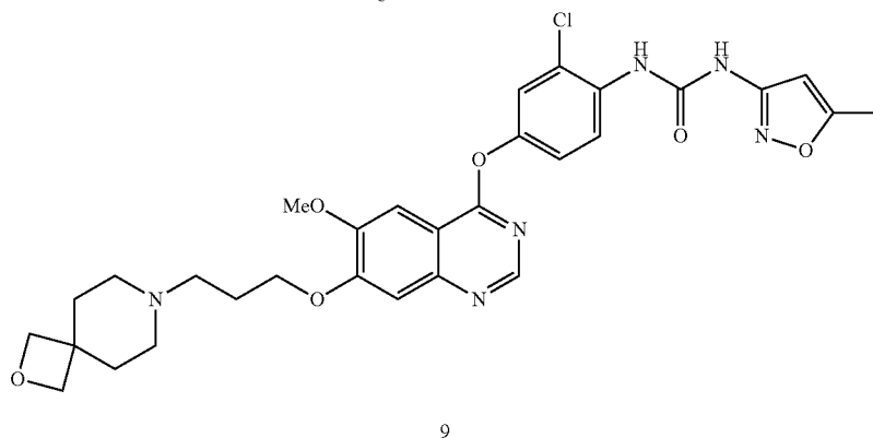
Compound 9
