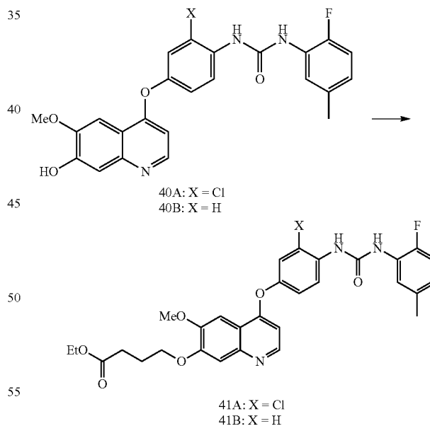
Compound 41
