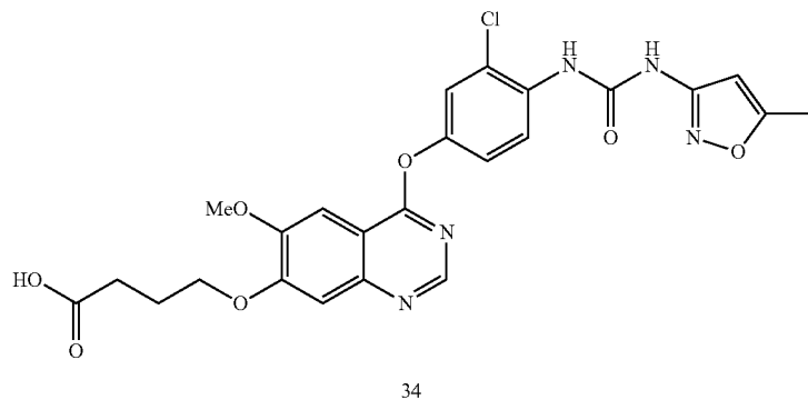
Compound 34
