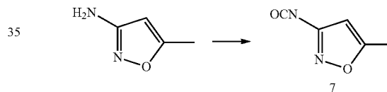
Compound 7
