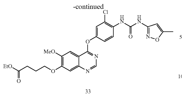
Compound 33
