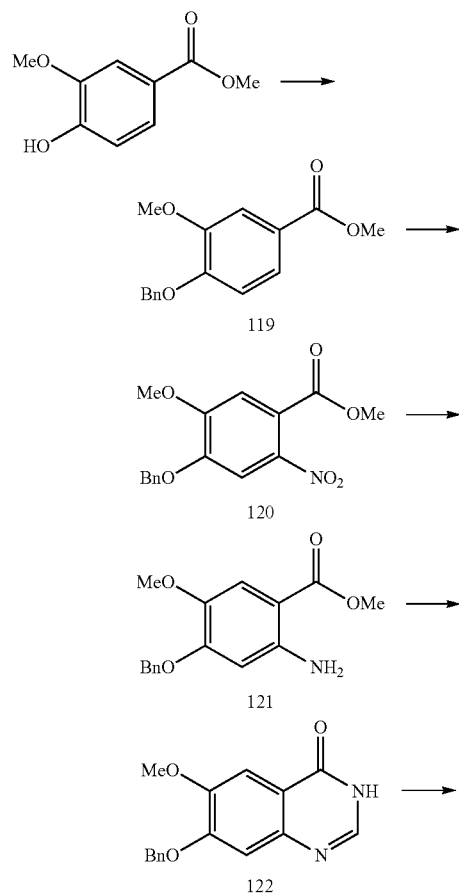
Scheme 3
