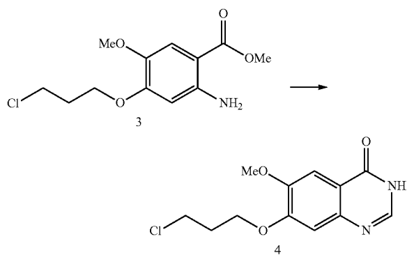
Compound 4
