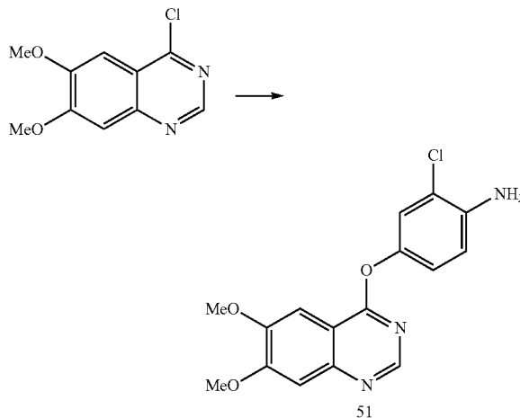
Compound 51
