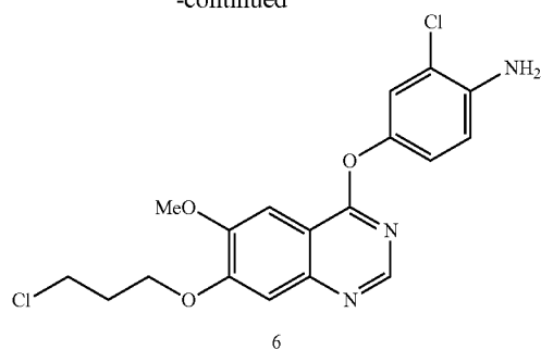
Compound 6
