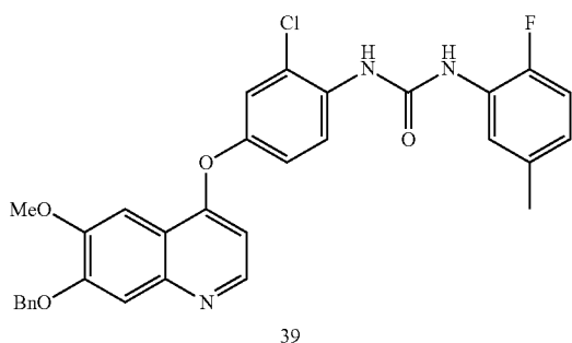
Compound 39
