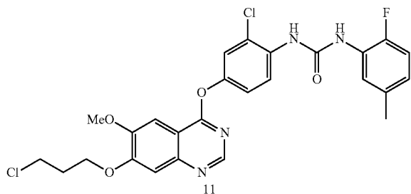
Compound 11
