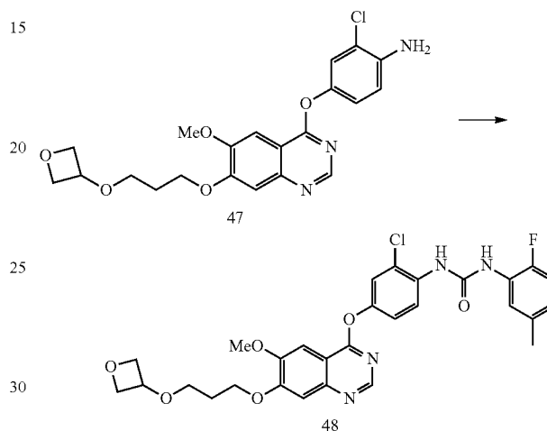
Compound 48
