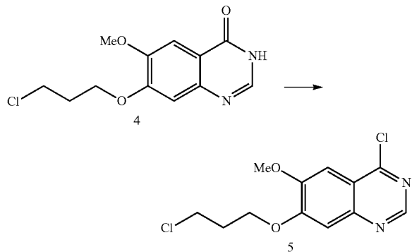
Compound 5
