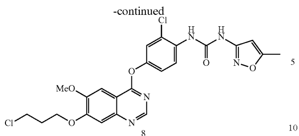
Compound 8
