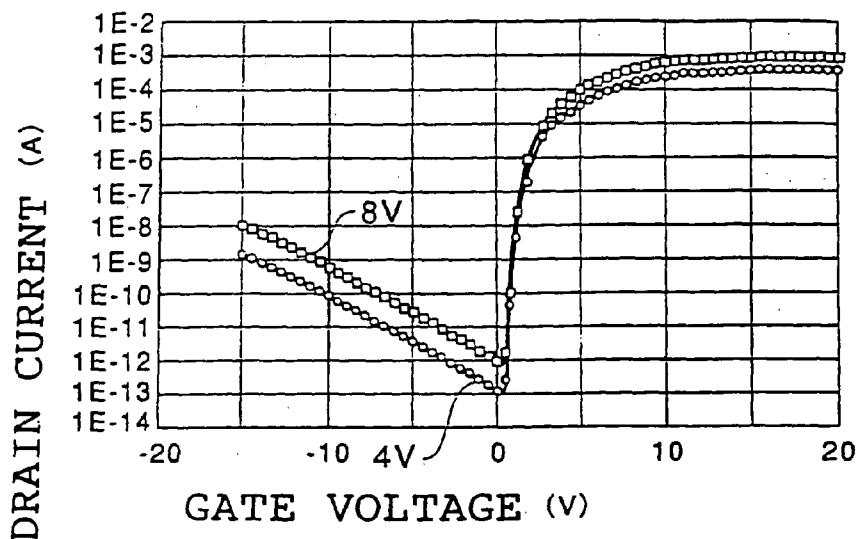
FIG. 11 AMPERE/VOLT CHARACTERISTICS N CHANNEL TYPE TFT
