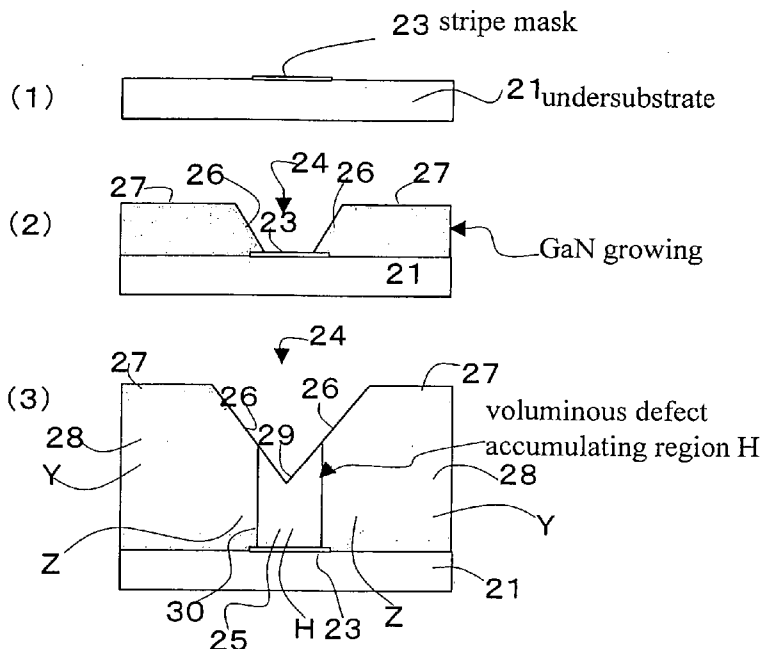
Relation between mask and voluminous defect accumulating region H in the present invention
