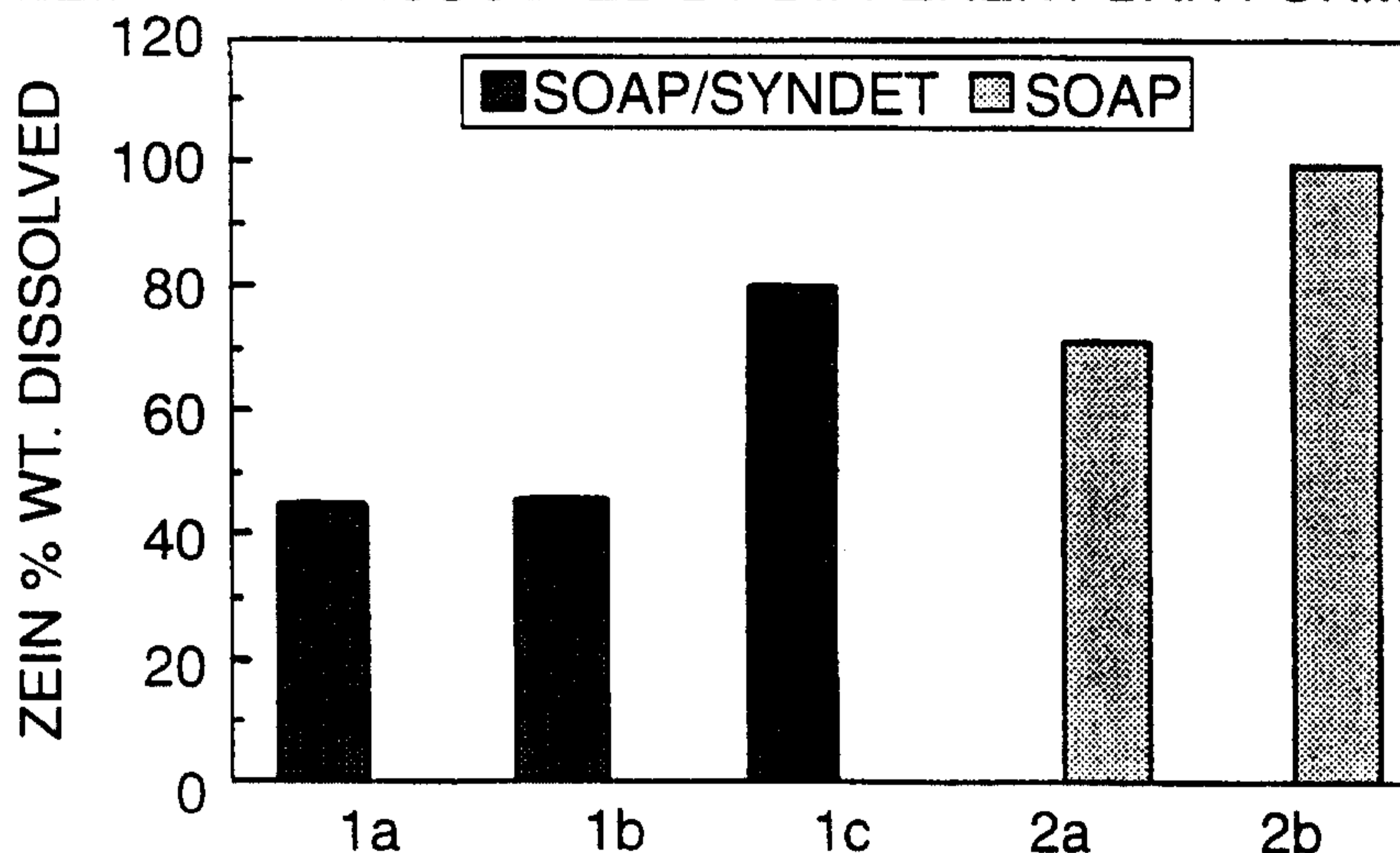
ZEIN% WT. DISSOLVED BY DIFFERENT BAR FORMULATIONS
