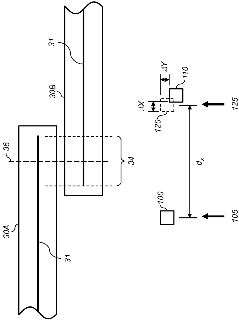
FIG. 3 (Prior Art)
