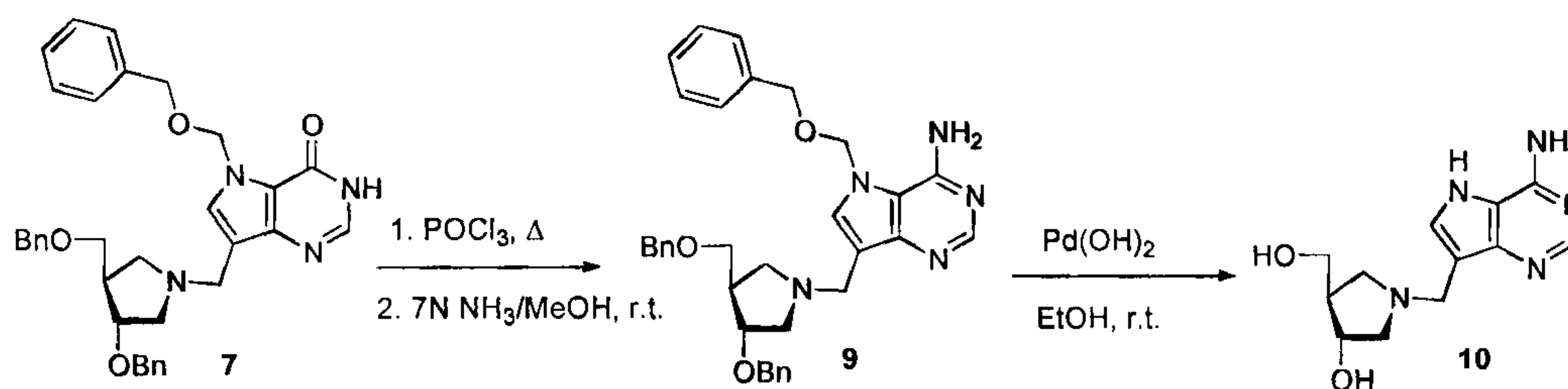
Scheme 4
