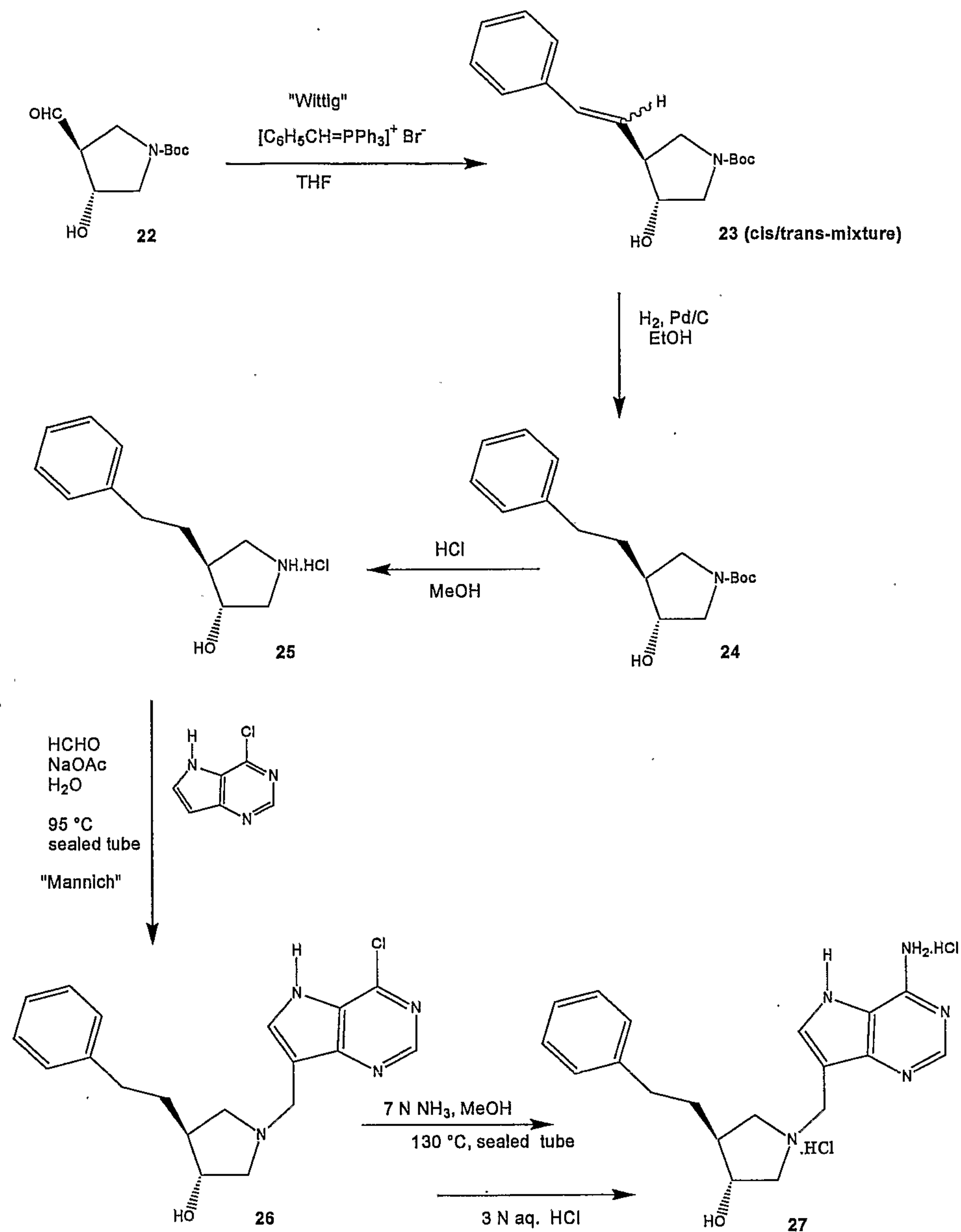
Scheme 7
