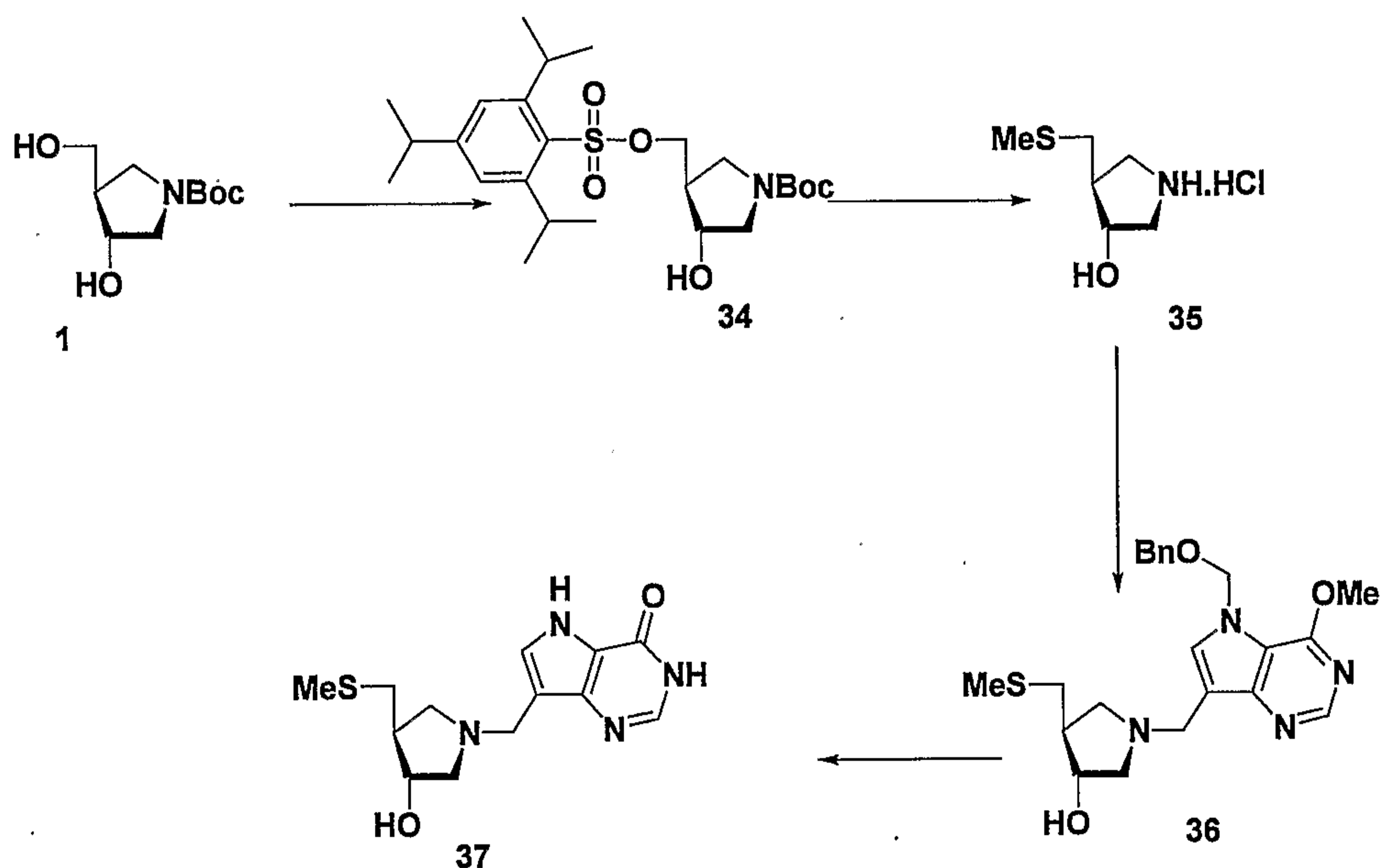
Scheme 10
