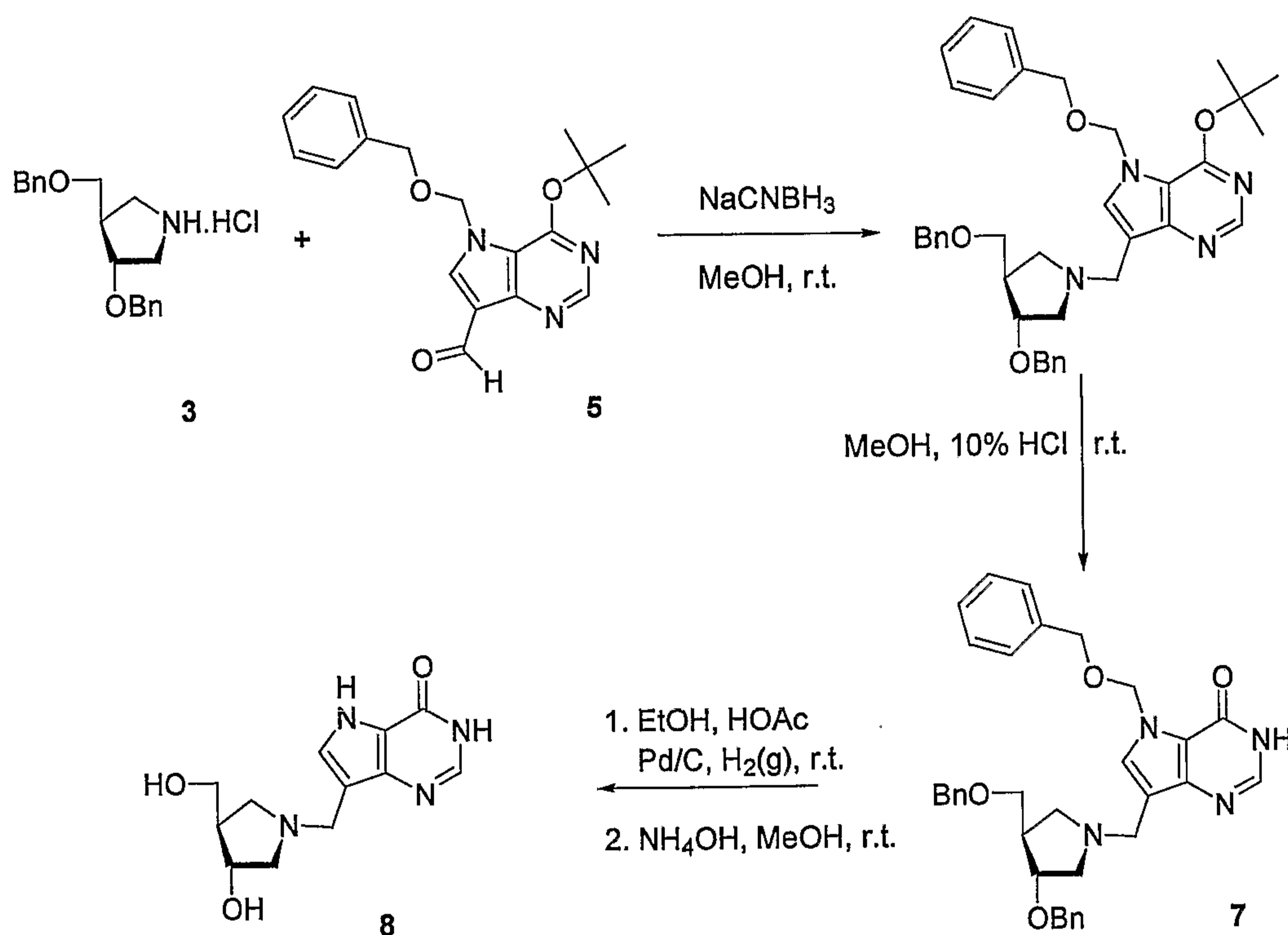
Scheme 3
