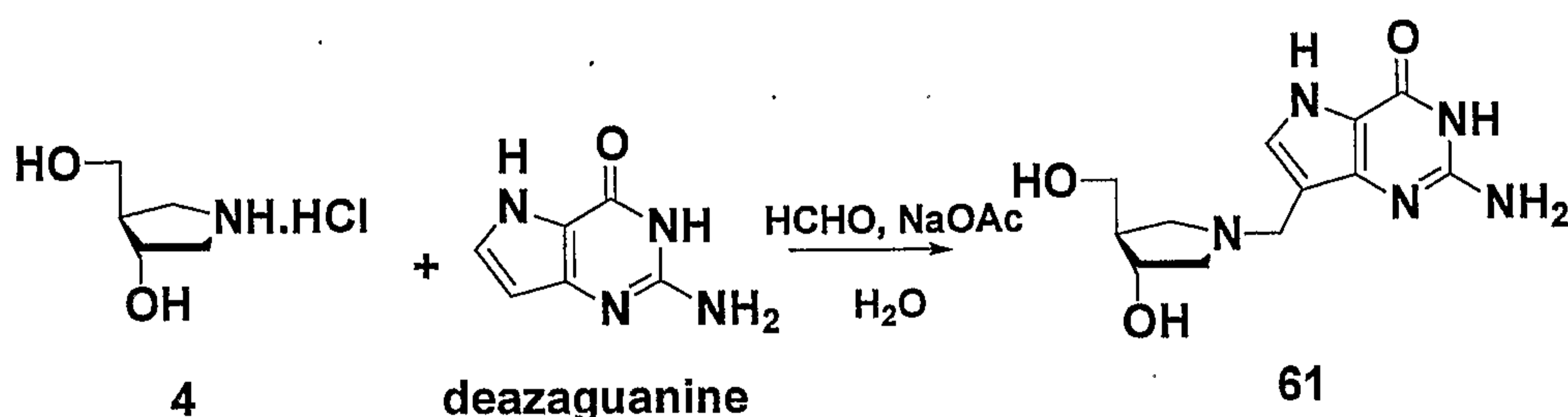
Scheme 17
