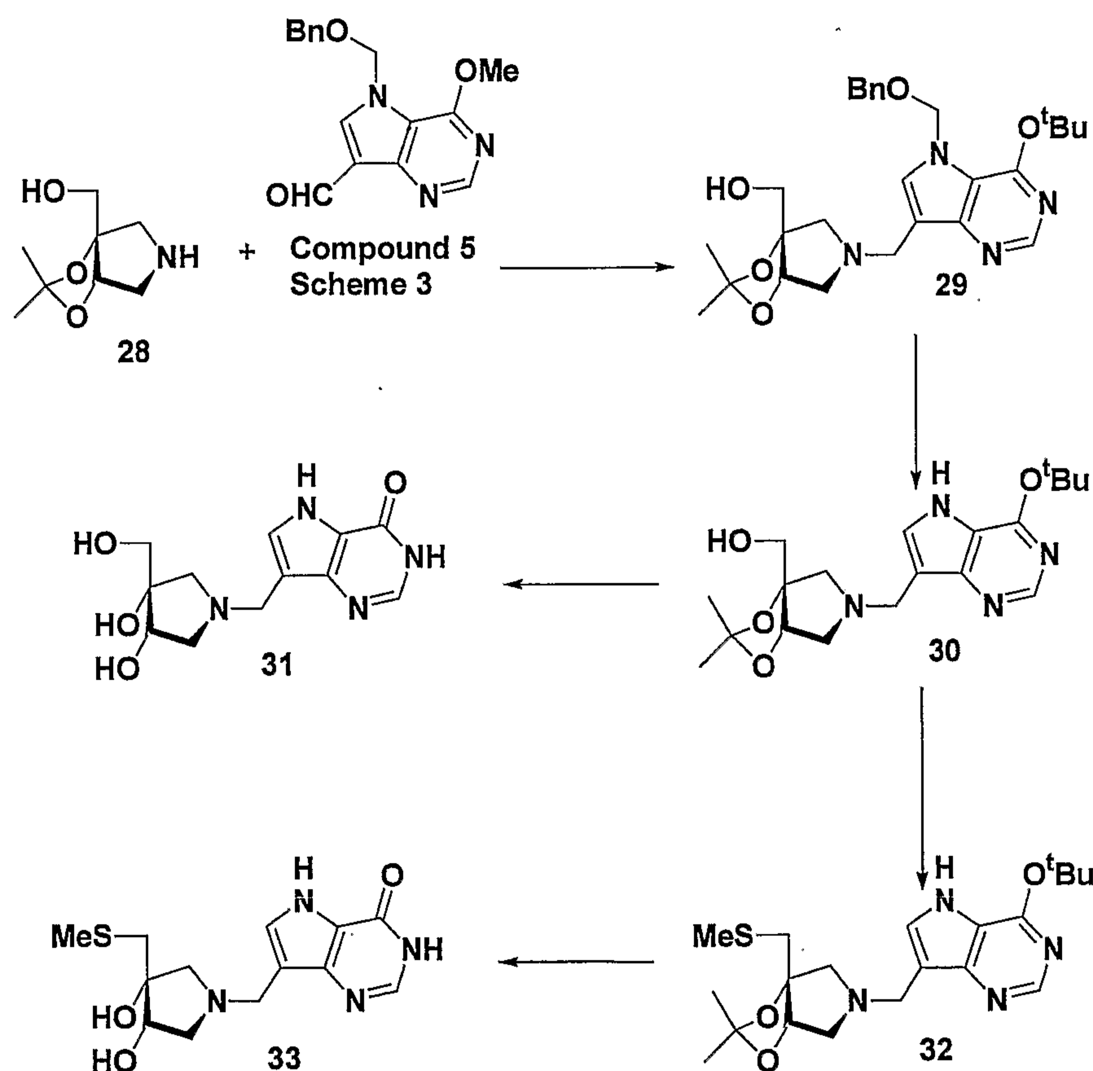
Scheme 9
