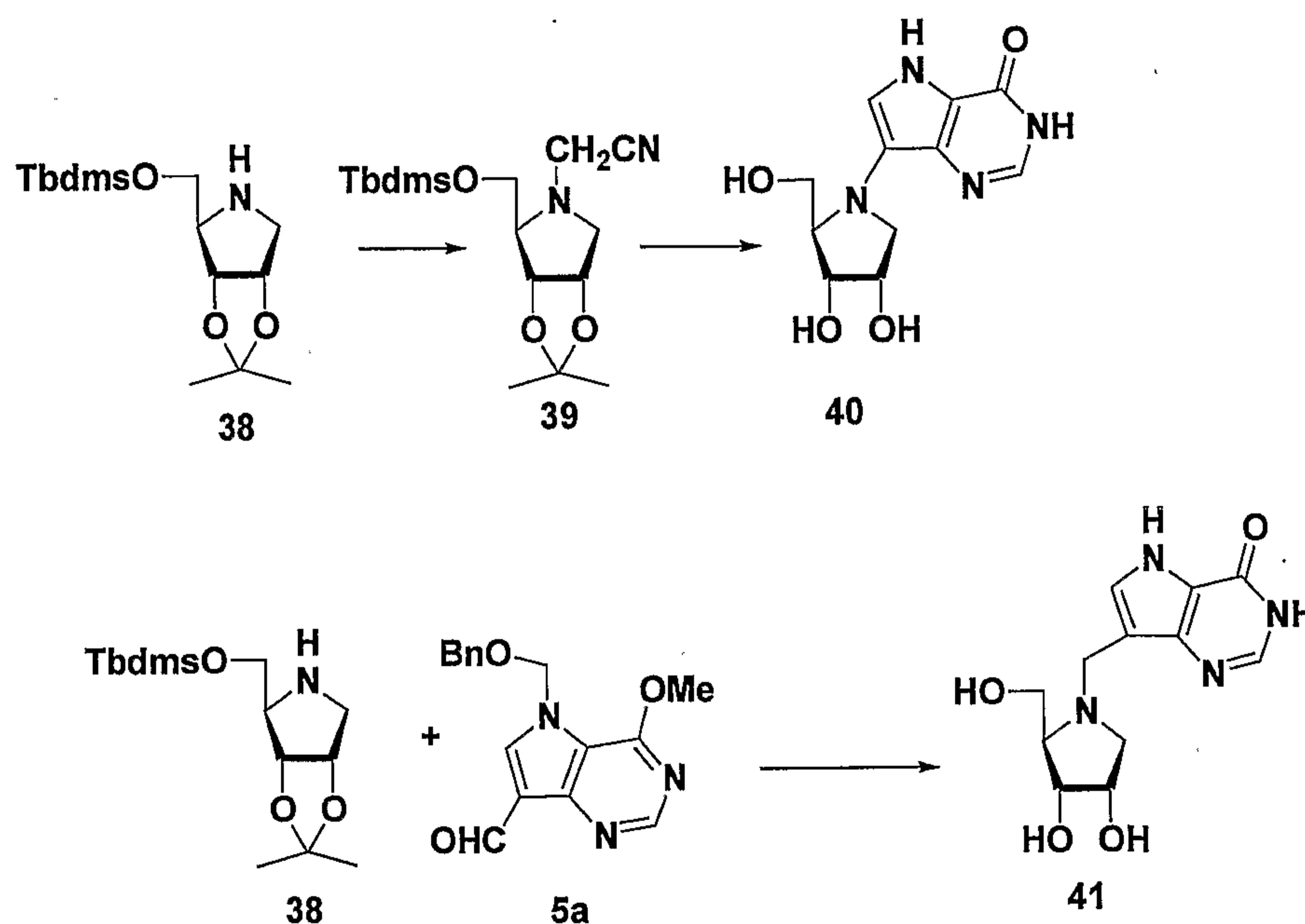
Scheme 11
