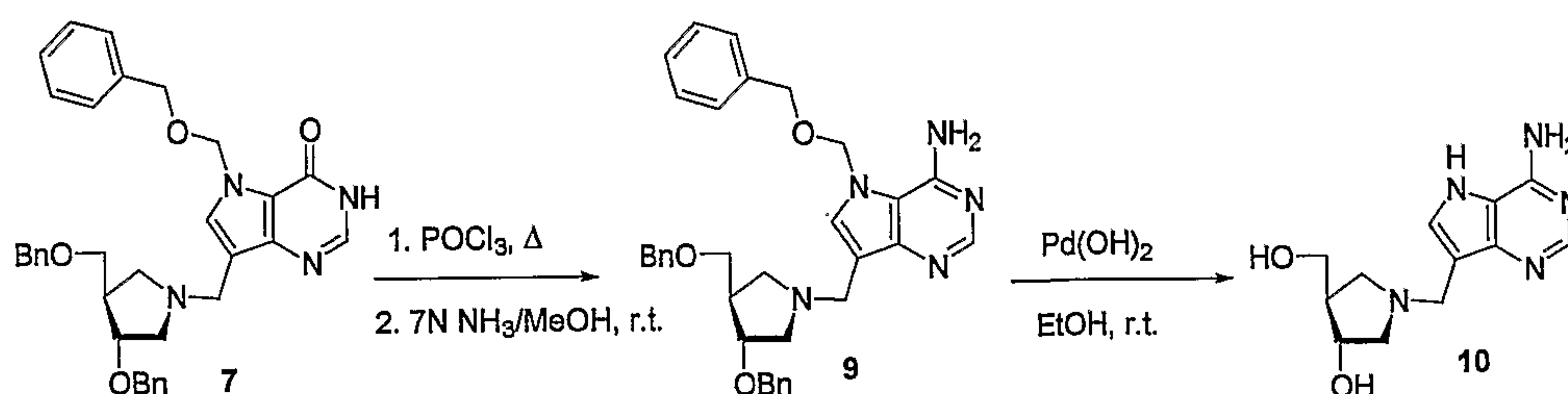
Scheme 4
