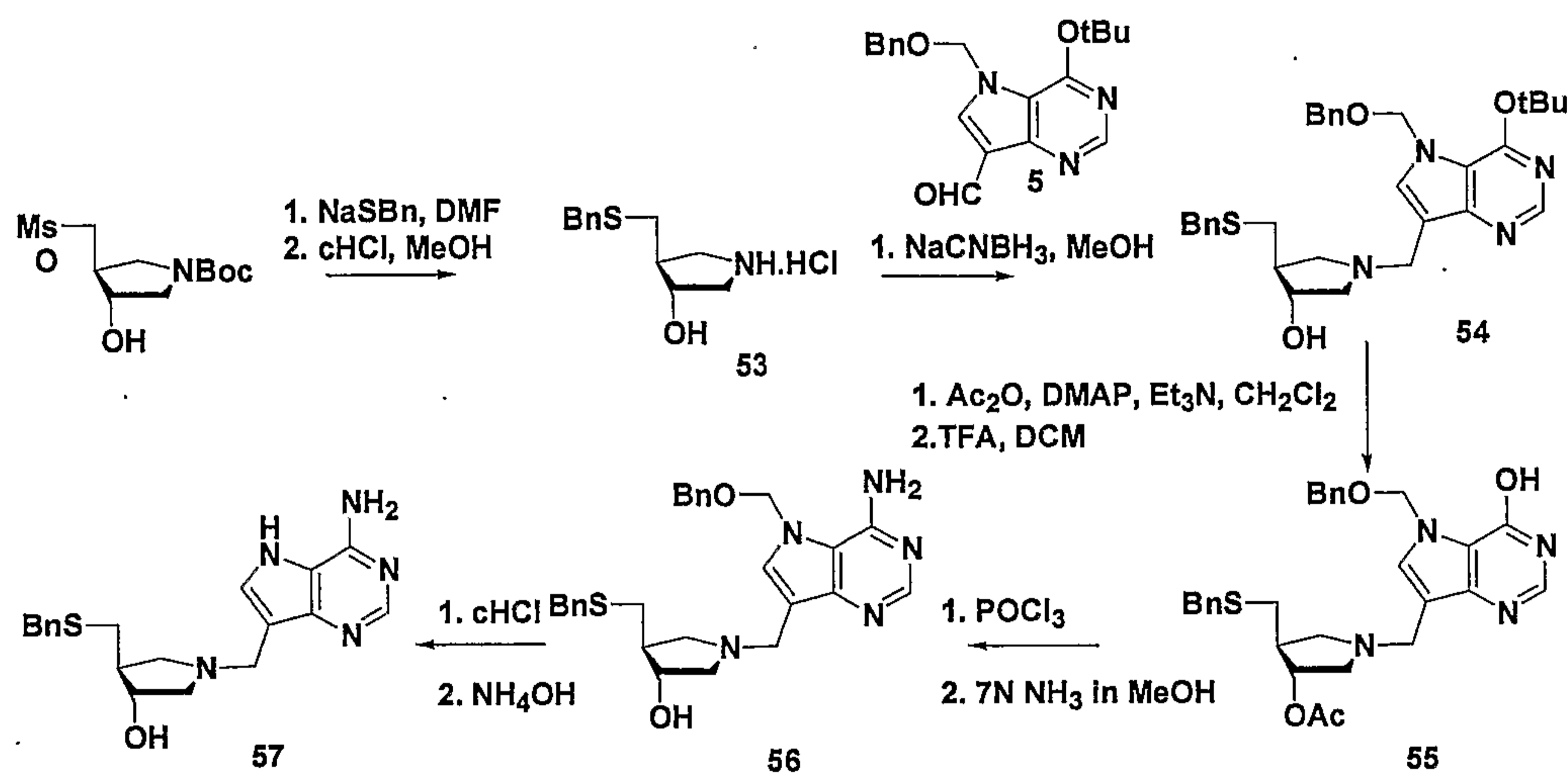
Scheme 14
