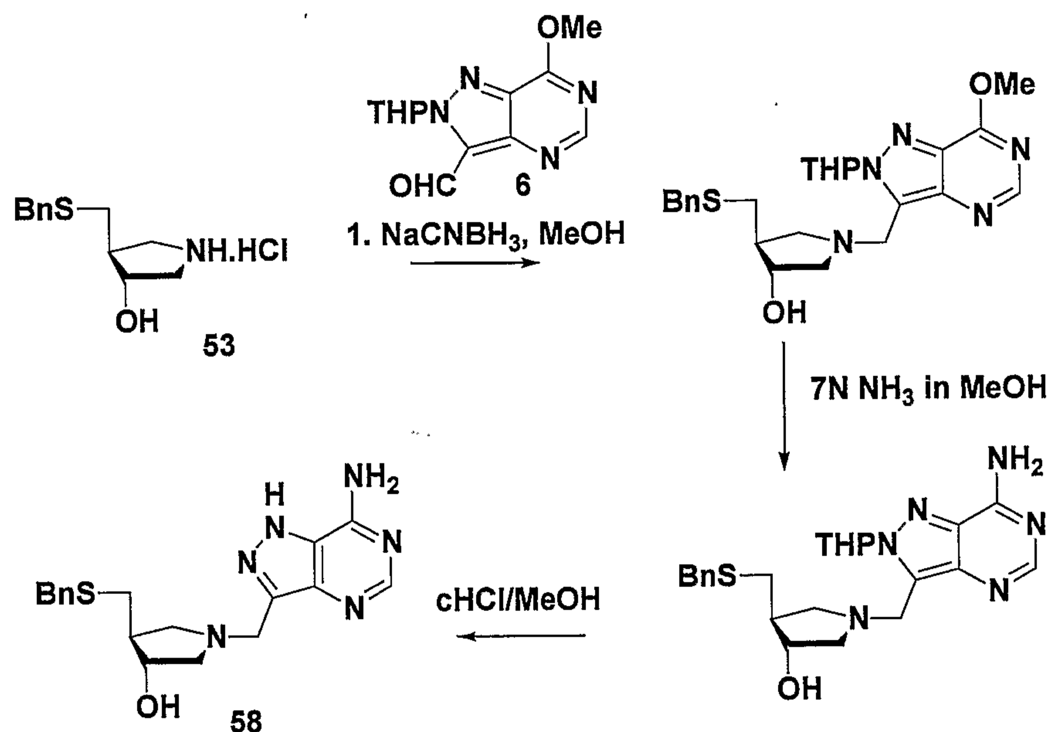
Scheme 15
