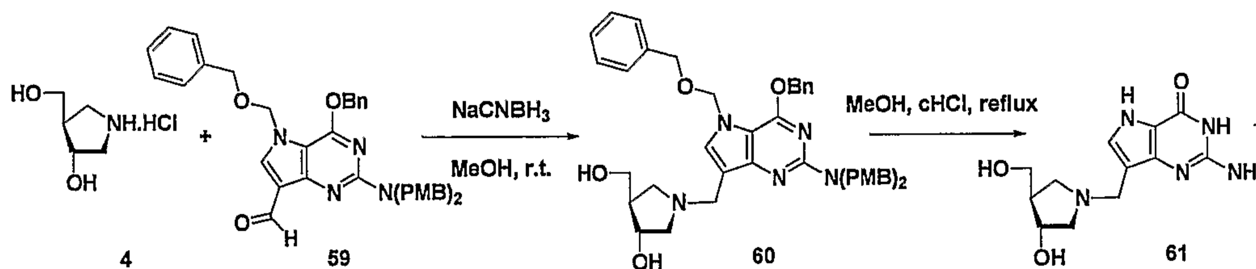
Scheme 16
