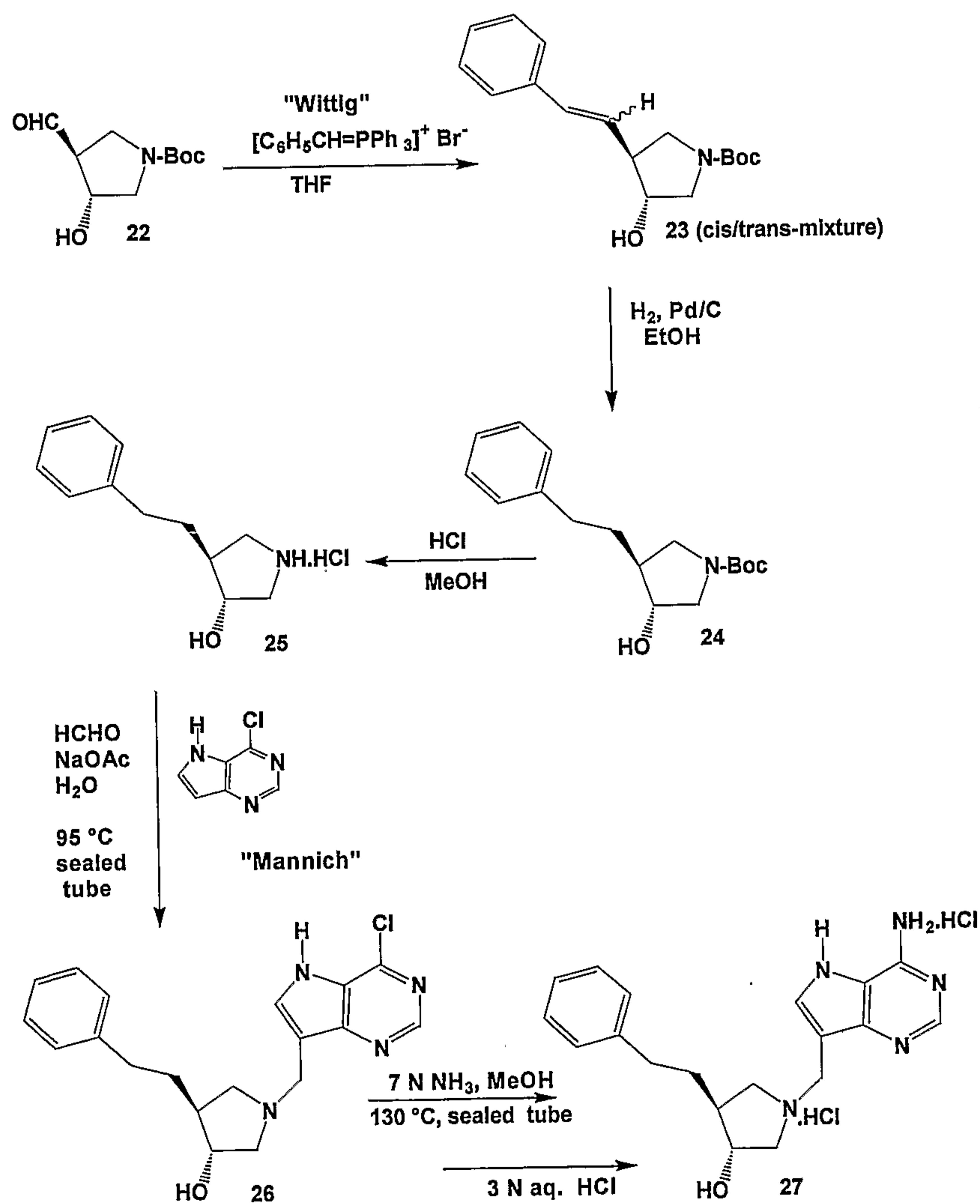
Scheme 7
