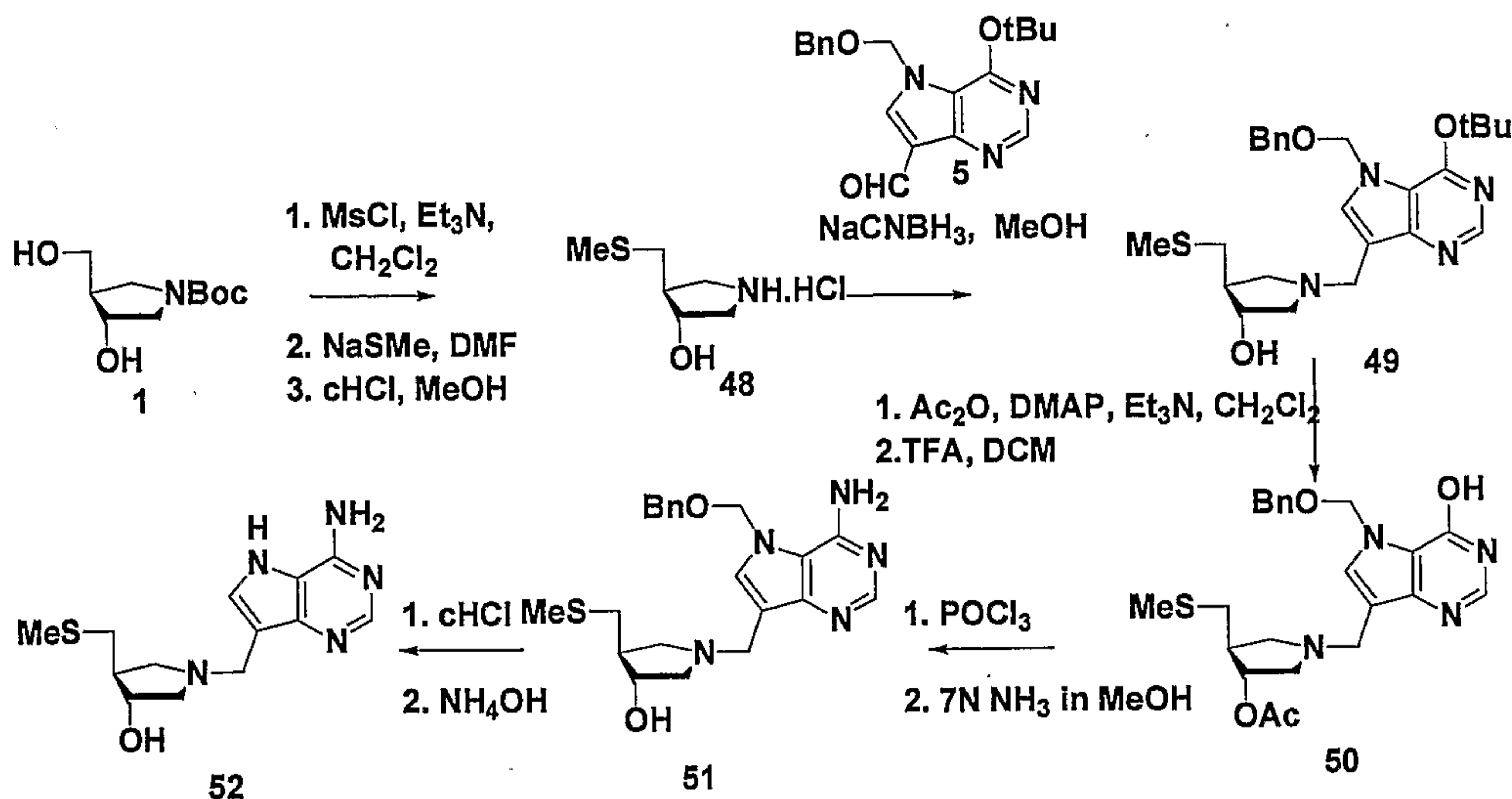
Scheme 13
