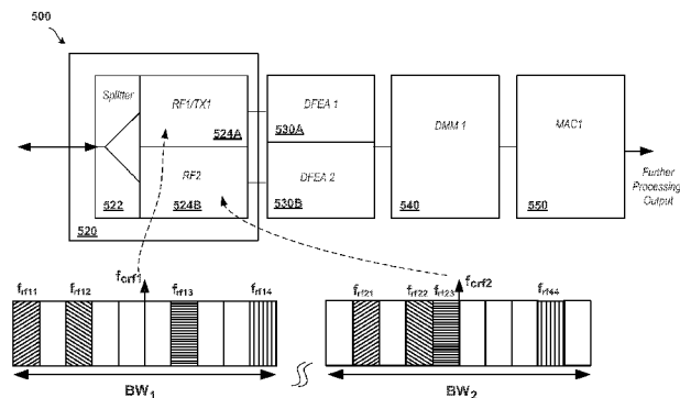
FIG. 5 Example of Channel Bonding Over Multiple Bands
