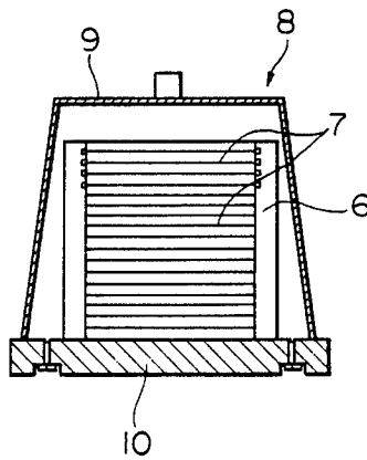
FIG. 2 PRIOR ART
