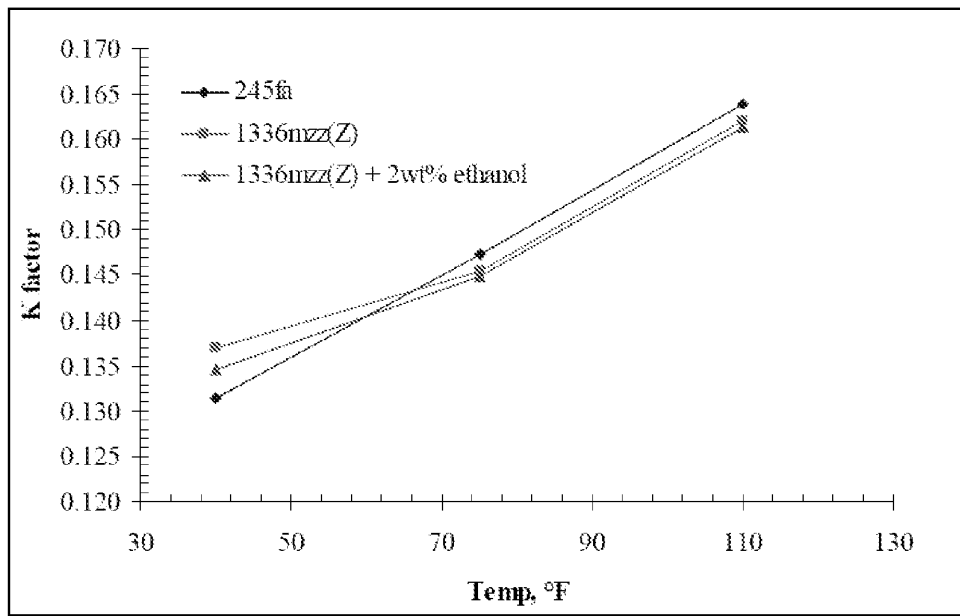
Figure 1. k factors of polyurethane foams
