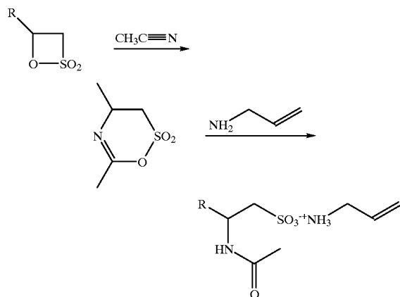
Scheme VII: 2-Acetamidoalkyl-1-Sulfonic Acid Allyl Amine Salts
