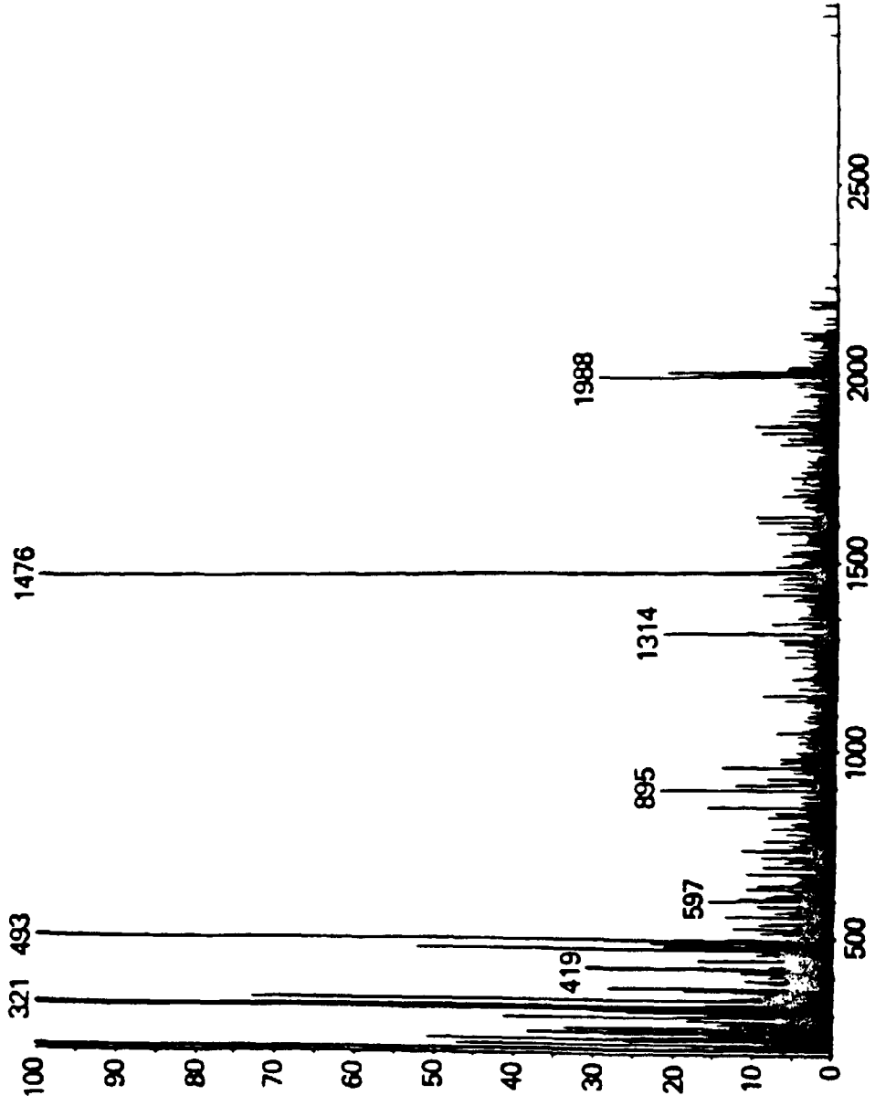
Figure 8C FAB-MS, OA-21
