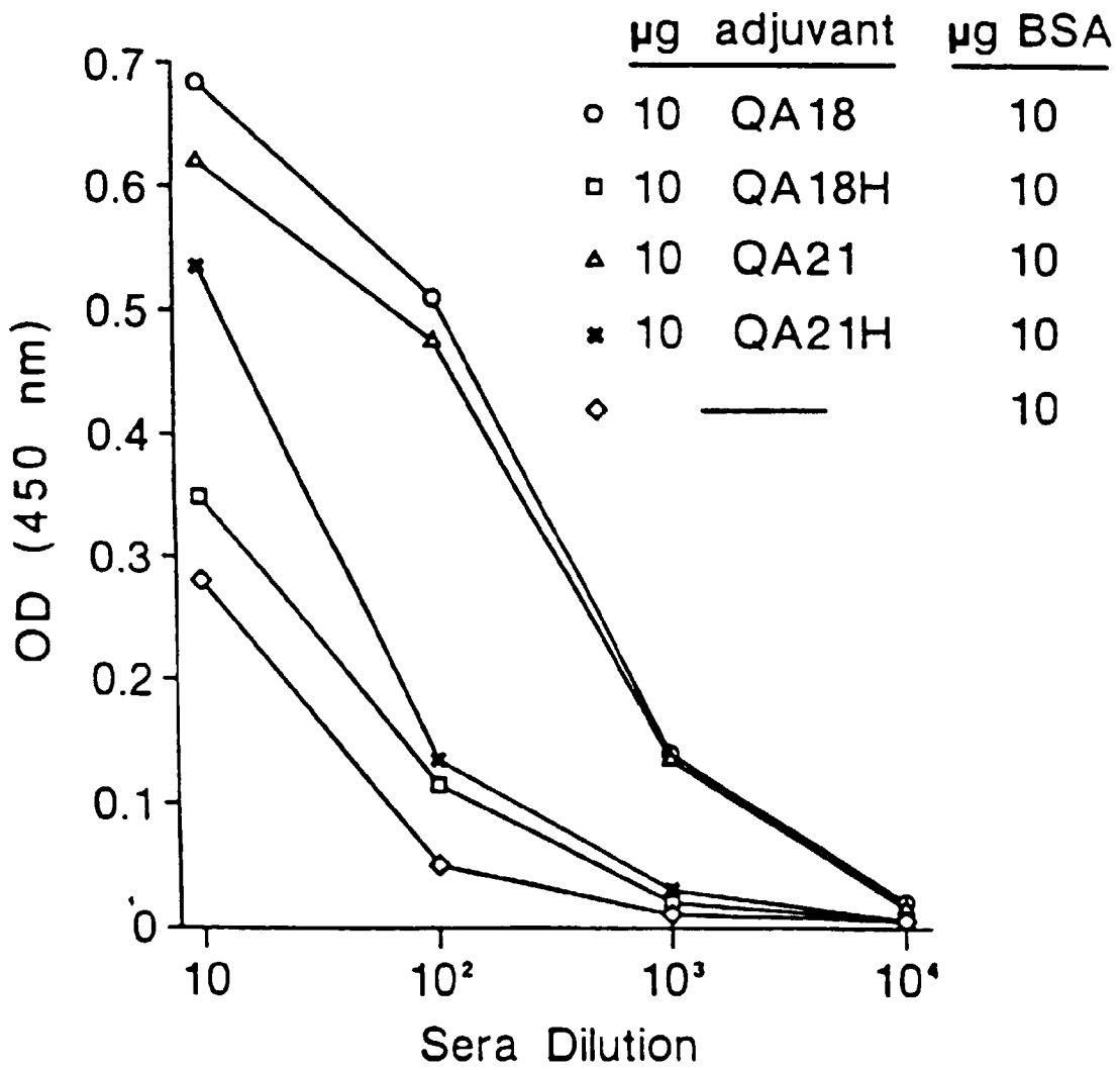
Figure 15 Anti-BSA ELISA
