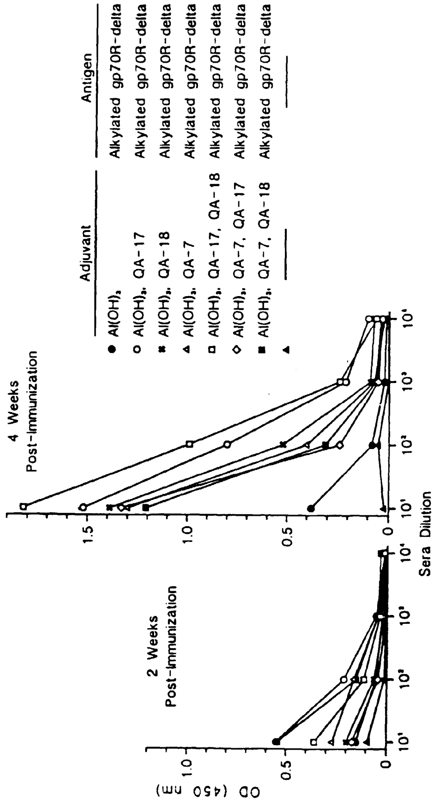
Figure 14 Anti-FelV ELISA
