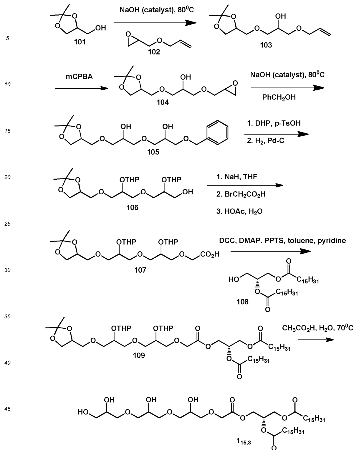
Scheme 1: synthetic route towards (2S)-9,13,17,18-tetrahydroxy-5-oxo-4,7,11,15-tetraoxaocetadecane-1,2-diyl dipalmitate 1 15,3 .
