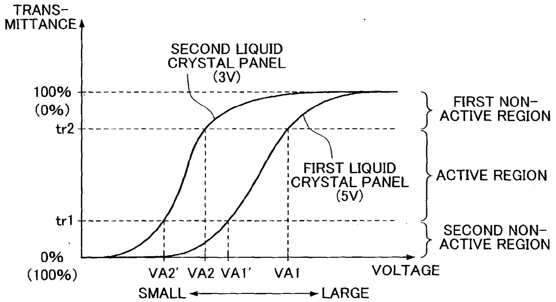
RELATION BETWEEN TRANSMITTANCE AND APPLIED VOLTAGE
