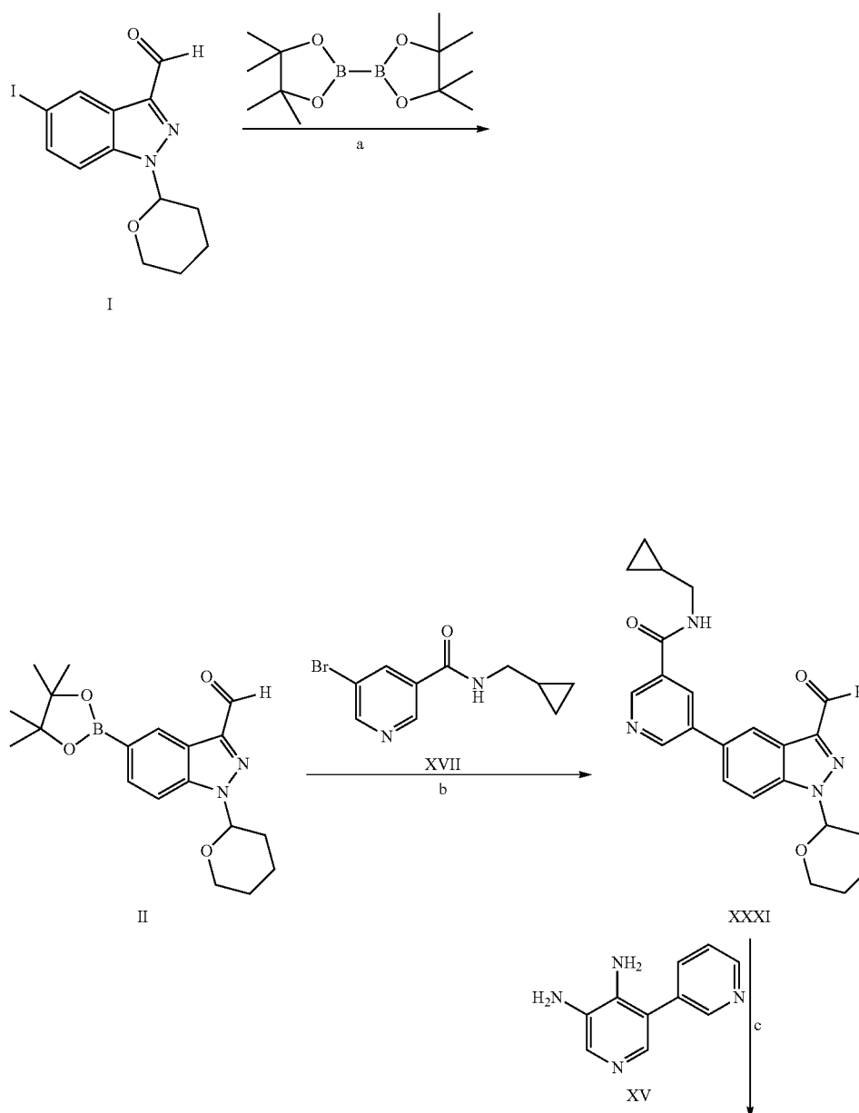
Scheme 6
