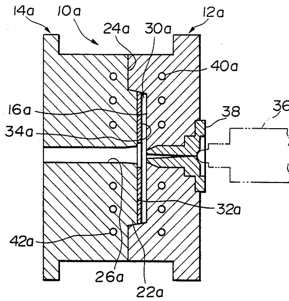
FIG. 1 (PRIOR ART)
