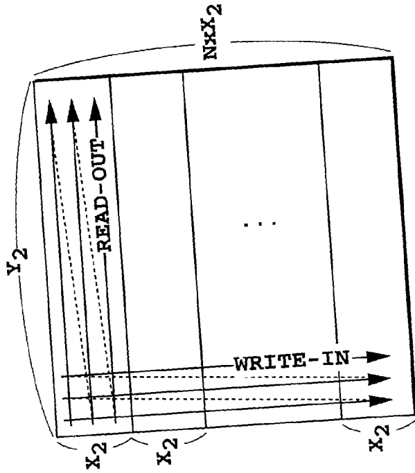
INTERLEAVER
