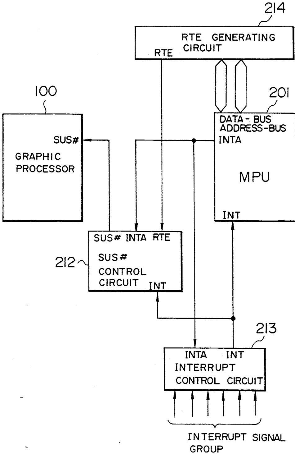
CONTROL OF SUS# SIGNAL
