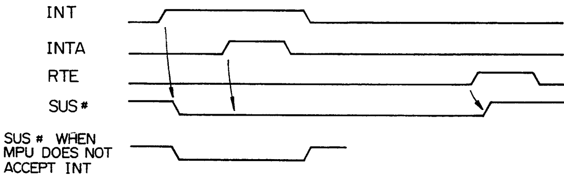
SUS# SIGNAL CONTROL
