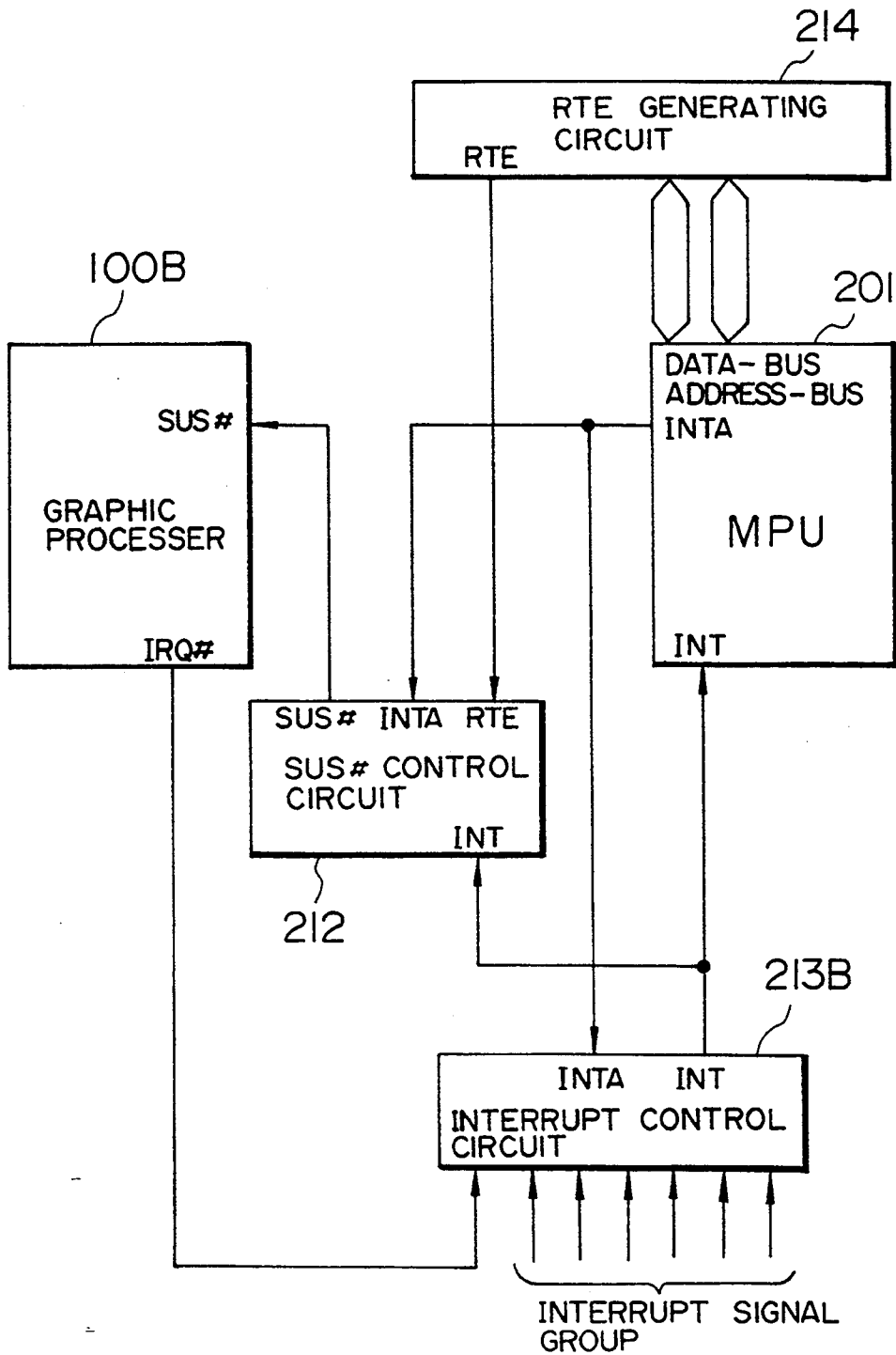
FIG. 22 ASSERTING IRQ# SIGNAL BY SUS# SIGNAL
