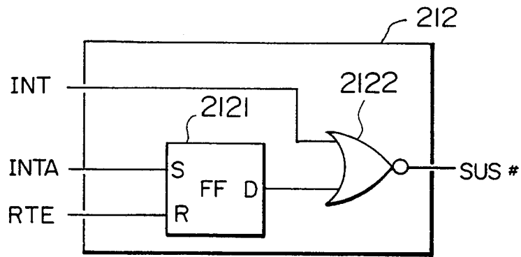
SUS# SIGNAL CONTROL LOGIC
