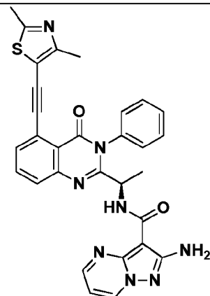
Compound 2079r,
