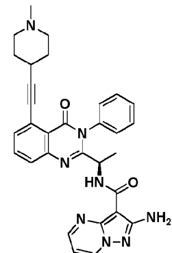
Compound 2085r,
