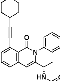
Compound 23,
