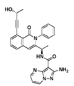
Compound 15r,
