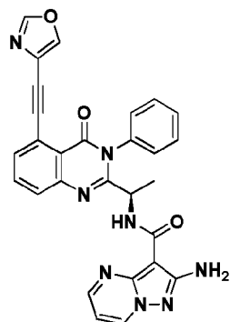
Compound 2066r,
