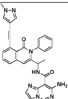
Compound 1073 ' ,
