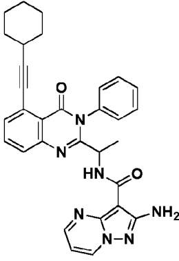
Compound 2065',
