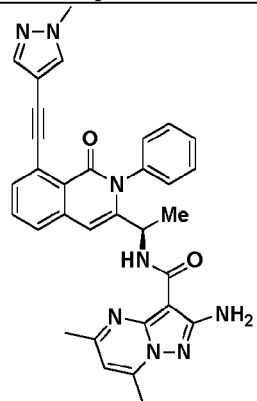
Compound 108r,
