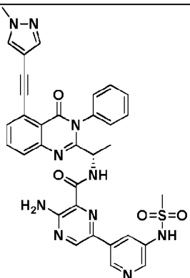
Compound 3065,
