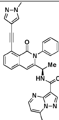
Compound 102r,
