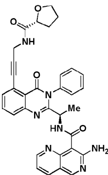
Compound 3081r,
