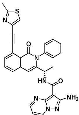
Compound 40,
