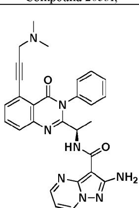
Compound 2057r,
