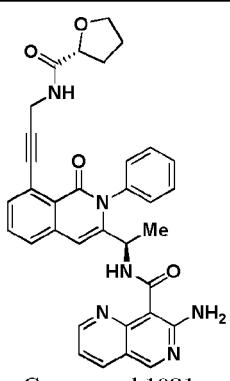
Compound 1081r,
