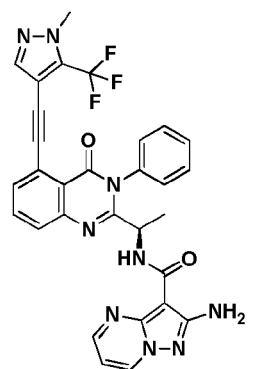
Compound 2069r,
