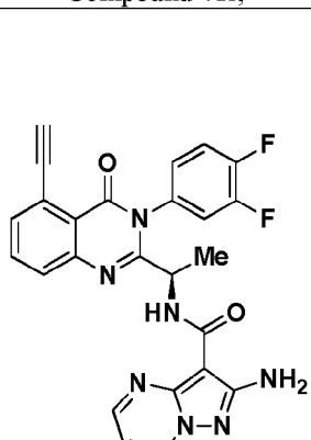
Compound 45r,
