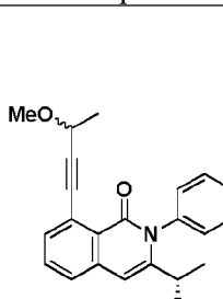
Compound 18,
