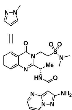
Compound 2104,
