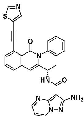
Compound 41,
