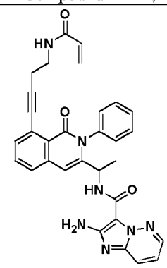
Compound 1088 ' ,
