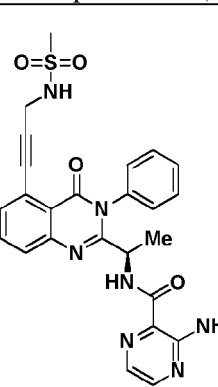
Compound 3079r,
