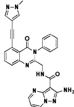
Compound 2107,
