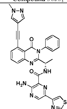
Compound 3057,
