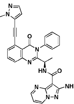
Compound 2073r,
