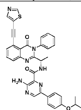
Compound 3064,
