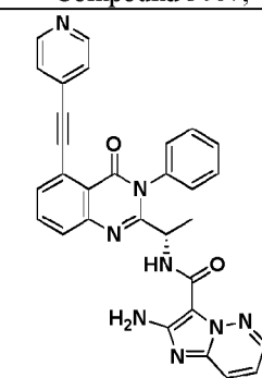
Compound 3071,
