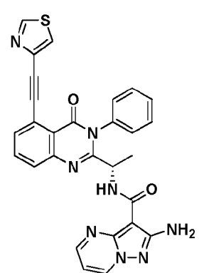
Compound 2054,
