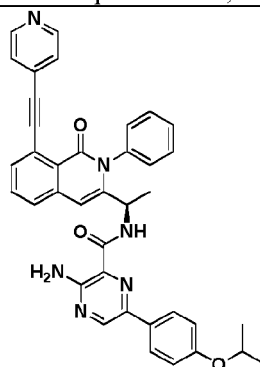
Compound 1063r,
