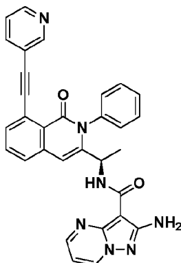
Compound 17r,
