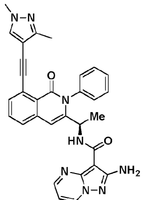
Compound 19r,
