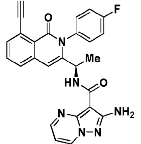
Compound 2050r,
