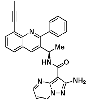
Compound 51r,
