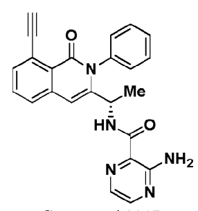
Compound 2047,
