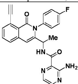
Compound 2049',
