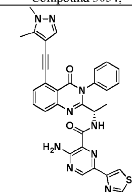
Compound 3058,
