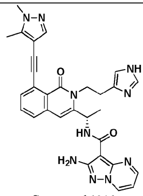
Compound 1046,
