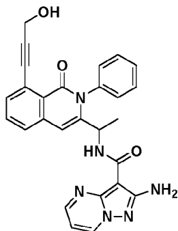
Compound 13',
