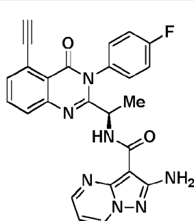
Compound 50r,
