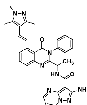
Compound 3008',
