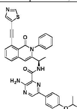
Compound 1064r,
