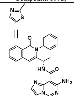
Compound 1076,
