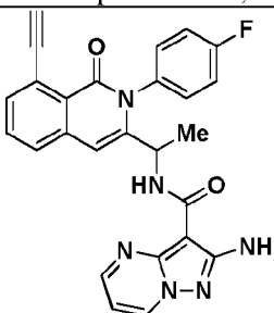
Compound 2050',
