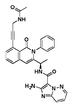
Compound 1086r,
