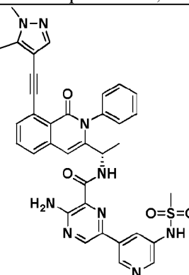
Compound 1066,
