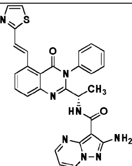
Compound 3003,
