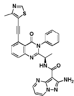
Compound 2075r,
