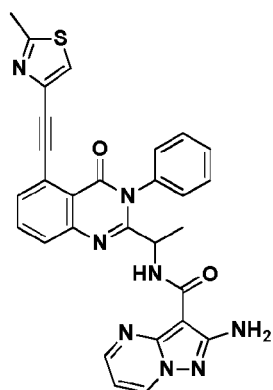
Compound 2040',
