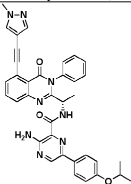
Compound 3061,
