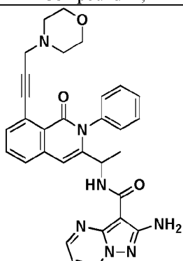
Compound 10',
