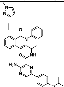
Compound 1062r,
