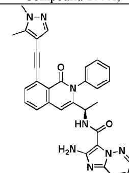
Compound 1070r,
