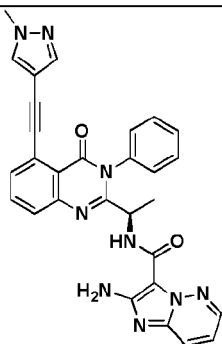
Compound 3069r,
