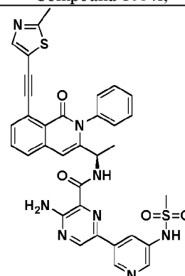
Compound 1068r,
