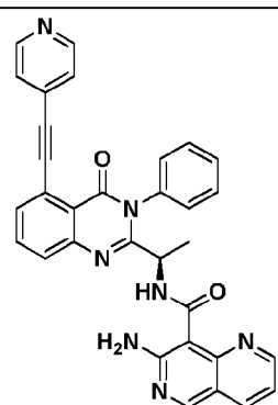
Compound 3055r,
