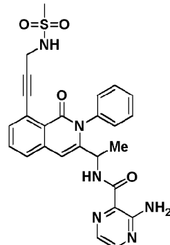
Compound 1079 ' ,
