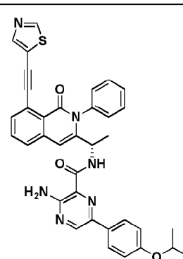
Compound 1064,
