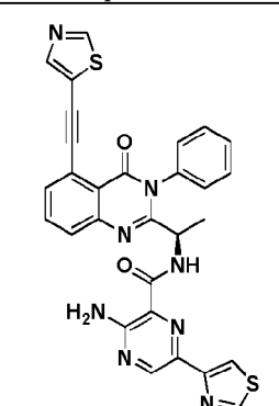
Compound 3060r,
