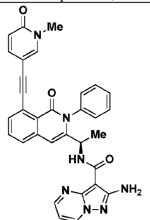
Compound 20r,
