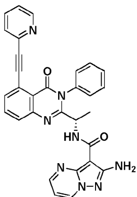
Compound 2032,
