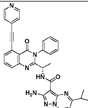
Compound 3051,
