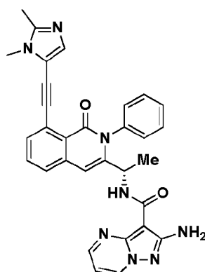
Compound 38,
