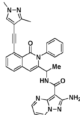
Compound 19',
