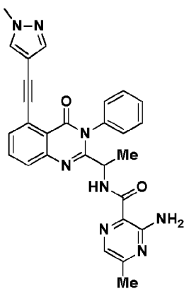
Compound 2068',
