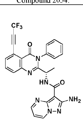
Compound 2058,
