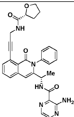
Compound 1077,
