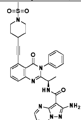
Compound 2083r,
