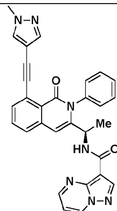
Compound 39r,
