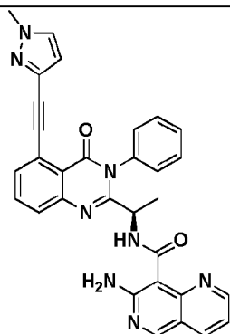
Compound 3054r,
