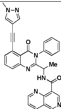
Compound 2042',
