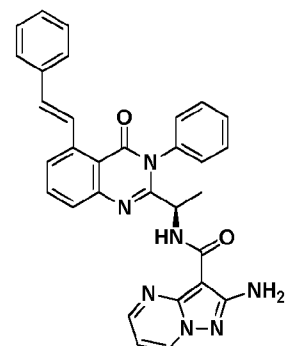
Compound 2087r,
