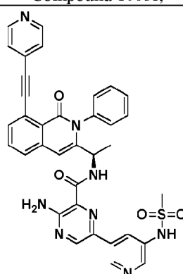
Compound 1067r,
