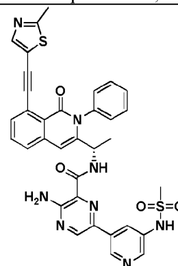
Compound 1068,
