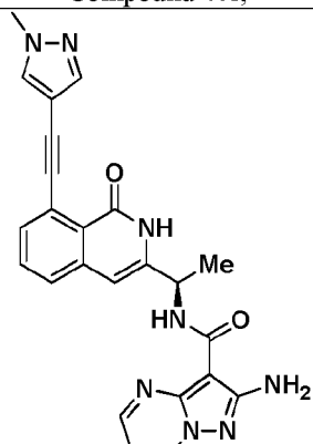
Compound 44r,
