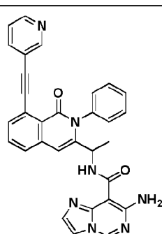
Compound 1075 ' ,
