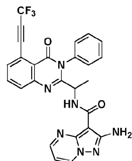
Compound 2058',
