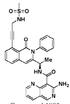
Compound 1083r,
