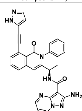
Compound 43r,
