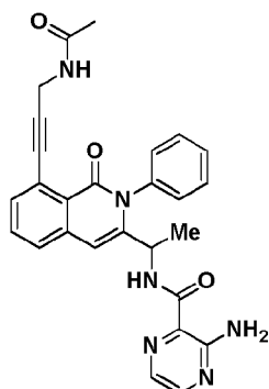
Compound 1078 ' ,
