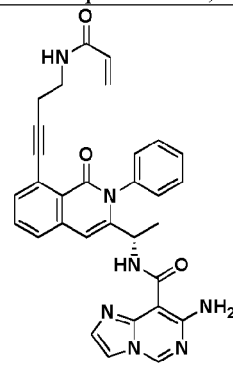
Compound 1092
