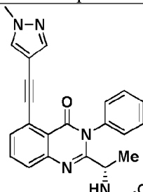
Compound 17,
