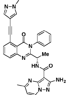
Compound 2106,
