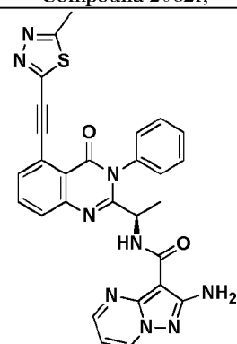
Compound 2086r,
