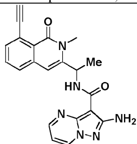
Compound 2048',
