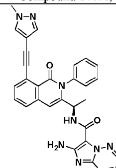
Compound 1069r,
