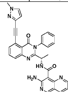
Compound 3054,
