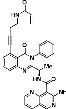
Compound 3084r,
