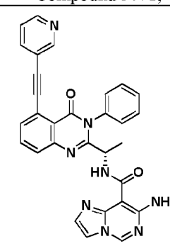
Compound 3075,
