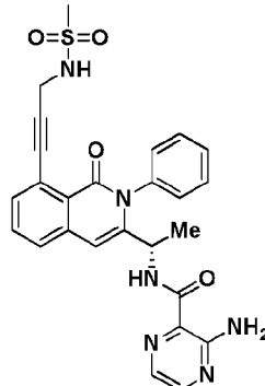
Compound 1079,
