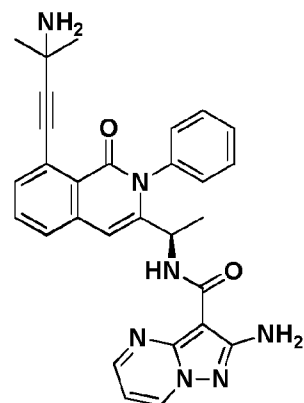
Compound 8r,
