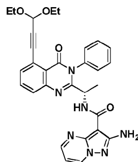
Compound 2034,
