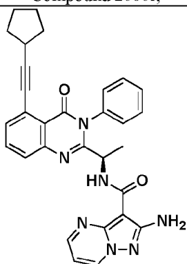
Compound 2064r,
