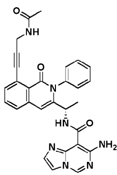
Compound 1090,
