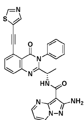
Compound 2041,
