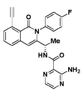
Compound 2049,
