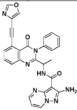
Compound 2066',
