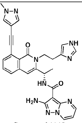
Compound 1045,
