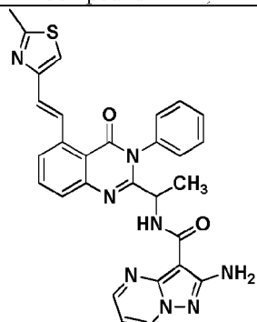
Compound 3005',
