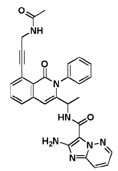
Compound 1086 ' ,
