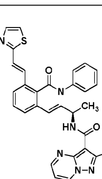
Compound 1003r,
