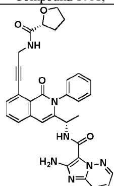
Compound 1085,
