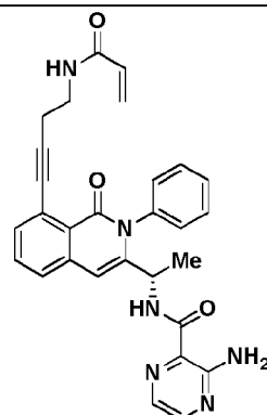
Compound 1080,
