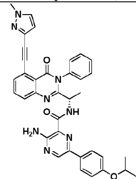
Compound 3062,
