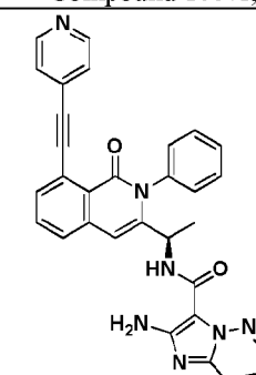
Compound 1071r,
