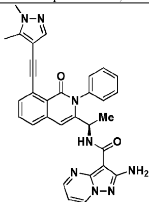
Compound 2088r,
