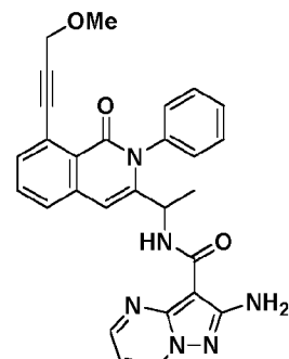
Compound 12',
