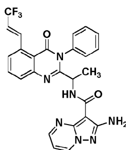
Compound 3001',
