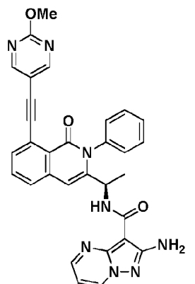
Compound 18r,
