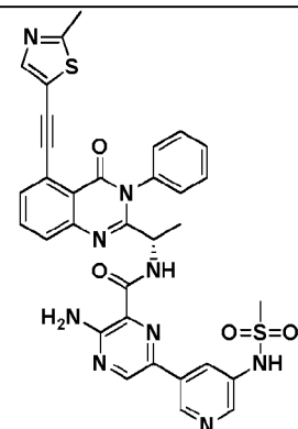
Compound 3068,
