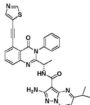
Compound 3052,
