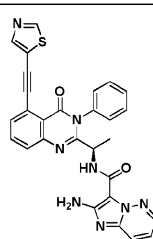
Compound 3072r,
