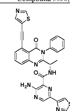
Compound 3060,
