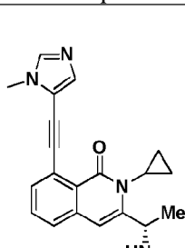
Compound 19,
