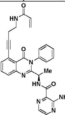
Compound 3080r,
