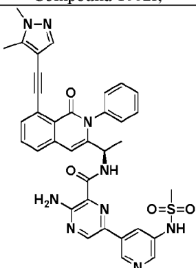
Compound 1066r,
