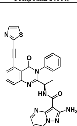
Compound 2059r,
