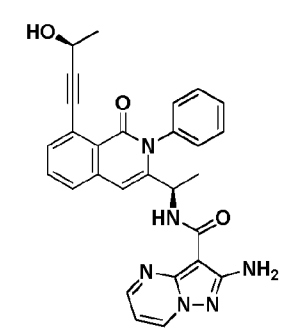
Compound 16r,
