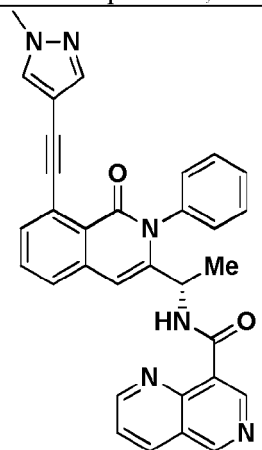
Compound 42,
