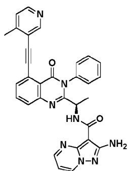
Compound 2061r,
