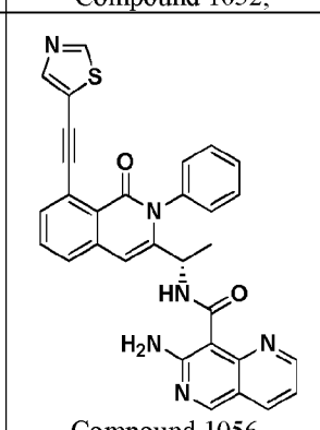
Compound 1056,
