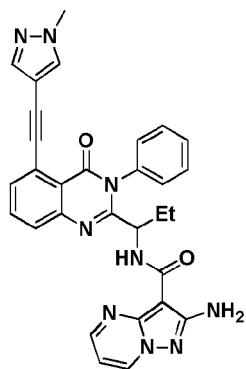
Compound 2105',
