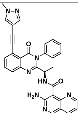
Compound 3053r,
