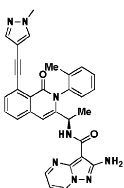
Compound 101r,
