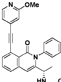
Compound 25,
