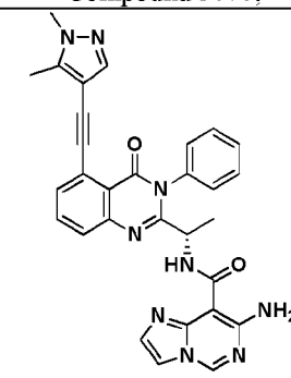
Compound 3074,
