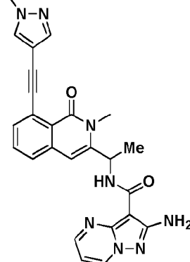
Compound 2055',
