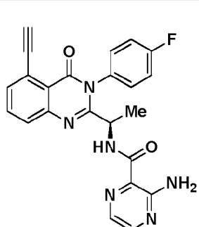
Compound 49r,
