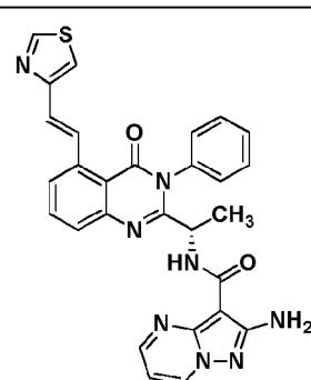
Compound 3004,
