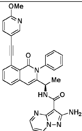
Compound 6r,
