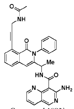
Compound 1082 ' ,
