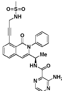
Compound 1079r,
