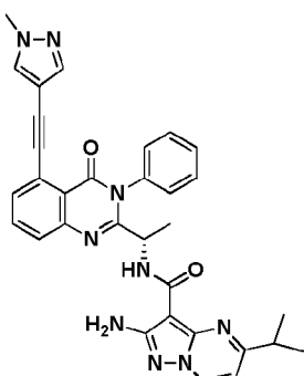
Compound 3049,
