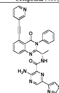
Compound 3059,
