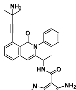
Compound 8',
