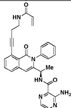
Compound 1080r,
