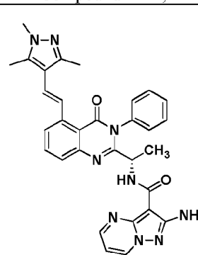
Compound 3008,
