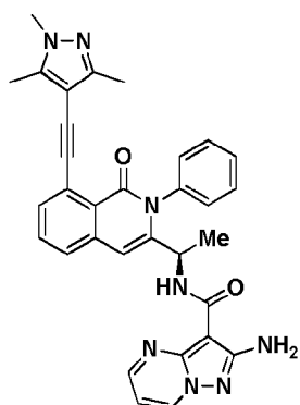
Compound 37r,
