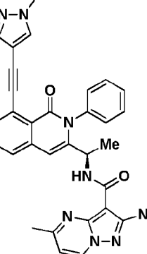
Compound 106r,
