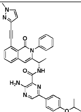
Compound 1062,
