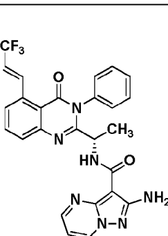
Compound 3001BB,
