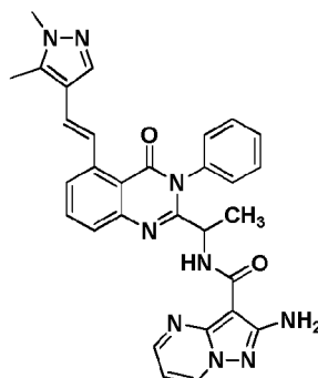
Compound 3007',
