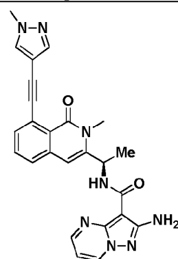
Compound 2055r,
