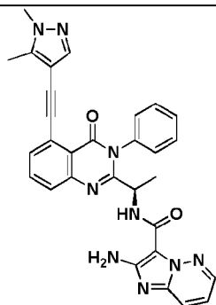
Compound 3070r,
