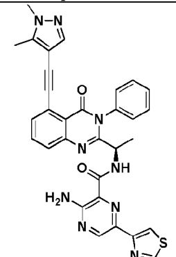
Compound 3058r,
