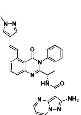
Compound 2052,
