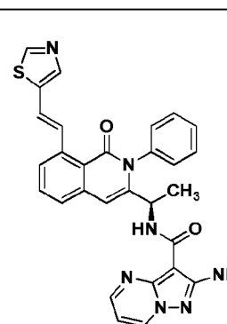
Compound 1002r,
