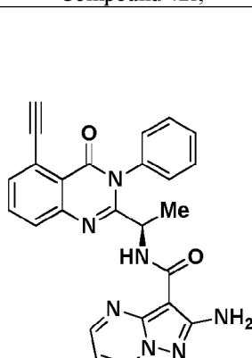
Compound 46r,
