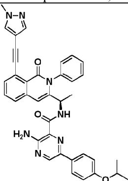
Compound 1061r,
