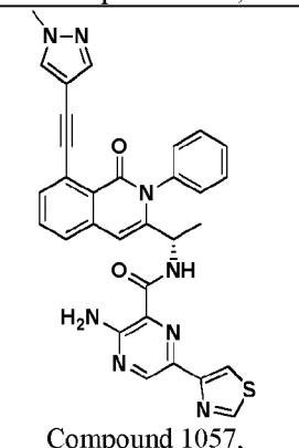
Compound 1057,
