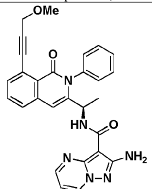
Compound 12r,
