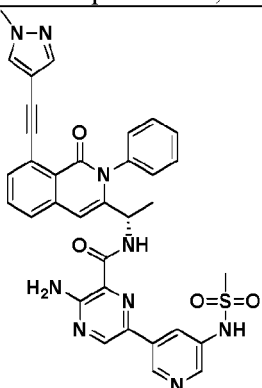
Compound 1065,
