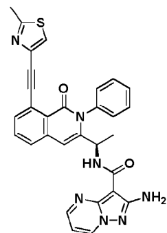
Compound 2063r,
