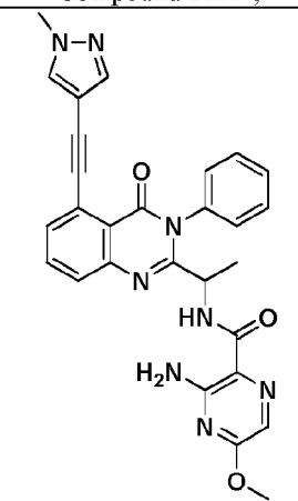
Compound 2071',
