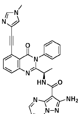
Compound 2081r,
