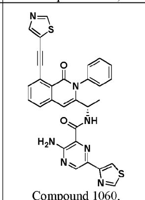
Compound 1060,
