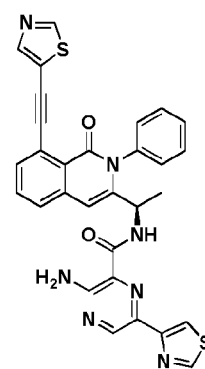
Compound 1060r,
