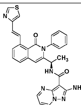
Compound 1004r,
