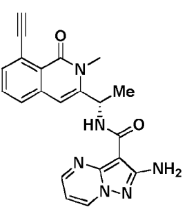
Compound 2048,
