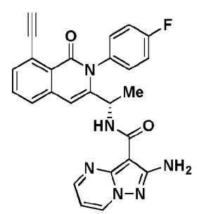
Compound 2050,
