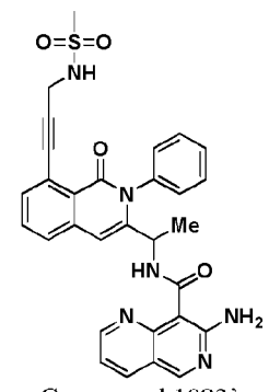
Compound 1083 ' ,
