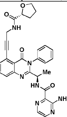
Compound 3077r,
