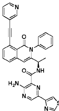
Compound 1059r,
