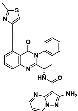
Compound 2040,
