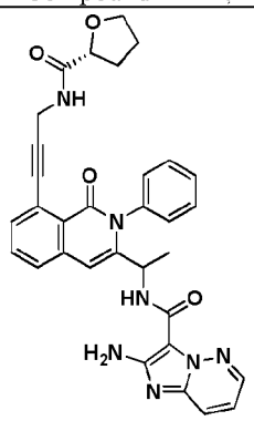
Compound 1085 ' ,
