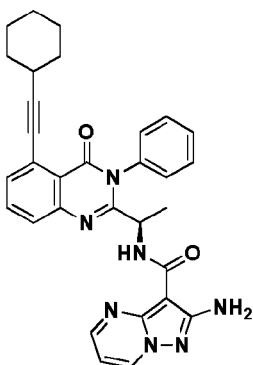
Compound 2065r,
