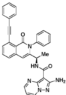
Compound 5r,
