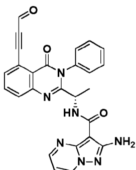
Compound 2036,
