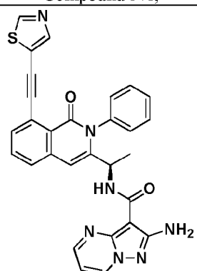
Compound 41r,
