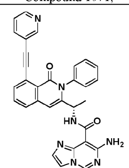
Compound 1075,
