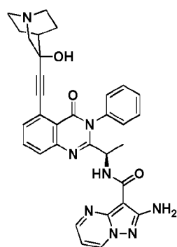
Compound 2062r,
