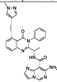
Compound 3073,
