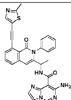
Compound 1076 ' ,
