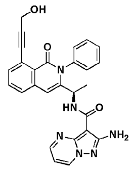
Compound 13r,
