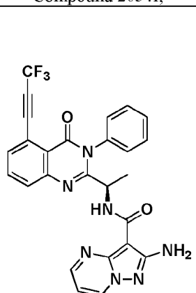
Compound 2058r,
