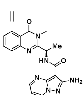
Compound 48r,
