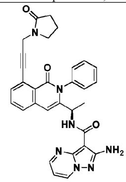
Compound 14r,
