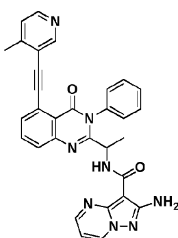
Compound 2061',
