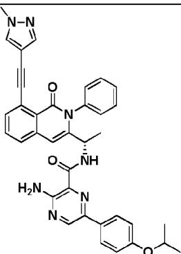
Compound 1061,
