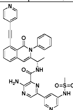
Compound 1067,
