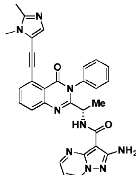
Compound 2038,
