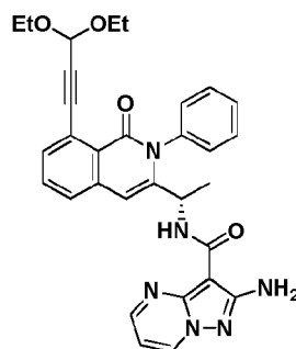
Compound 34,
