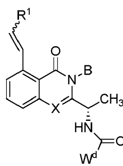
Formula (A),
