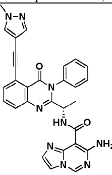
Compound 3073r,
