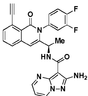
Compound 2045r,
