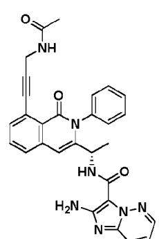
Compound 1086,
