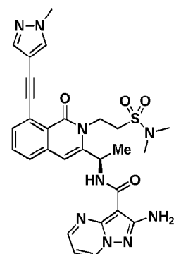
Compound 104r,
