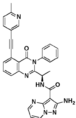
Compound 2077r,
