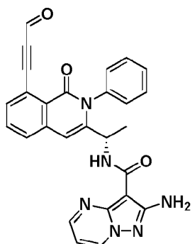
Compound 36,
