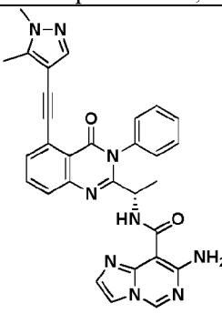
Compound 3074r,
