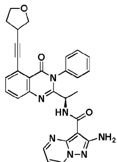
Compound 2084r,
