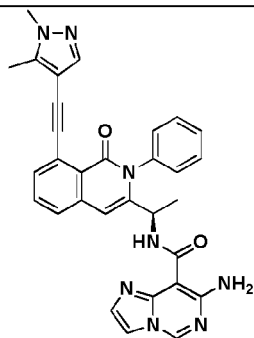
Compound 1074r,
