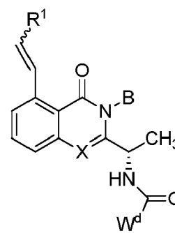
Formula (A),
