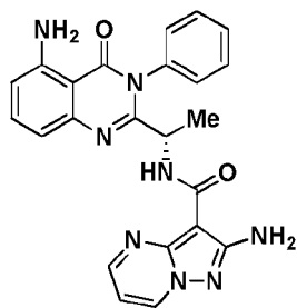
Compound 2109,
