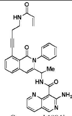
Compound 1084 ' ,
