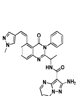
Compound 2053',
