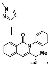
Compound 27,
