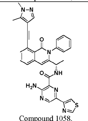
Compound 1058,
