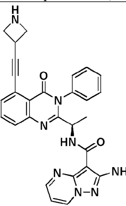
Compound 2074r,
