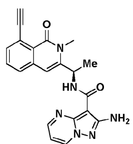
Compound 2048r,
