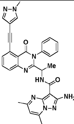
Compound 2108',
