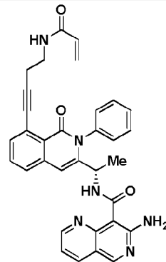
Compound 1084,
