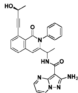
Compound 16',
