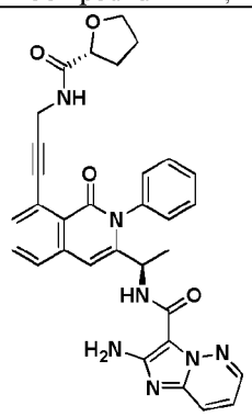
Compound 1085r,
