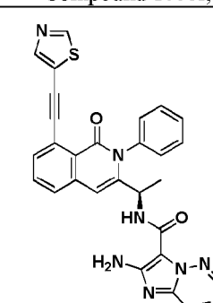
Compound 1072r,
