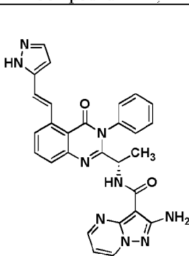
Compound 3006,
