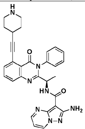
Compound 2072r,
