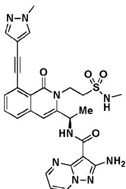
Compound 100r,
