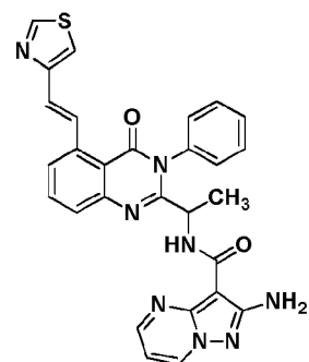
Compound 3004',
