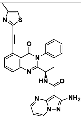
Compound 2060r,
