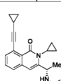
Compound 20,
