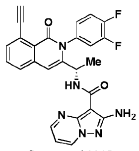
Compound 2045,
