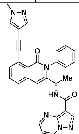
Compound 39,
