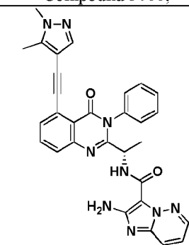
Compound 3070,
