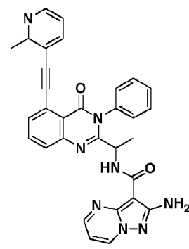
Compound 2067',
