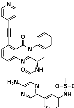
Compound 3067r,
