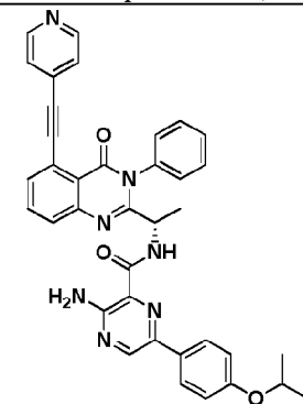
Compound 3063,
