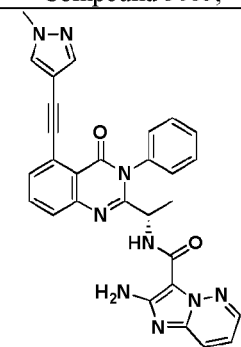
Compound 3069,
