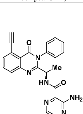
Compound 47r,
