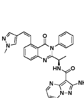
Compound 2053r,
