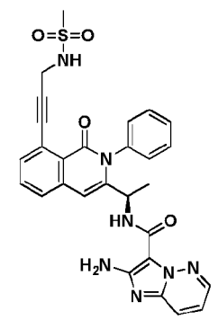
Compound 1087r,
