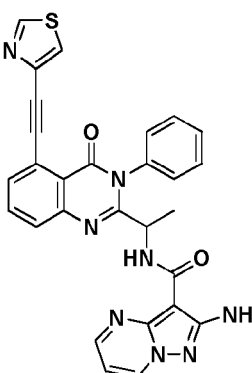
Compound 2054',
