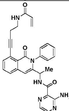
Compound 1080 ' ,
