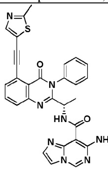
Compound 3076r,
