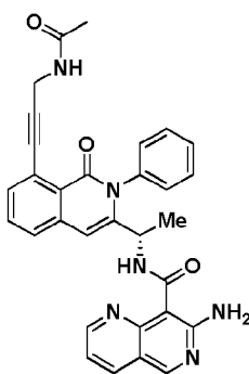
Compound 1082,
