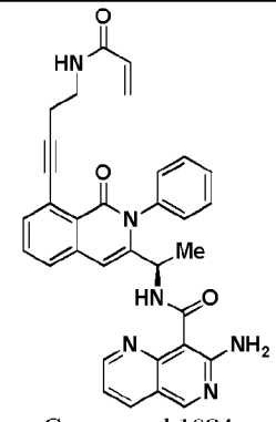
Compound 1084r,
