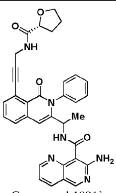
Compound 1081 ' ,
