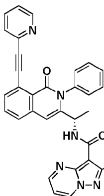
Compound 32,
