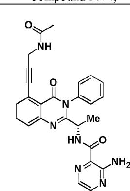
Compound 3078,
