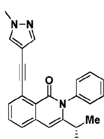
Compound 26,
