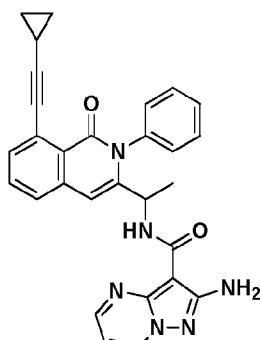
Compound 9',
