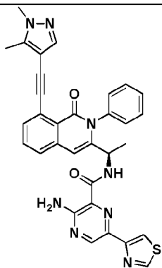
Compound 1058r,
