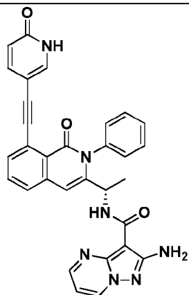
Compound 33,
