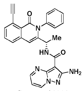
Compound 2046,
