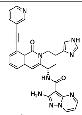
Compound 1047,
