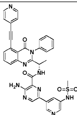
Compound 3067,
