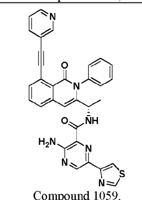
Compound 1059,
