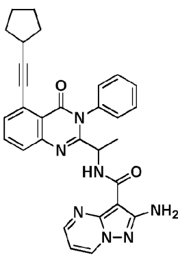
Compound 2064',
