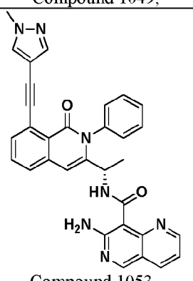
Compound 1053,
