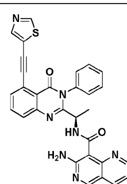
Compound 3056r,
