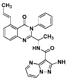
Compound 2070',
