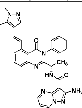
Compound 3007,
