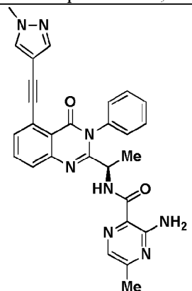
Compound 2068r,
