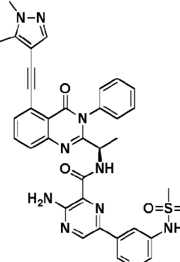
Compound 3066r,
