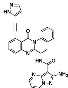
Compound 2043',
