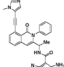
Compound 7',
