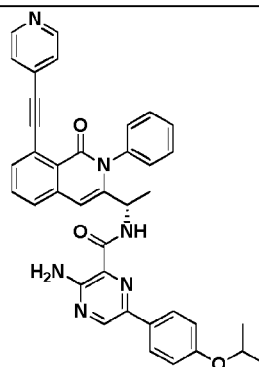
Compound 1063,
