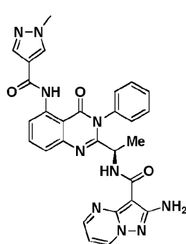
Compound 2090r,
