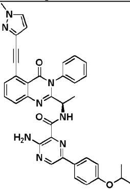
Compound 3062r,
