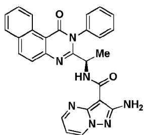
Compound 2089r,
