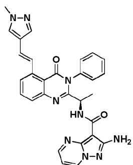
Compound 2052r,
