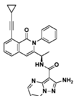
Compound 9r,
