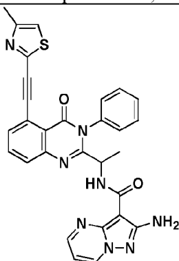
Compound 2060',
