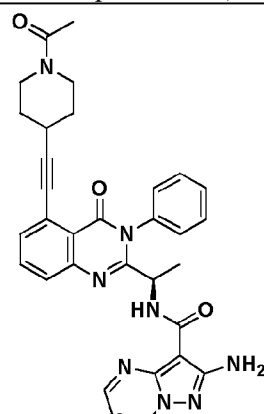
Compound 2082r,
