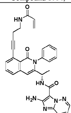
Compound 1088,
