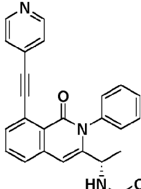
Compound 22,
