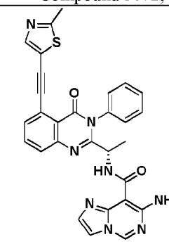
Compound 3076,
