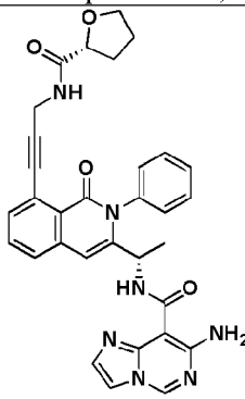
Compound 1089,
