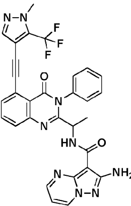
Compound 2069',
