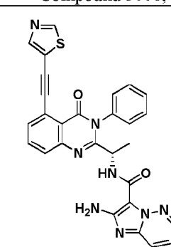
Compound 3072,
