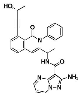
Compound 15',
