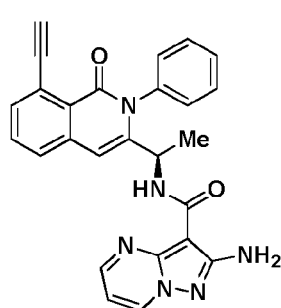
Compound 2046r,
