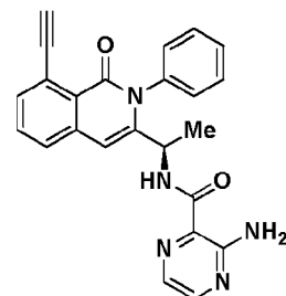
Compound 2047r,
