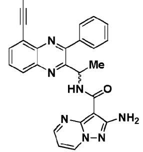
Compound 2051,
