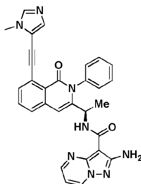
Compound 7r,
