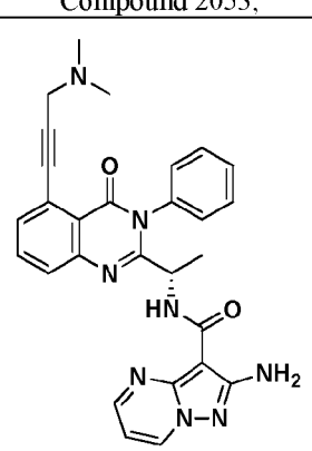
Compound 2057,
