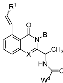
Formula (A'),
