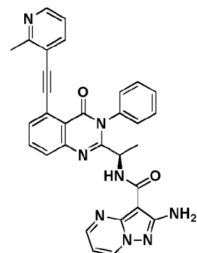
Compound 2067r,
