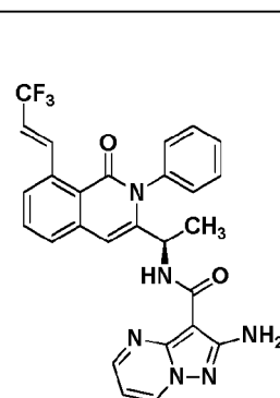
Compound 1001r,
