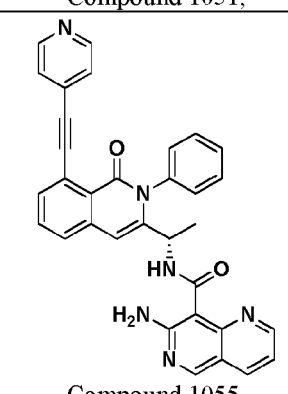
Compound 1055,
