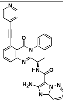
Compound 3071r,
