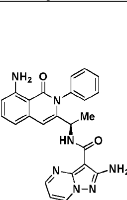
Compound 109r,
