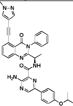
Compound 3061r,
