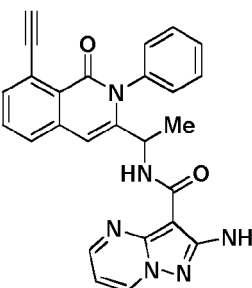
Compound 2046',
