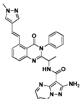
Compound 2052',
