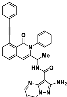
Compound 5',
