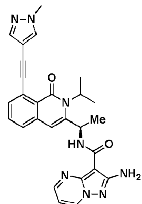
Compound 103r,
