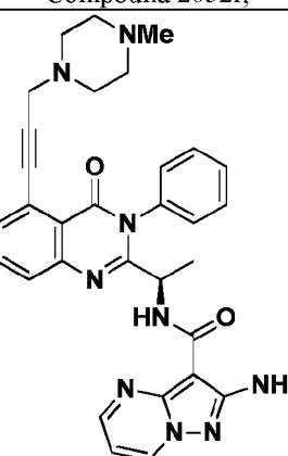
Compound 2056r,
