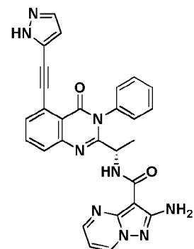
Compound 2043,
