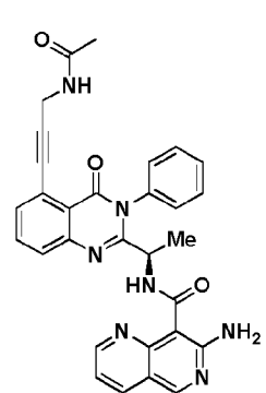
Compound 3082r,
