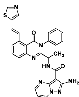
Compound 3002',
