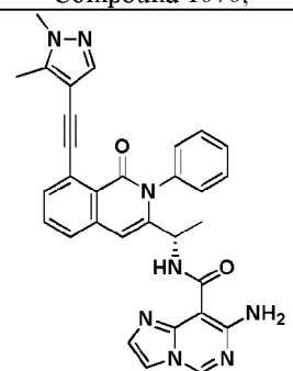
Compound 1074,
