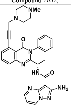
Compound 2056,
