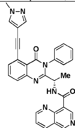
Compound 2042,
