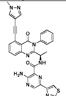
Compound 3057r,
