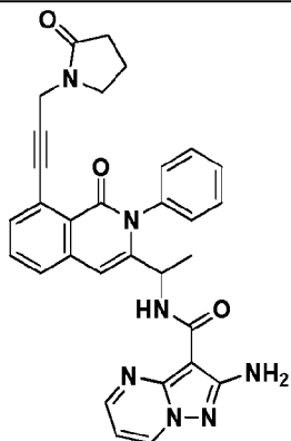
Compound 14',
