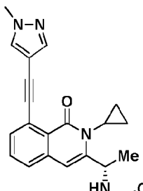
Compound 21,
