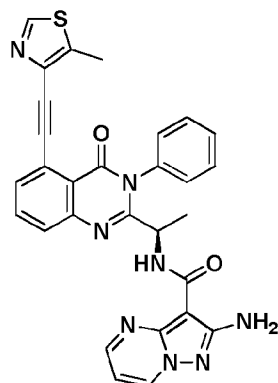
Compound 2078r,
