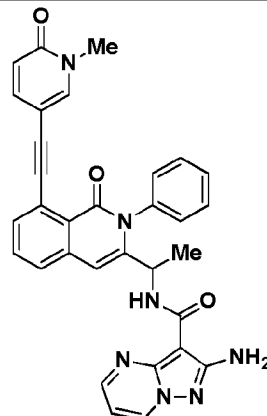
Compound 20',
