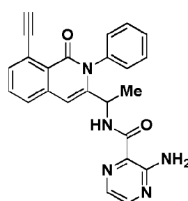
Compound 2047',
