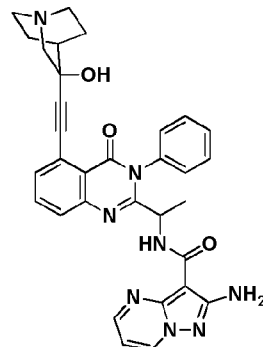
Compound 2062',
