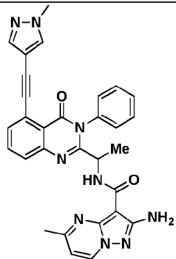
Compound 2106',
