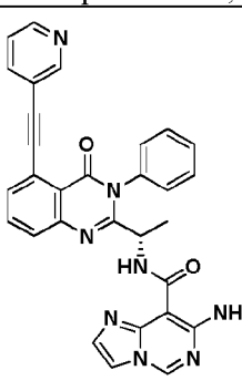
Compound 3075r,
