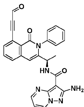
Compound 36r,
