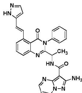
Compound 3006',
