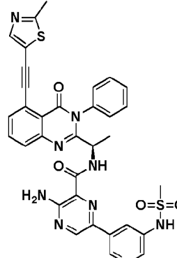
Compound 3068r,
