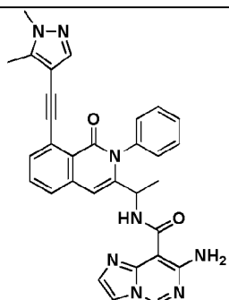
Compound 1074 ' ,
