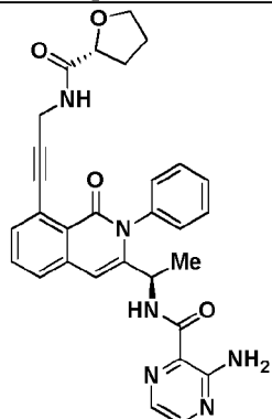
Compound 1077r,
