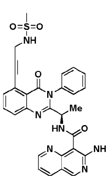
Compound 3083r,
