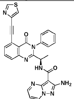
Compound 2054r,
