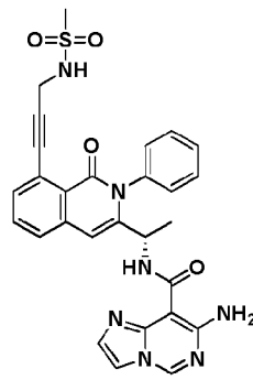
Compound 1091,
