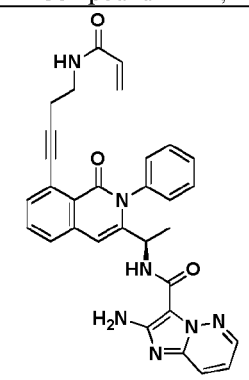
Compound 1088r,
