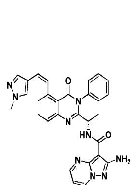
Compound 2053,
