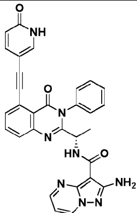
Compound 2033,
