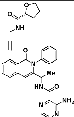
Compound 1077 ' ,
