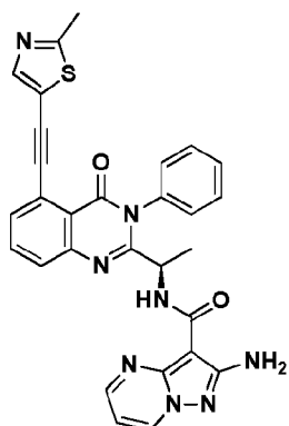
Compound 2076r,
