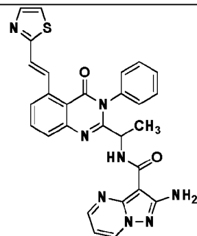
Compound 3003',
