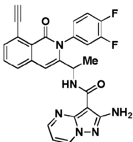
Compound 2045',
