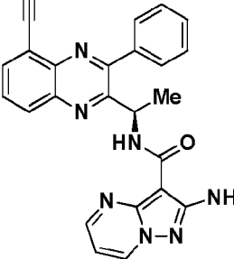
Compound 2051r,
