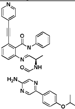
Compound 3063r,
