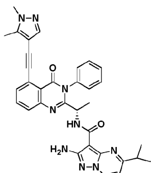
Compound 3050,
