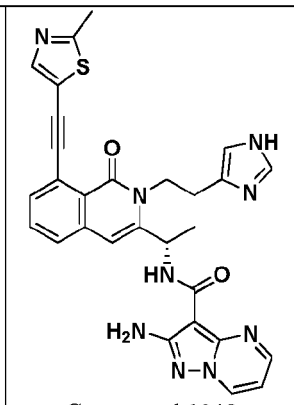
Compound 1048,
