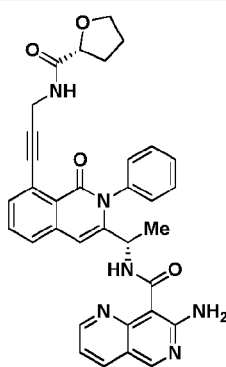
Compound 1081,
