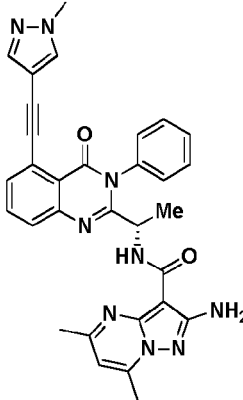
Compound 2108,
