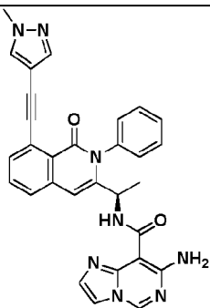
Compound 1073r,
