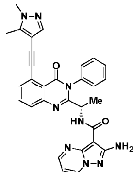
Compound 2035,
