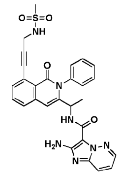
Compound 1087 ' ,
