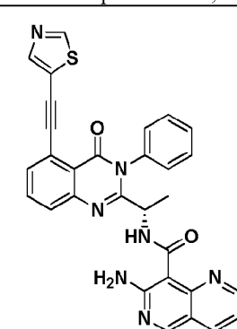
Compound 3056,
