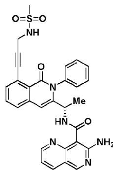
Compound 1083,
