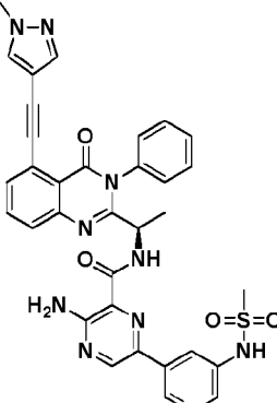
Compound 3065r,
