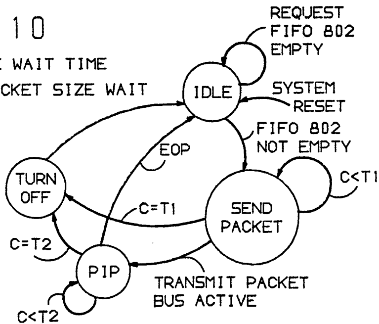
OUTPUT CONTROLLER 803
