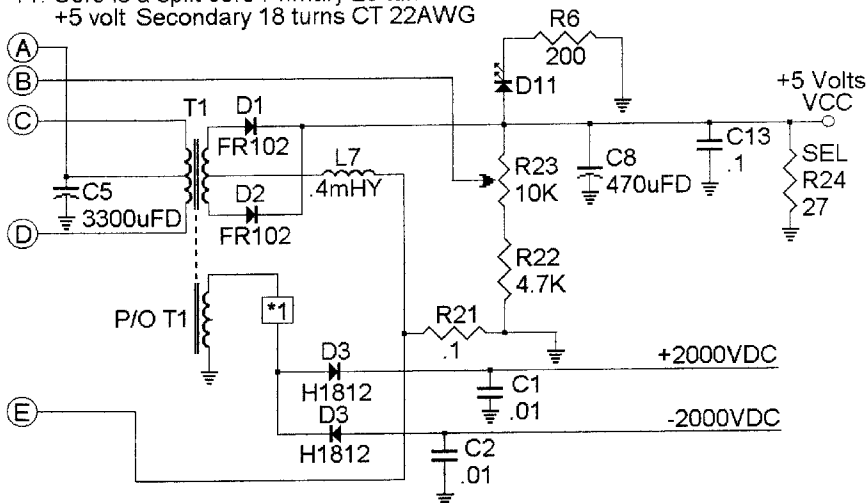
T1: Core is a split core Primary 20 turns CT 22AWG +5 volt Secondary 18 turns CT 22AWG
