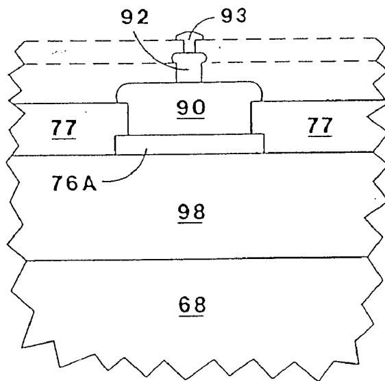
FIG. 11 PRIOR ART
