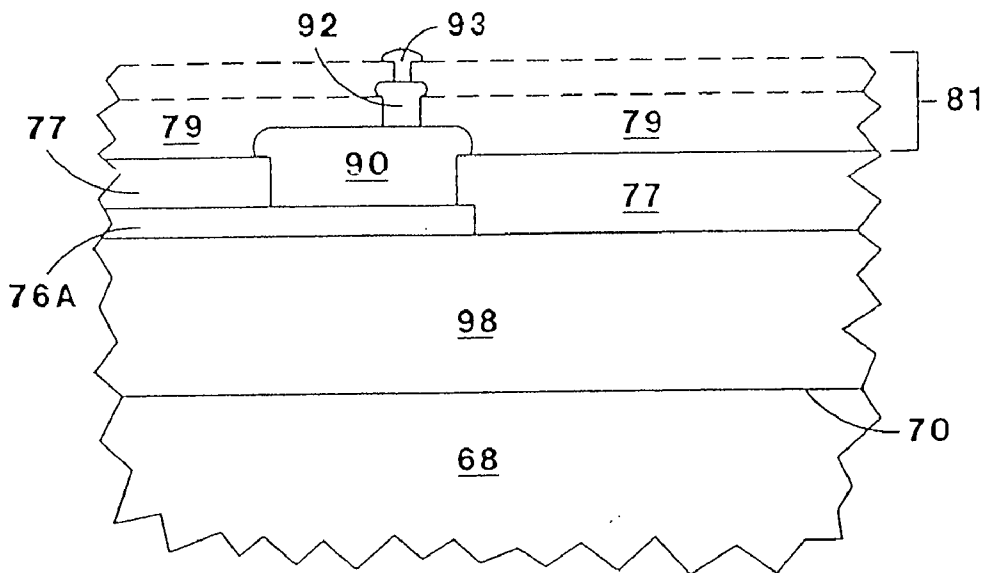
FIG. 10 PRIOR ART
