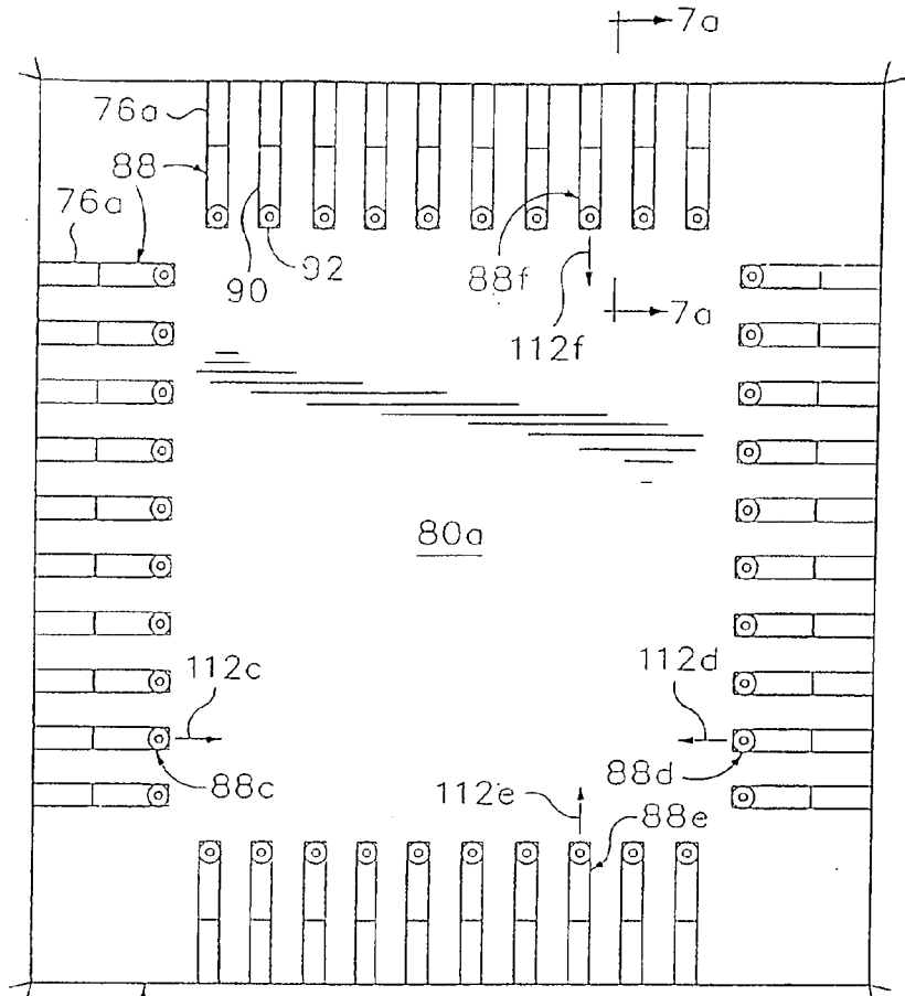
FIG. 6 PRIOR ART
