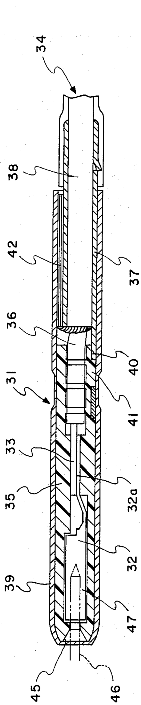
FIG. 1 PRIOR ART
