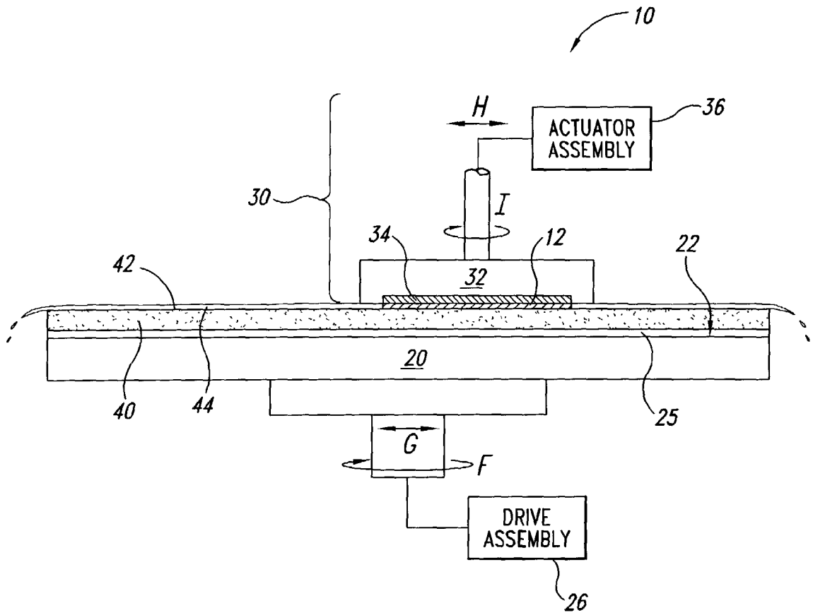
Fig. 1 (Prior Art)
