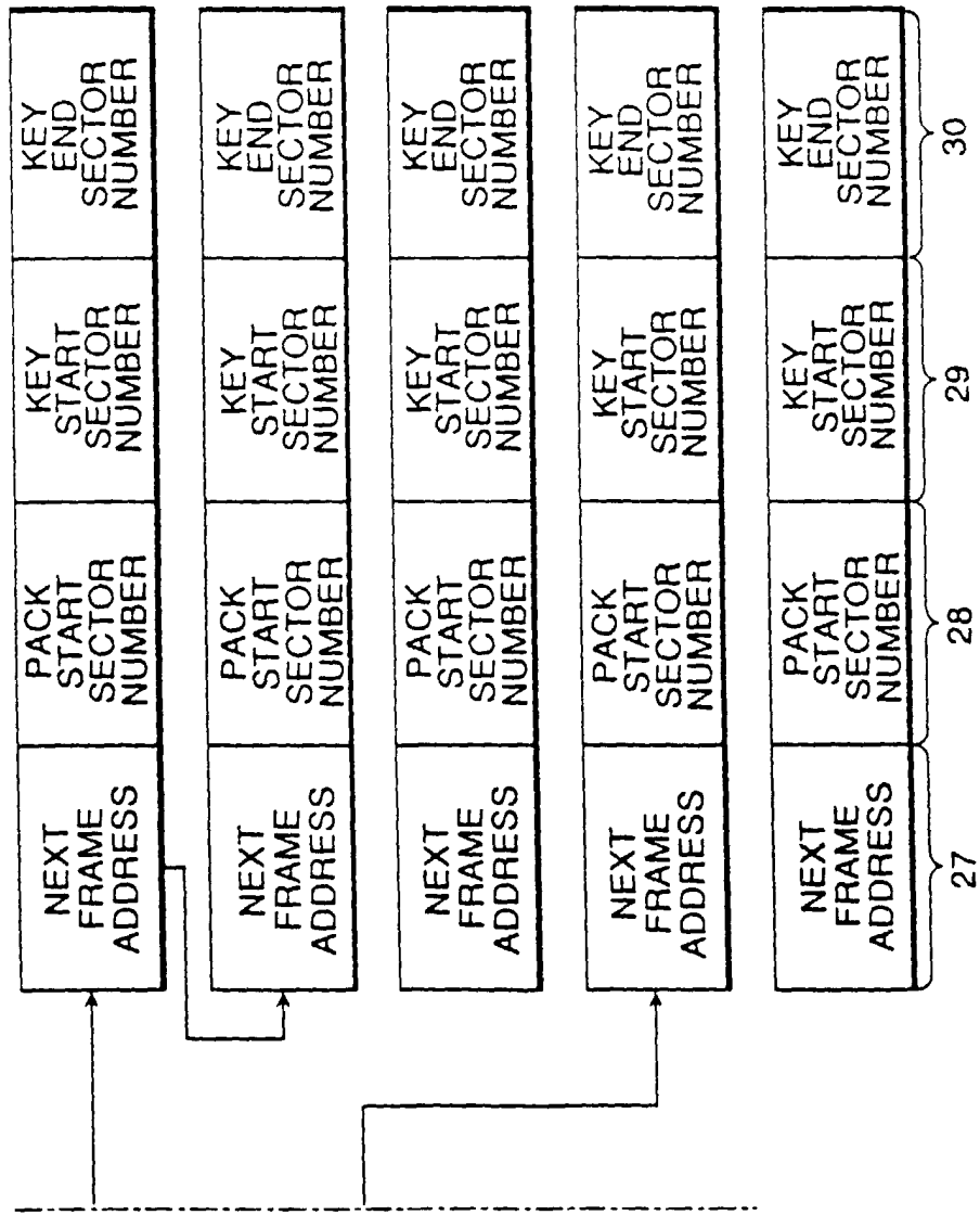
MEMORY 14 (KEY FRAME TABLE)
