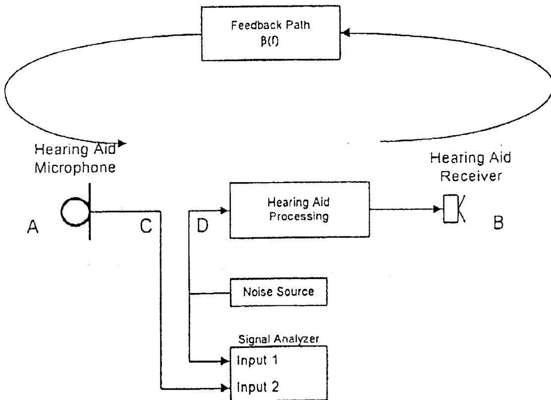
FIG. 3 (PRIOR ART)
