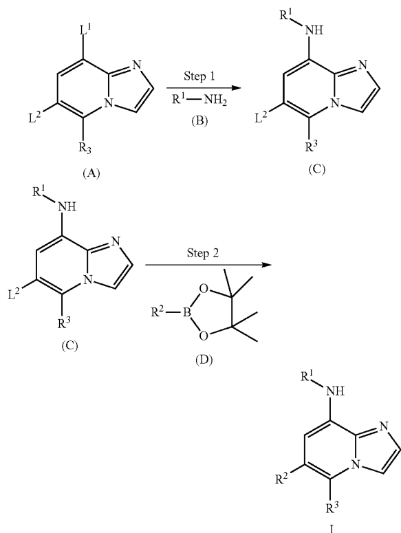
REACTION SCHEME 1
