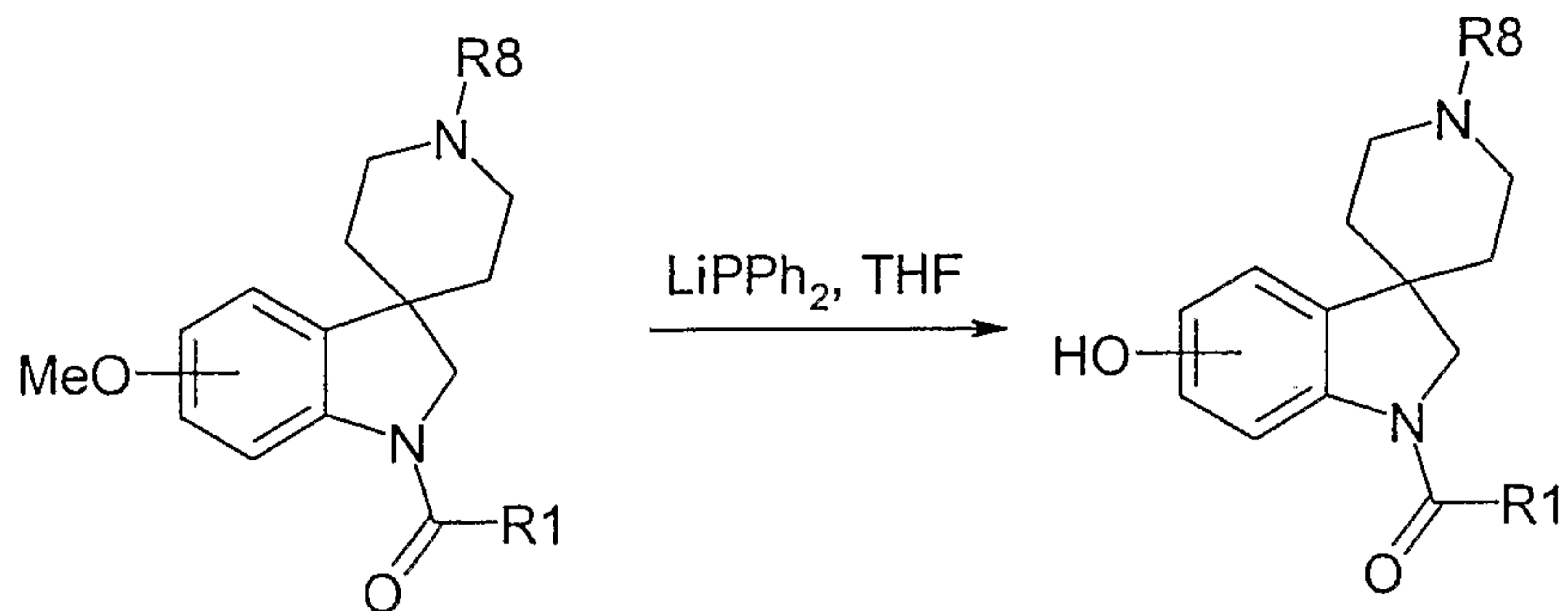
SCHEME IV
