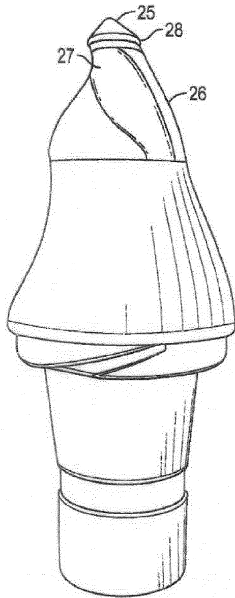
FIG. 5 (Prior Art)
