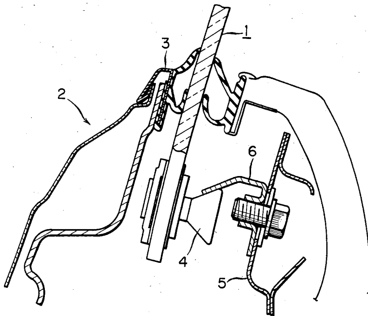
Fig. 6 PRIOR ART
