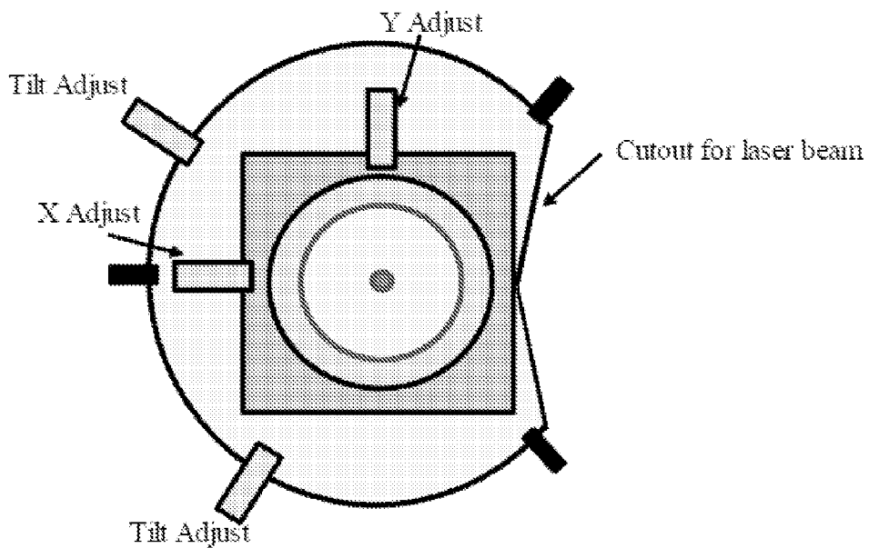
Top View of Precision Adjustment System
