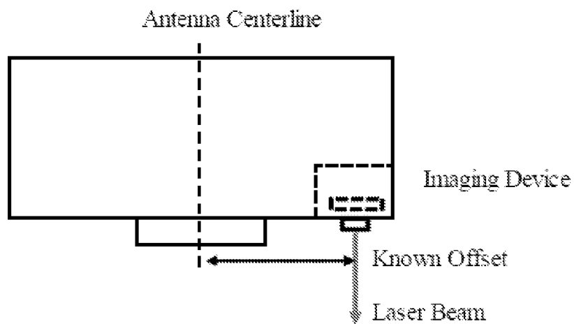
Side View of Integrated Receiver & Imaging Device
