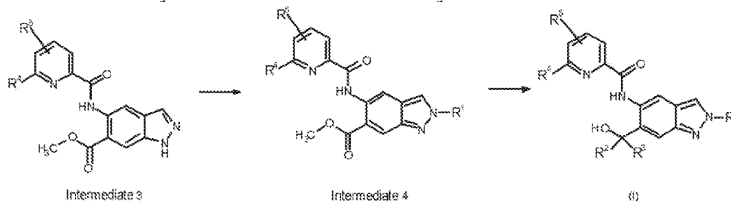
Synthesis Scheme 3
