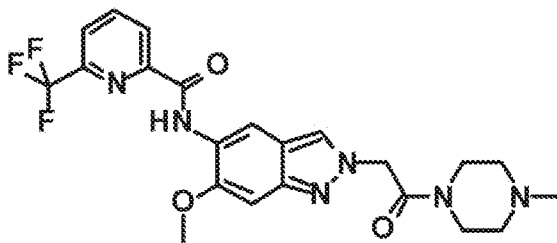
Example 64
