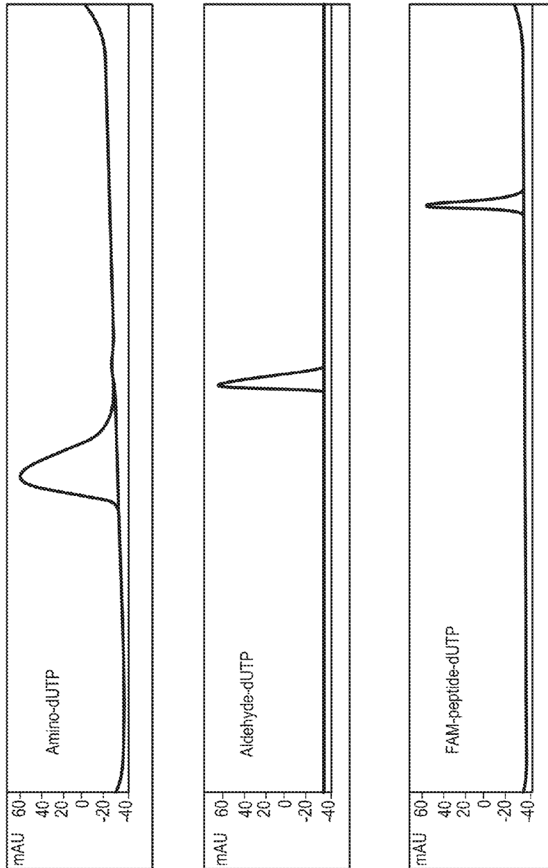
HPLC Analysis of Modified dUTPs
