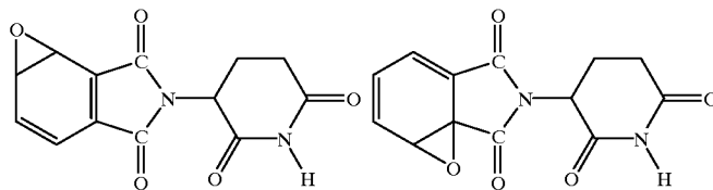
Epoxides of thalidomide
